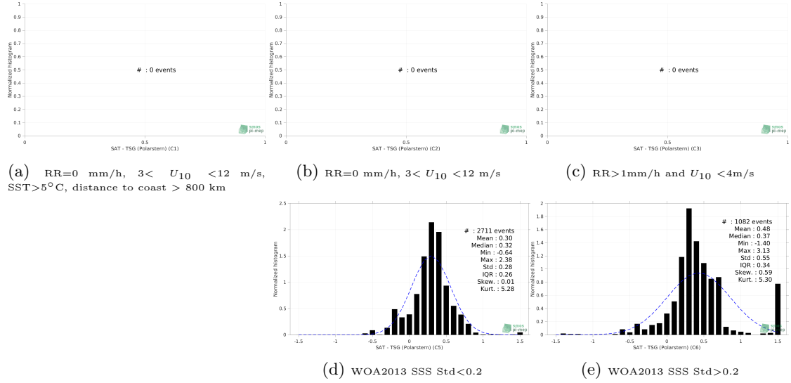
Figure 13: Normalized histogram of \Delta SSS (Aquarius SSS L3 CAP v5 - Monthly (JPL) - TSG (Polarstern)) for 5 different subdatasets corresponding to: RR=0 mm/h, 3 < U_{10} < 12 m/s, SST >5^{\circ} C, distance to coast > 800 km (a), RR=0 mm/h, 3 < U_{10} < 12 m/s (b), RR >1 mm/h and U_{10} < 4 m/s (c), WOA2013 SSS Std <0.2 (d), WOA2013 SSS Std >0.2 (e).
