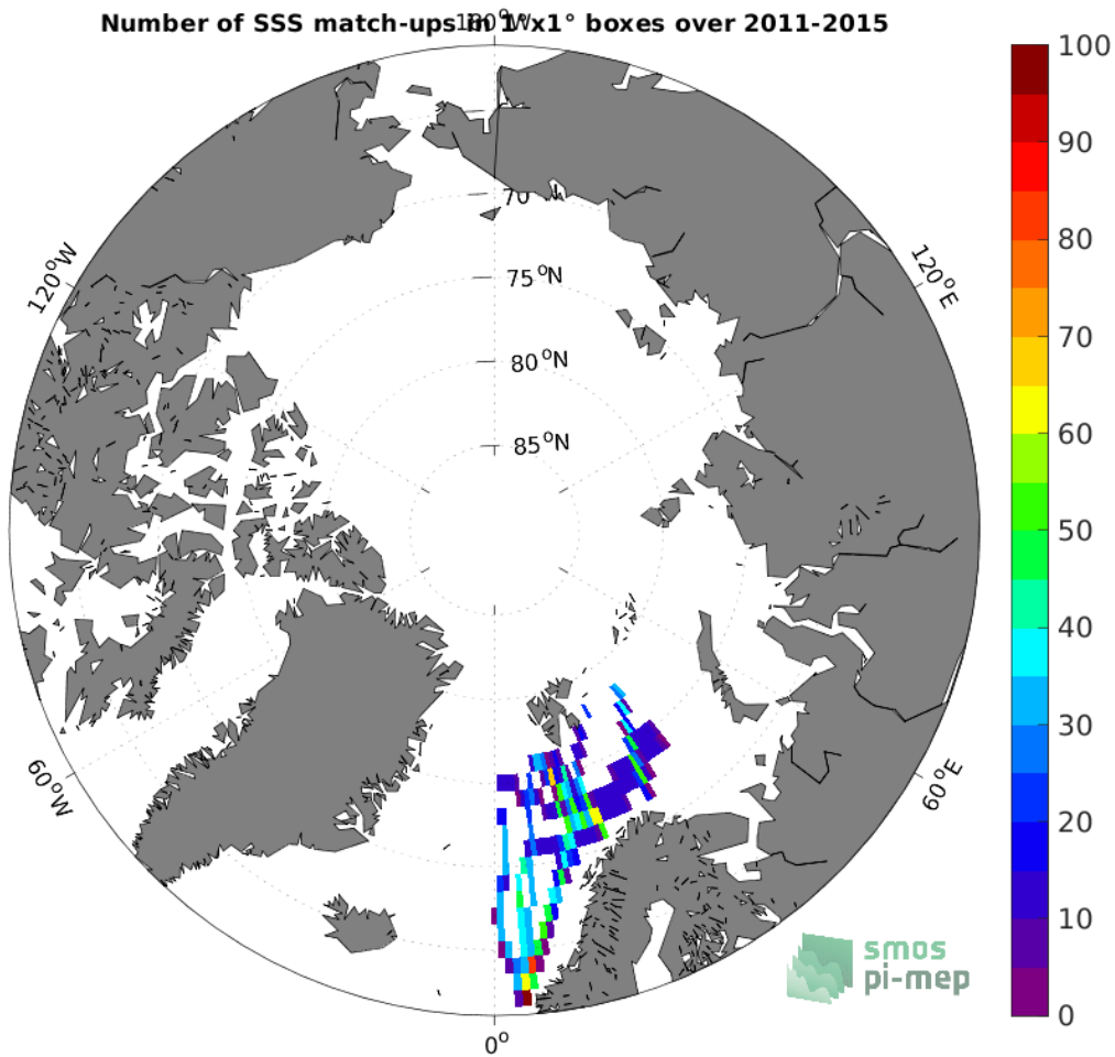
Figure 4: Number of SSS match-ups between TSG (Polarstern) SSS and the Aquarius SSS L3 CAP v5 - Monthly (JPL) SSS product for the Arctic Ocean Pi-MEP region over 1^{\circ} \times 1^{\circ} boxes and for the full satellite product period.
