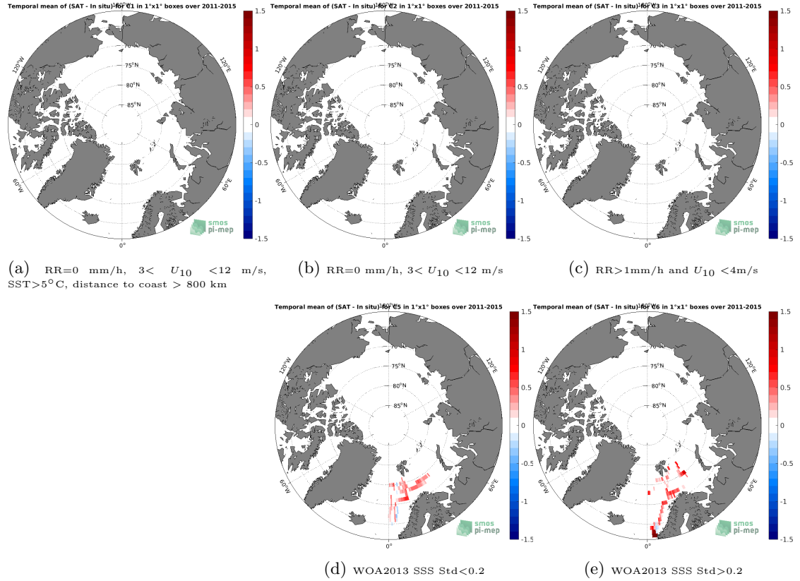
Figure 12: Temporal mean gridded over spatial boxes of size 1^{\circ}\times 1^{\circ} of \Delta\text{SSS} (Aquarius SSS L3 CAP v5 - Monthly (JPL) - TSG (Polarstern)) for 5 different subdatasets corresponding to: RR=0 mm/h, 3 < U_{10} < 12 m/s, SST >5^{\circ}\text{C} , distance to coast > 800 km (a), RR=0 mm/h, 3 < U_{10} < 12 m/s (b), RR >1 mm/h and U_{10} < 4 m/s (c), WOA2013 SSS Std <0.2 (d), WOA2013 SSS Std >0.2 (e).
