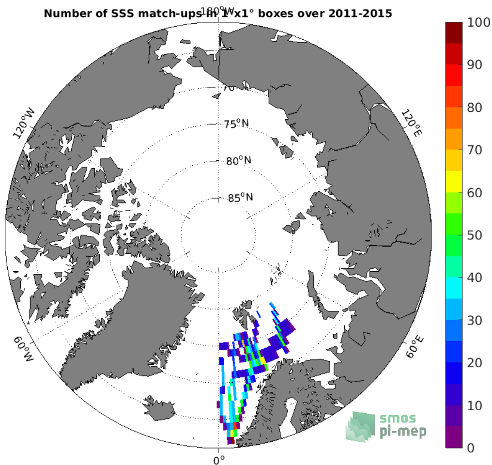
Figure 4: Number of SSS match-ups between TSG (Polarstern) SSS and the Aquarius SSS L3 CAP v5 - Monthly (JPL) SSS product for the Arctic Ocean Pi-MEP region over 1^\circ \times 1^\circ boxes and for the full satellite product period.
