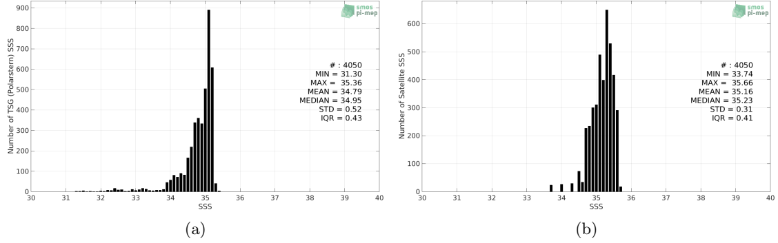
Figure 2: Histograms of SSS from TSG (Polarstern) (a) and Aquarius SSS L3 CAP v5 - Monthly (JPL) (b) considering all match-up pairs per bins of 0.1 over the Arctic Ocean Pi-MEP region and for the full satellite product period.
