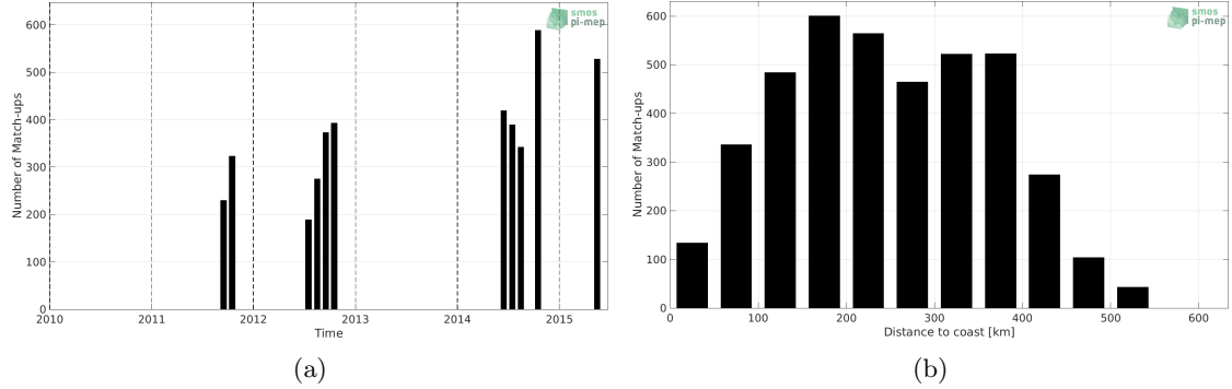
Figure 1: Number of match-ups between TSG (Polarstern) and Aquarius SSS L3 CAP v5 - Monthly (JPL) SSS as a function of time (a) and as function of the distance to coast (b) over the Arctic Ocean Pi-MEP region and for the full satellite product period.
