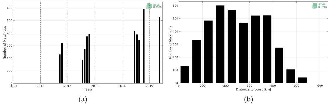
Figure 1: Number of match-ups between TSG-POLARSTERN and Aquarius-L3-JPL-V5-MONTHLY SSS as a function of time (a) and as function of the distance to coast (b) over the Arctic Ocean Pi-MEP region and for the full satellite product period.
