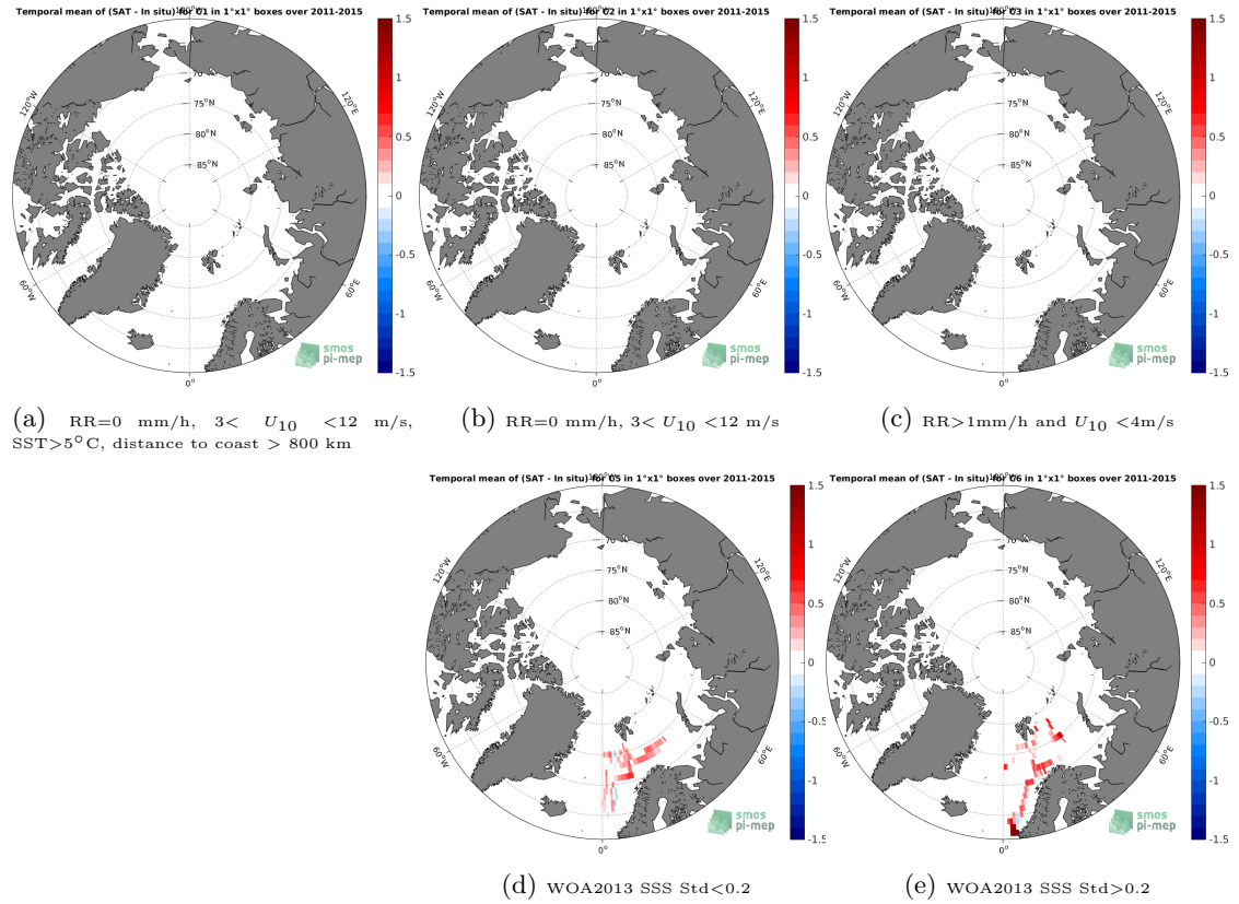
Figure 12: Temporal mean gridded over spatial boxes of size 1^{\circ}\times 1^{\circ} of \Delta\text{SSS} (Aquarius-L3-JPL-V5-MONTHLY - TSG-POLARSTERN) for 5 different subdatasets corresponding to: \text{RR}=0 mm/h, 3 < U_{10} < 12 m/s, \text{SST} > 5^{\circ}\text{C} , distance to coast > 800 km (a), \text{RR}=0 mm/h, 3 < U_{10} < 12 m/s (b), \text{RR} > 1 mm/h and U_{10} < 4 m/s (c), WOA2013 SSS Std < 0.2 (d), WOA2013 SSS Std > 0.2 (e).
