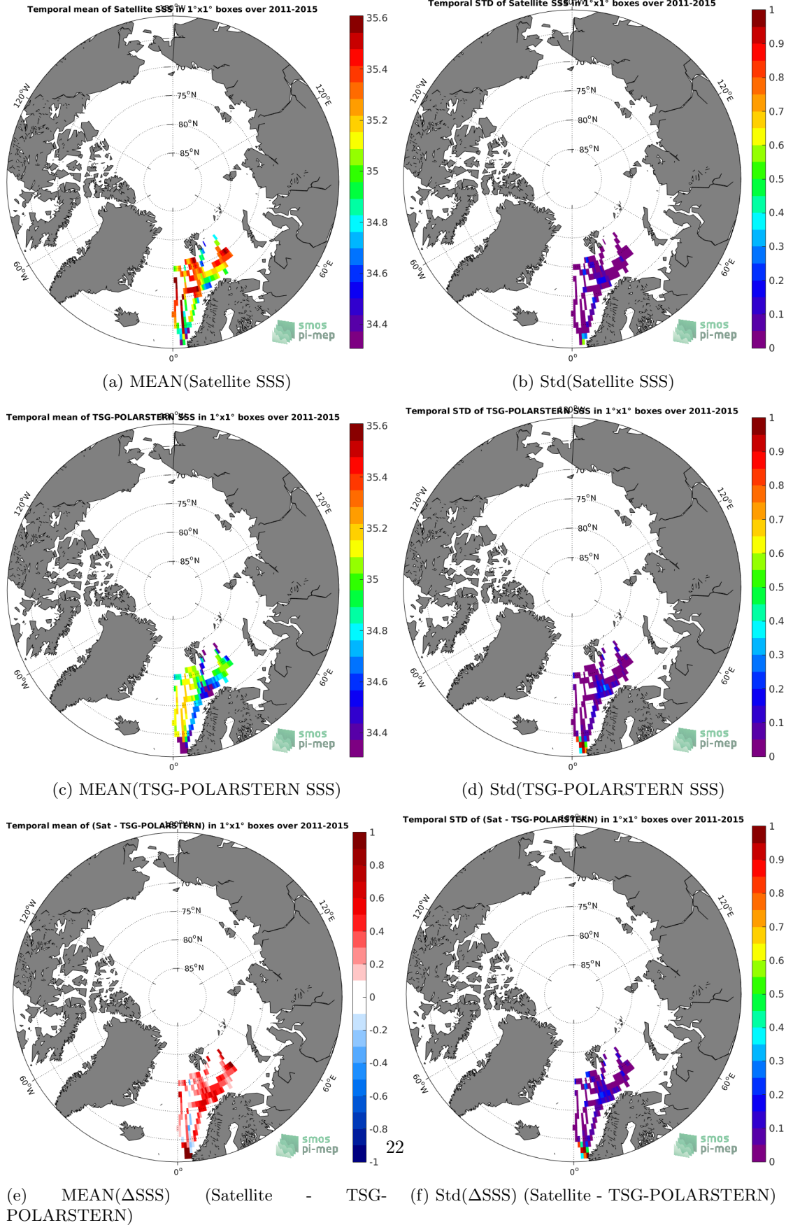
Figure 6: Temporal mean (left) and Std (right) of SSS from Aquarius-L3-JPL-V5-MONTHLY (top), TSG-POLARSTERN (middle), and of \Delta SSS (Satellite - TSG-POLARSTERN). Only match-up pairs are used to generate these maps.
