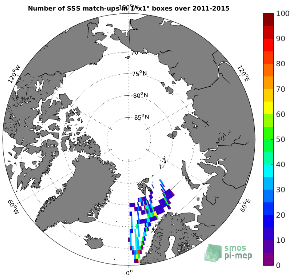
Figure 4: Number of SSS match-ups between TSG-POLARSTERN SSS and the Aquarius-L3-JPL-V5-MONTHLY SSS product for the Arctic Ocean Pi-MEP region over 1^\circ \times 1^\circ boxes and for the full satellite product period.
