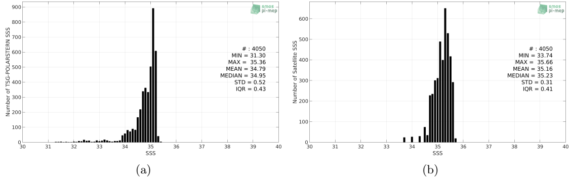
Figure 2: Histograms of SSS from TSG-POLARSTERN (a) and Aquarius-L3-JPL-V5-MONTHLY (b) considering all match-up pairs per bins of 0.1 over the Arctic Ocean Pi-MEP region and for the full satellite product period.
