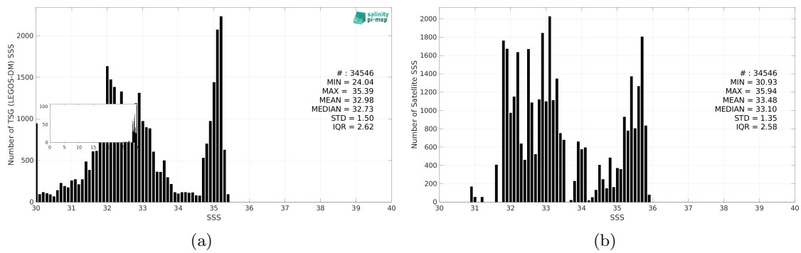
Figure 3: Histograms of SSS from TSG (LEGOS-DM) (a) and Aquarius SSS L3 CAP v5 - Monthly (JPL) (b) considering all match-up pairs per bins of 0.1 over the Arctic Ocean Pi-MEP region and for the full satellite product period.
