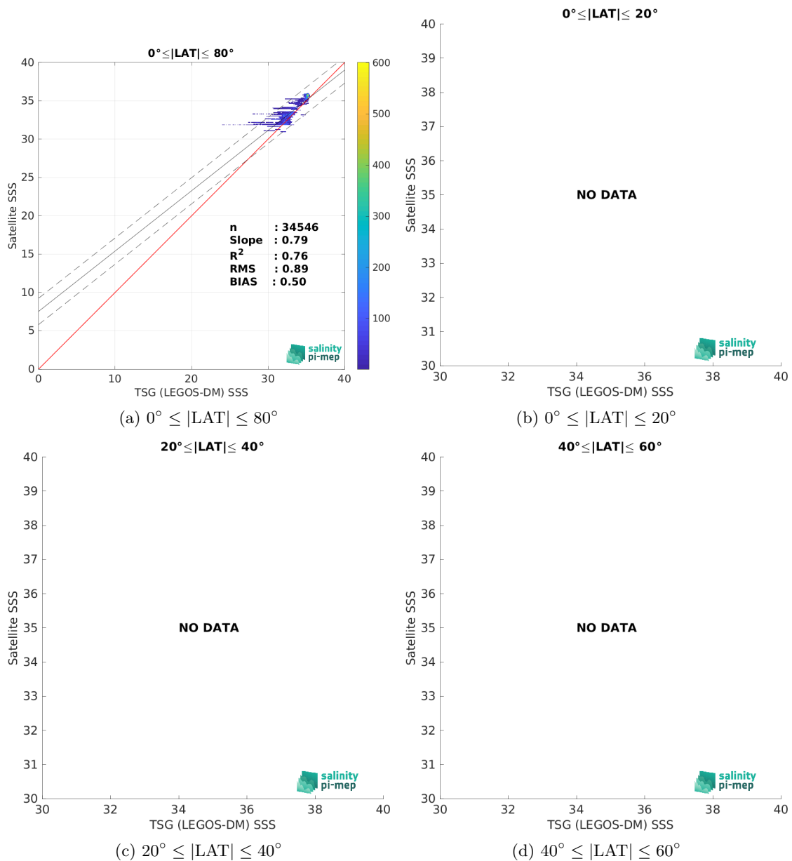
Figure 10: Contour maps of the concentration of Aquarius SSS L3 CAP v5 - Monthly (JPL) SSS (y-axis) versus TSG (LEGOS-DM) SSS (x-axis) at match-up pairs for different latitude bands. For each plot, the red line shows x=y . The black thin and dashed lines indicate a linear fit through the data cloud and the \pm 95\% confidence levels, respectively. The number match-up pairs n , the slope and R^2 coefficient of the linear fit, the root mean square (RMS) and the mean bias between satellite and in situ data are indicated for each latitude band in each plots.
