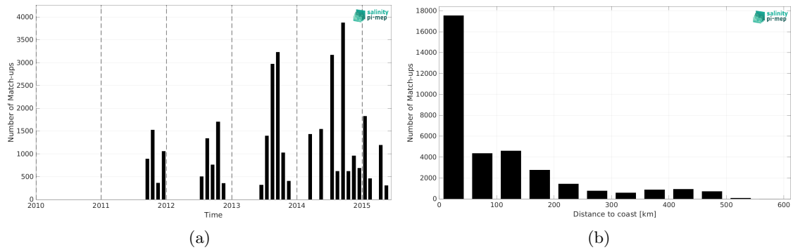
Figure 2: Number of match-ups between TSG (LEGOS-DM) and Aquarius SSS L3 CAP v5 - Monthly (JPL) SSS as a function of time (a) and as function of the distance to coast (b) over the Arctic Ocean Pi-MEP region and for the full satellite product period.
