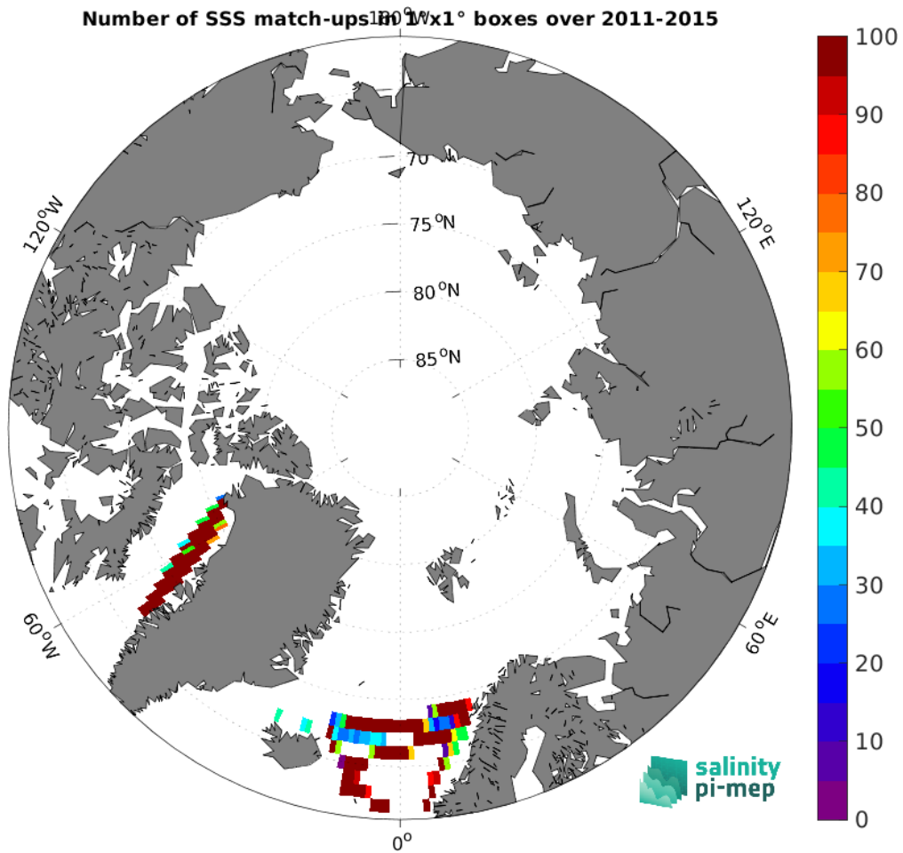
Figure 5: Number of SSS match-ups between TSG (LEGOS-DM) SSS and the Aquarius SSS L3 CAP v5 - Monthly (JPL) SSS product for the Arctic Ocean Pi-MEP region over 1^\circ \times 1^\circ boxes and for the full satellite product period.
