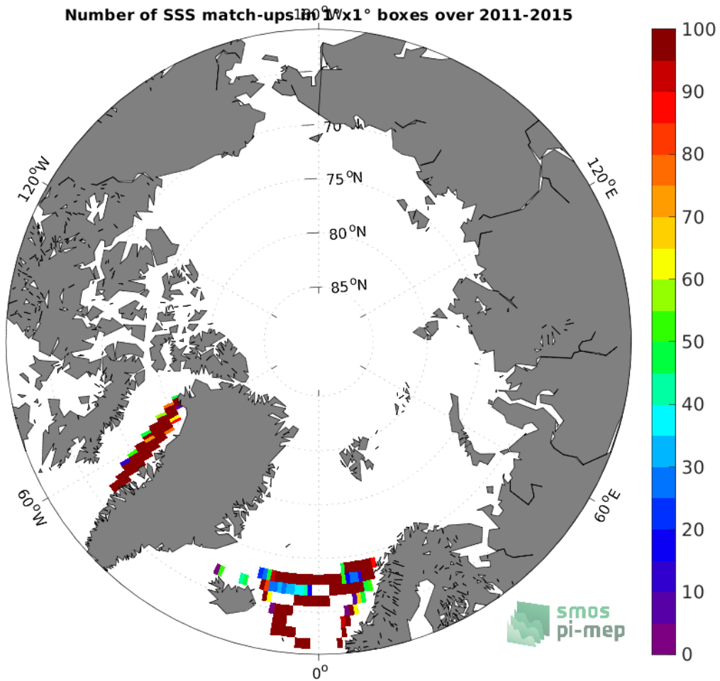
Figure 4: Number of SSS match-ups between TSG (LEGOS-DM) SSS and the Aquarius SSS L3 CAP v5 - Monthly (JPL) SSS product for the Arctic Ocean Pi-MEP region over 1^{\circ} \times 1^{\circ} boxes and for the full satellite product period.
