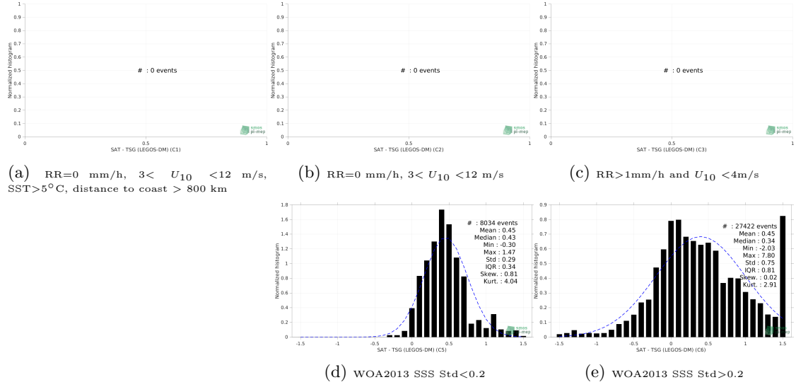
Figure 13: Normalized histogram of \Delta SSS (Aquarius SSS L3 CAP v5 - Monthly (JPL) - TSG (LEGOS-DM)) for 5 different subdatasets corresponding to: RR=0 mm/h, 3 < U_{10} < 12 m/s, SST >5^{\circ} C, distance to coast > 800 km (a), RR=0 mm/h, 3 < U_{10} < 12 m/s (b), RR >1 mm/h and U_{10} < 4 m/s (c), WOA2013 SSS Std <0.2 (d), WOA2013 SSS Std >0.2 (e).
