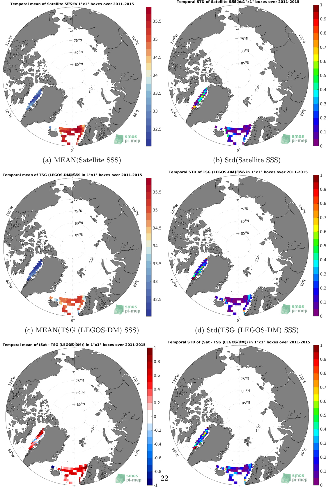
(e) MEAN( \Delta SSS) (Satellite - TSG (LEGOS-DM)) (f) Std( \Delta SSS) (Satellite - TSG (LEGOS-DM)) Figure 6: Temporal mean (left) and Std (right) of SSS from Aquarius SSS L3 CAP v5 - Monthly (JPL) (top), TSG (LEGOS-DM) (middle), and of \Delta SSS (Satellite - TSG (LEGOS-DM)). Only match-up pairs are used to generate these maps.
