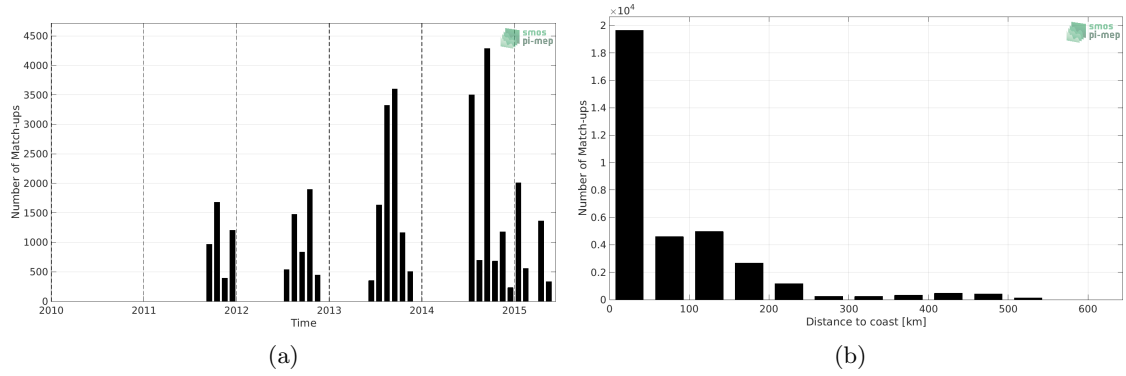
Figure 1: Number of match-ups between TSG (LEGOS-DM) and Aquarius SSS L3 CAP v5 - Monthly (JPL) SSS as a function of time (a) and as function of the distance to coast (b) over the Arctic Ocean Pi-MEP region and for the full satellite product period.
