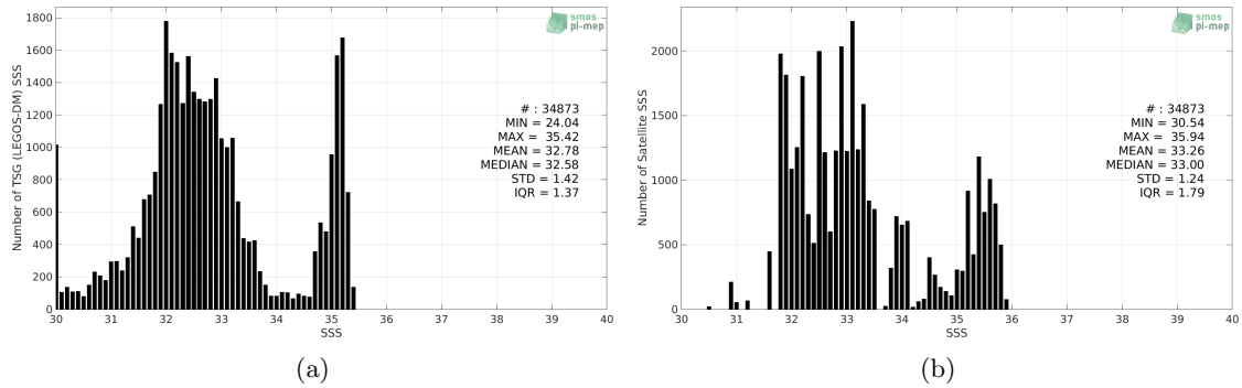
Figure 2: Histograms of SSS from TSG (LEGOS-DM) (a) and Aquarius SSS L3 CAP v5 - Monthly (JPL) (b) considering all match-up pairs per bins of 0.1 over the Arctic Ocean Pi-MEP region and for the full satellite product period.
