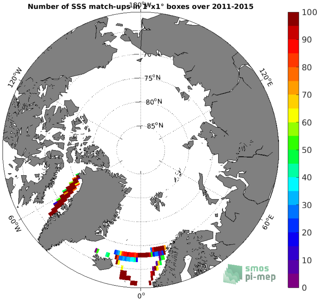
Figure 4: Number of SSS match-ups between TSG (LEGOS-DM) SSS and the Aquarius SSS L3 CAP v5 - Monthly (JPL) SSS product for the Arctic Ocean Pi-MEP region over 1^\circ \times 1^\circ boxes and for the full satellite product period.
