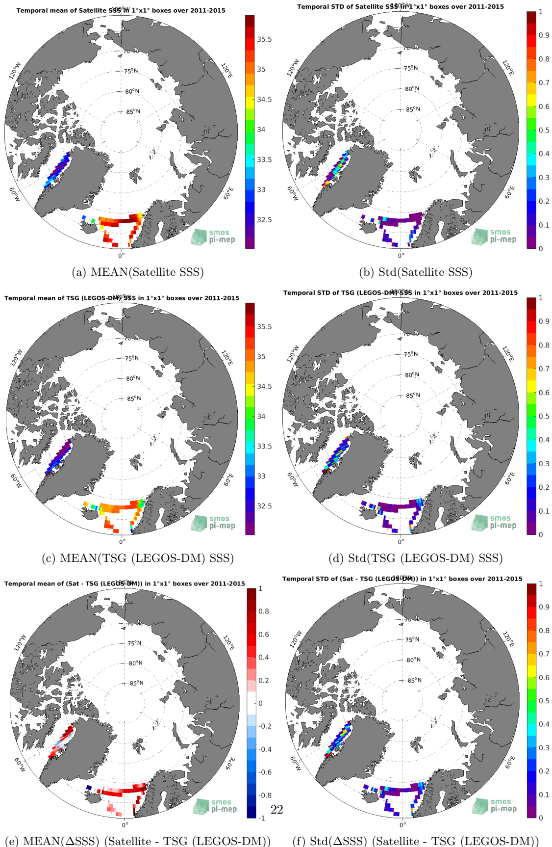
Figure 6: Temporal mean (left) and Std (right) of SSS from Aquarius SSS L3 CAP v5 - Monthly (JPL) (top), TSG (LEGOS-DM) (middle), and of \Delta SSS (Satellite - TSG (LEGOS-DM)). Only match-up pairs are used to generate these maps.
