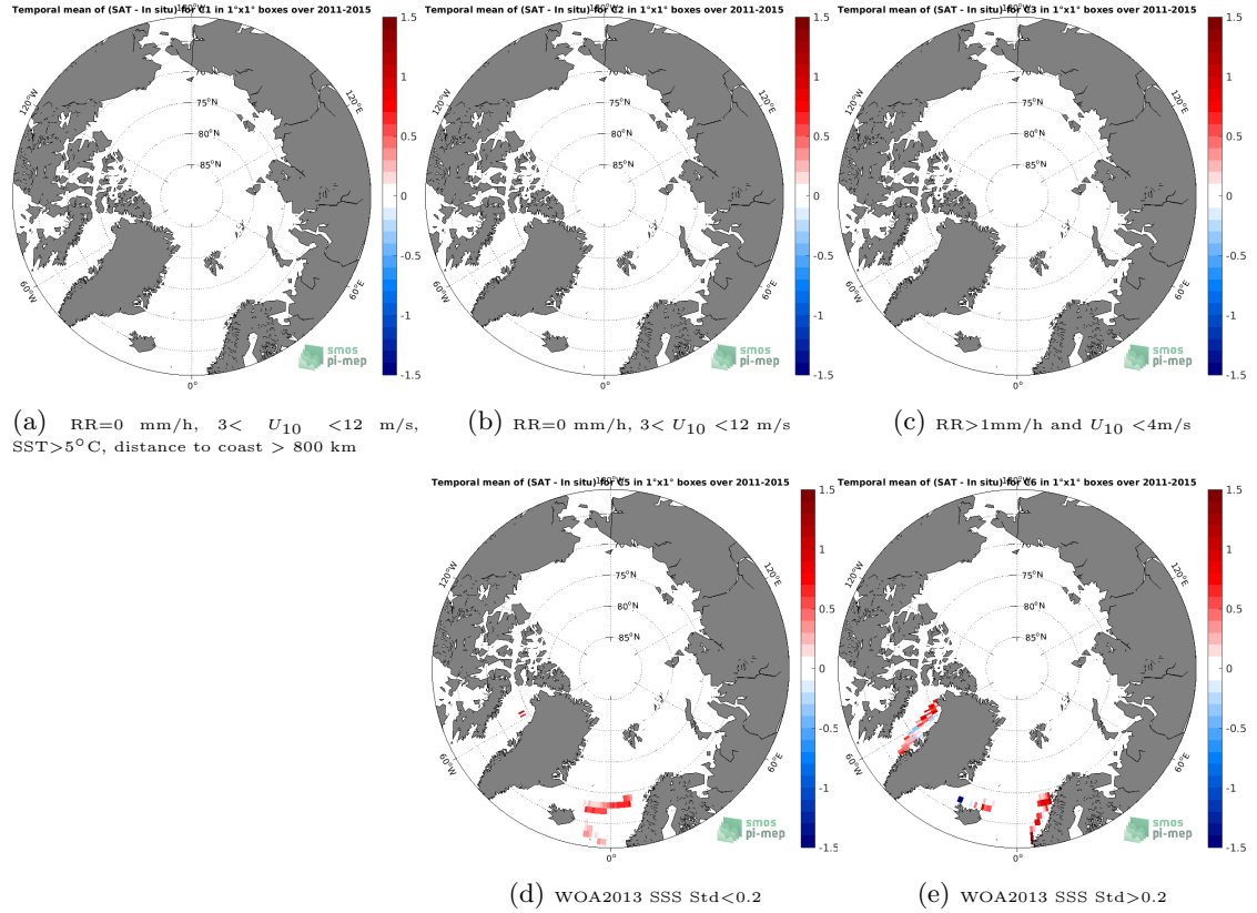
Figure 12: Temporal mean gridded over spatial boxes of size 1^{\circ}\times 1^{\circ} of \Delta\text{SSS} (Aquarius SSS L3 CAP v5 - Monthly (JPL) - TSG (LEGOS-DM)) for 5 different subdatasets corresponding to: \text{RR}=0 mm/h, 3 < U_{10} < 12 m/s, \text{SST} > 5^{\circ}\text{C} , distance to coast > 800 km (a), \text{RR}=0 mm/h, 3 < U_{10} < 12 m/s (b), \text{RR} > 1 mm/h and U_{10} < 4 m/s (c), WOA2013 SSS Std < 0.2 (d), WOA2013 SSS Std > 0.2 (e).
