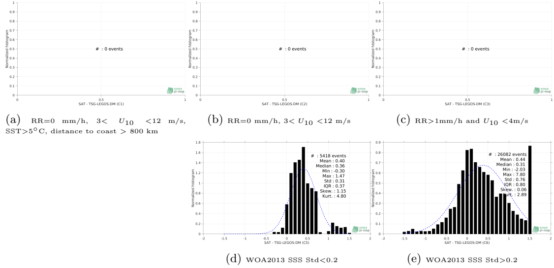
Figure 13: Normalized histogram of \Delta\text{SSS} (Aquarius-L3-JPL-V5-MONTHLY - TSG-LEGOS-DM) for 5 different subdatasets corresponding to: RR=0 mm/h, 3 < U_{10} < 12 m/s, SST > 5^\circ\text{C} , distance to coast > 800 km (a), RR=0 mm/h, 3 < U_{10} < 12 m/s (b), RR > 1\text{mm/h} and U_{10} < 4\text{m/s} (c), WOA2013 SSS Std < 0.2 (d), WOA2013 SSS Std > 0.2 (e).
