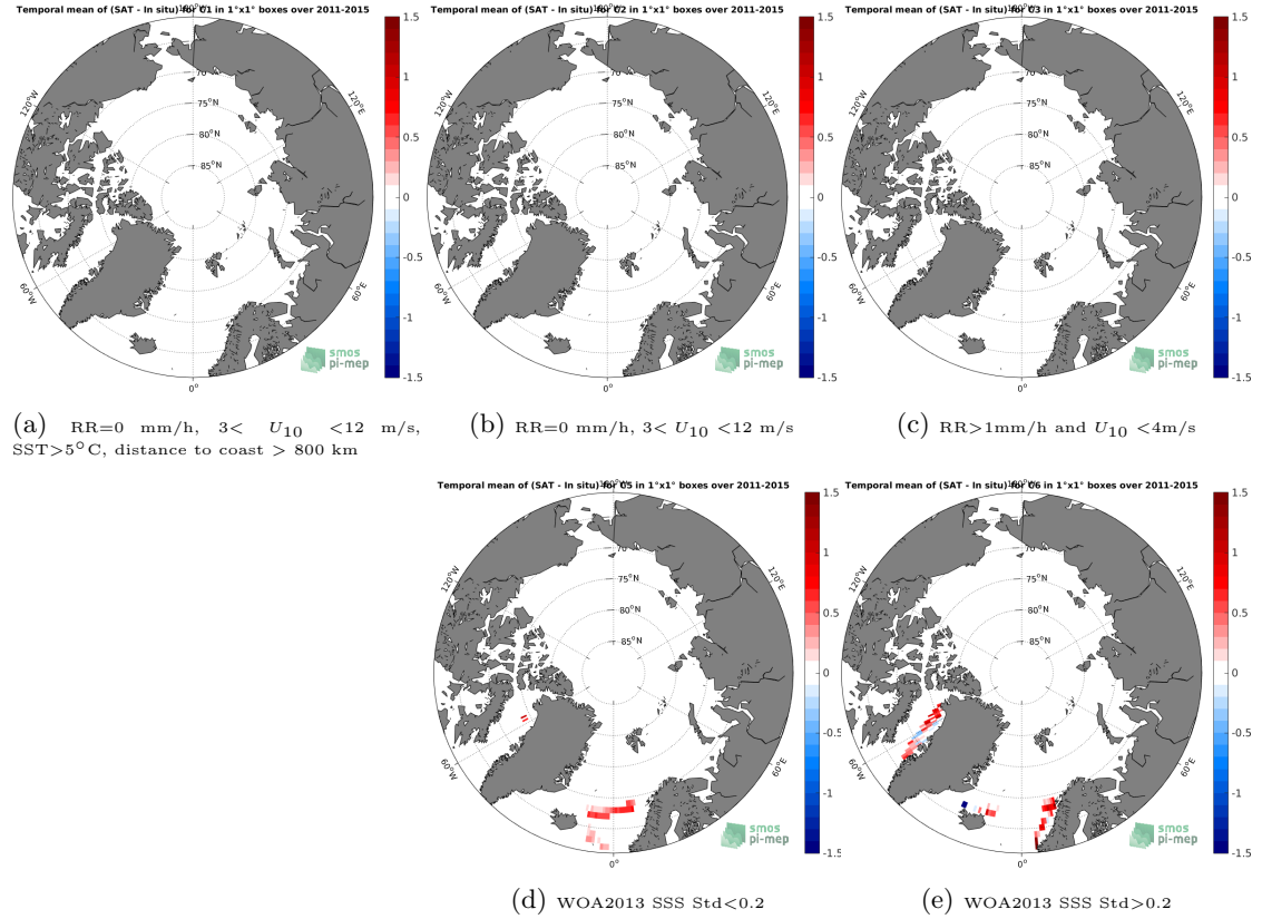
Figure 12: Temporal mean gridded over spatial boxes of size 1^{\circ}\times 1^{\circ} of \Delta\text{SSS} (Aquarius-L3-JPL-V5-MONTHLY - TSG-LEGOS-DM) for 5 different subdatasets corresponding to:RR=0 mm/h, 3 < U_{10} < 12 m/s, SST >5^{\circ}\text{C} , distance to coast > 800 km (a), RR=0 mm/h, 3 < U_{10} < 12 m/s (b), RR >1 mm/h and U_{10} < 4 m/s (c), WOA2013 SSS Std <0.2 (d), WOA2013 SSS Std >0.2 (e).
