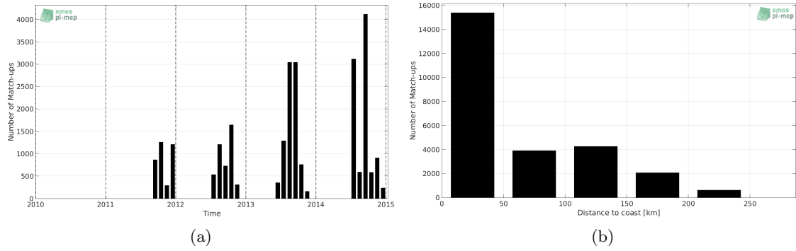
Figure 1: Number of match-ups between TSG-LEGOS-DM and Aquarius-L3-JPL-V5-MONTHLY SSS as a function of time (a) and as function of the distance to coast (b) over the Arctic Ocean Pi-MEP region and for the full satellite product period.
