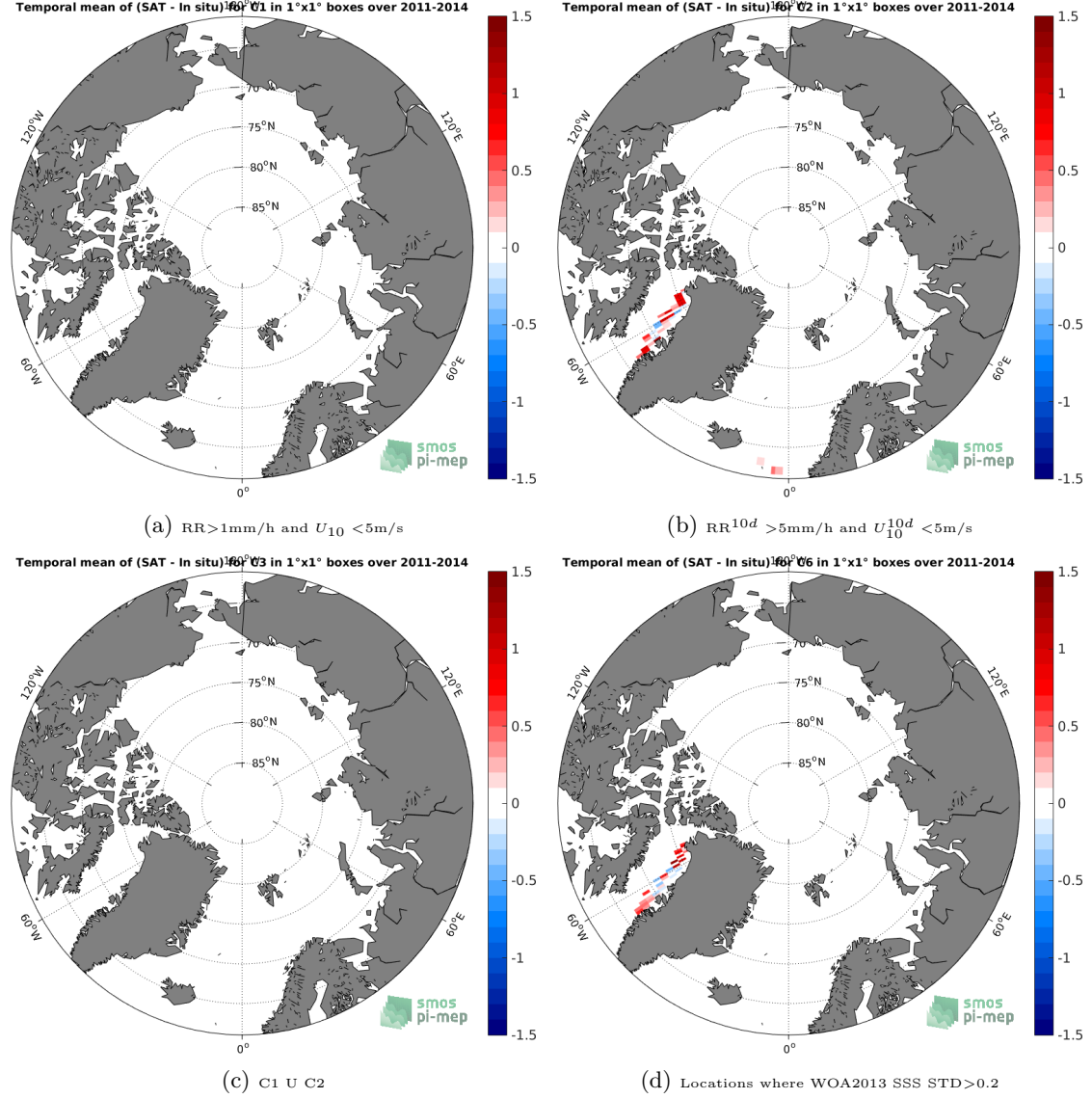
Figure 12: Temporal mean gridded over spatial boxes of size 1^\circ \times 1^\circ of \Delta SSS (Aquarius-L3-JPL-V5-MONTHLY - TSG-LEGOS-DM) for 4 different subdatasets corresponding to: RR > 1\text{mm/h} and U_{10} < 5\text{m/s} (a), RR^{10d} > 5\text{mm/h} and U_{10}^{10d} < 5\text{m/s} (b), C1 U C2 (c), Locations where WOA2013 SSS STD > 0.2 (d).
