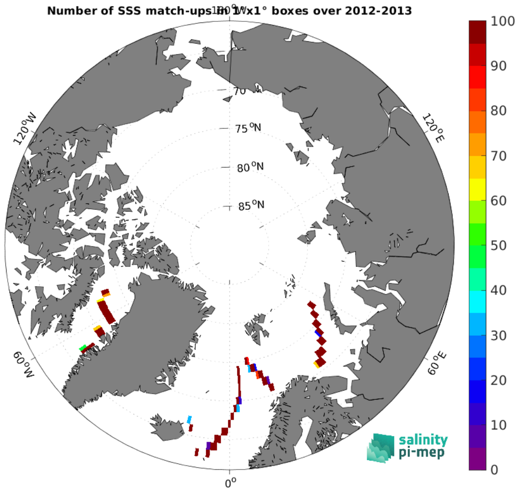
Figure 5: Number of SSS match-ups between TSG (GOSUD-Sailing-ship) SSS and the Aquarius SSS L3 CAP v5 - Monthly (JPL) SSS product for the Arctic Ocean Pi-MEP region over 1^\circ \times 1^\circ boxes and for the full satellite product period.
