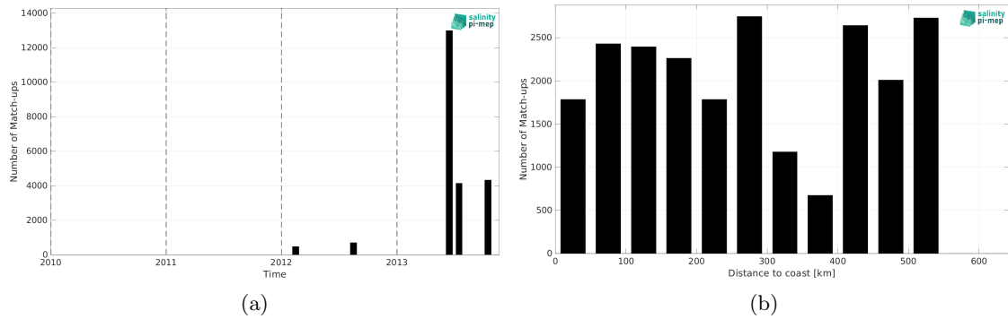
Figure 2: Number of match-ups between TSG (GOSUD-Sailing-ship) and Aquarius SSS L3 CAP v5 - Monthly (JPL) SSS as a function of time (a) and as function of the distance to coast (b) over the Arctic Ocean Pi-MEP region and for the full satellite product period.
