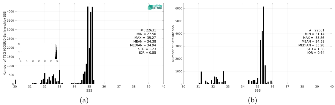
Figure 3: Histograms of SSS from TSG (GOSUD-Sailing-ship) (a) and Aquarius SSS L3 CAP v5 - Monthly (JPL) (b) considering all match-up pairs per bins of 0.1 over the Arctic Ocean Pi-MEP region and for the full satellite product period.
