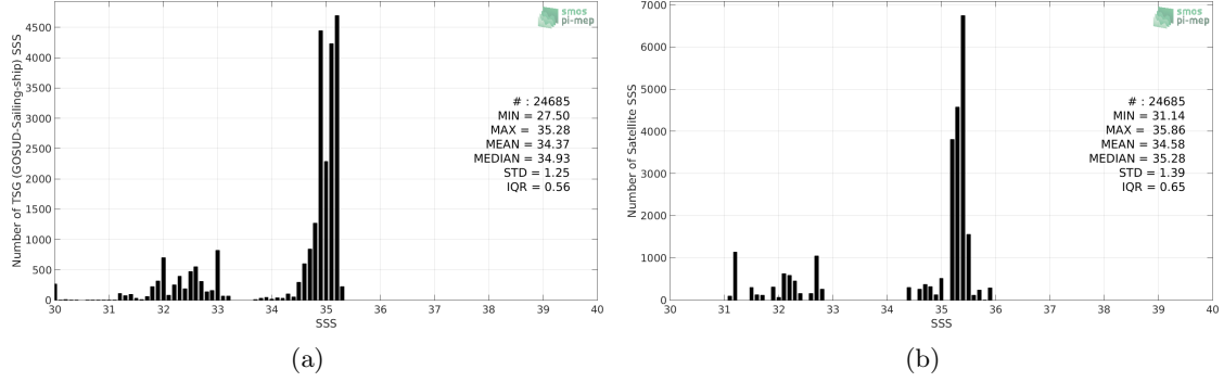
Figure 2: Histograms of SSS from TSG (GOSUD-Sailing-ship) (a) and Aquarius SSS L3 CAP v5 - Monthly (JPL) (b) considering all match-up pairs per bins of 0.1 over the Arctic Ocean Pi-MEP region and for the full satellite product period.
