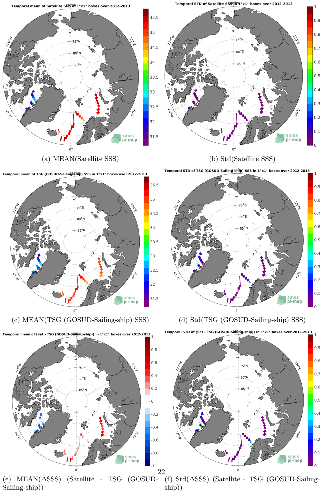
Figure 6: Temporal mean (left) and Std (right) of SSS from Aquarius SSS L3 CAP v5 - Monthly (JPL) (top), TSG (GOSUD-Sailing-ship) (middle), and of \Delta SSS (Satellite - TSG (GOSUD-Sailing-ship)). Only match-up pairs are used to generate these maps.
