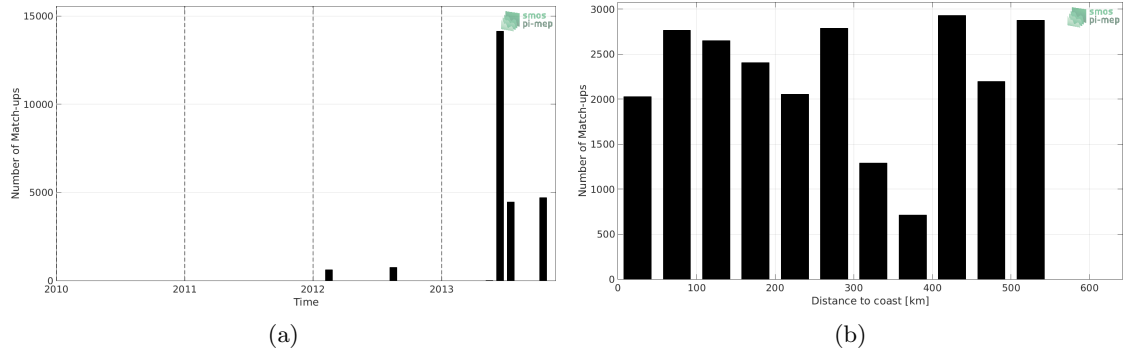
Figure 1: Number of match-ups between TSG (GOSUD-Sailing-ship) and Aquarius SSS L3 CAP v5 - Monthly (JPL) SSS as a function of time (a) and as function of the distance to coast (b) over the Arctic Ocean Pi-MEP region and for the full satellite product period.
