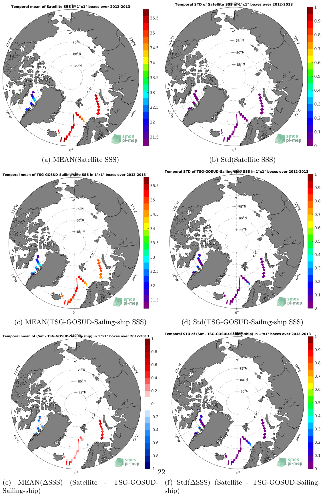
Figure 6: Temporal mean (left) and Std (right) of SSS from Aquarius-L3-JPL-V5-MONTHLY (top), TSG-GOSUD-Sailing-ship (middle), and of \Delta SSS (Satellite - TSG-GOSUD-Sailing-ship). Only match-up pairs are used to generate these maps.
