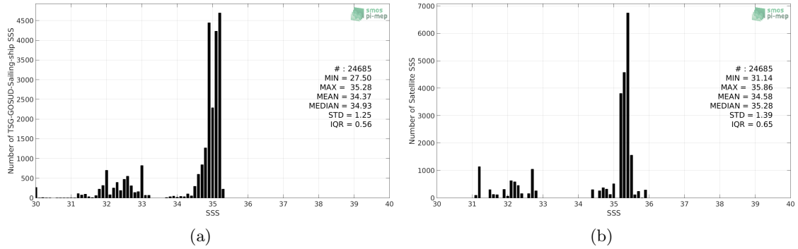
Figure 2: Histograms of SSS from TSG-GOSUD-Sailing-ship (a) and Aquarius-L3-JPL-V5-MONTHLY (b) considering all match-up pairs per bins of 0.1 over the Arctic Ocean Pi-MEP region and for the full satellite product period.
