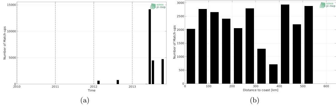
Figure 1: Number of match-ups between TSG-GOSUD-Sailing-ship and Aquarius-L3-JPL-V5-MONTHLY SSS as a function of time (a) and as function of the distance to coast (b) over the Arctic Ocean Pi-MEP region and for the full satellite product period.
