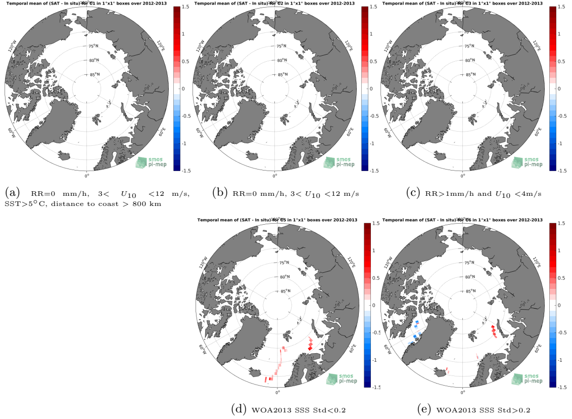
Figure 12: Temporal mean gridded over spatial boxes of size 1^\circ \times 1^\circ of \Delta SSS (Aquarius-L3-JPL-V5-MONTHLY - TSG-GOSUD-Sailing-ship) for 5 different subdatasets corresponding to: RR=0 mm/h, 3 < U_{10} < 12 m/s, SST > 5^\circ\text{C} , distance to coast > 800 km (a), RR=0 mm/h, 3 < U_{10} < 12 m/s (b), RR > 1 mm/h and U_{10} < 4 m/s (c), WOA2013 SSS Std < 0.2 (d), WOA2013 SSS Std > 0.2 (e).
