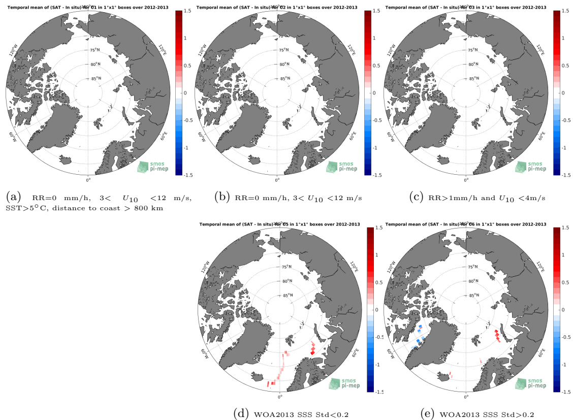
Figure 12: Temporal mean gridded over spatial boxes of size 1^\circ \times 1^\circ of \Delta SSS (Aquarius-L3-JPL-V5-MONTHLY - TSG-GOSUD-Sailing-ship) for 5 different subdatasets corresponding to:RR=0 mm/h, 3 < U_{10} < 12 m/s, SST >5^\circ C, distance to coast > 800 km (a), RR=0 mm/h, 3 < U_{10} < 12 m/s (b), RR >1 mm/h and U_{10} < 4 m/s (c), WOA2013 SSS Std <0.2 (d), WOA2013 SSS Std >0.2 (e).
