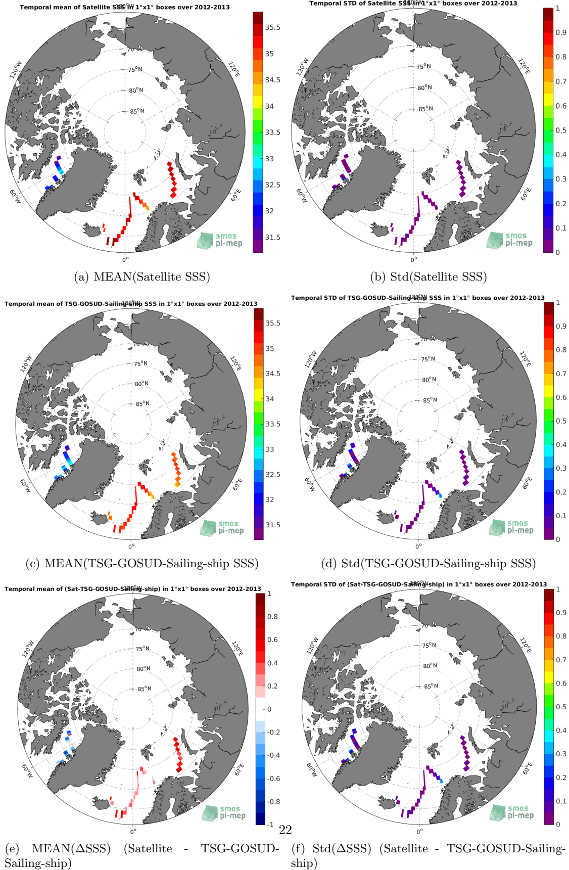
Figure 6: Temporal mean (left) and Std (right) of SSS from Aquarius-L3-JPL-V5-MONTHLY (top), TSG-GOSUD-Sailing-ship (middle), and of \Delta SSS (Satellite - TSG-GOSUD-Sailing-ship). Only match-up pairs are used to generate these maps.
