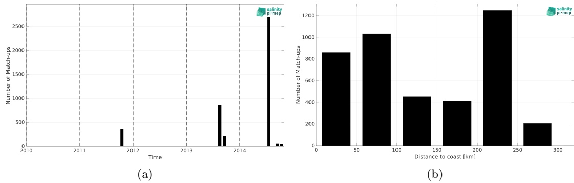
Figure 2: Number of match-ups between TSG (Amundsen) and Aquarius SSS L3 CAP v5 - Monthly (JPL) SSS as a function of time (a) and as function of the distance to coast (b) over the Arctic Ocean Pi-MEP region and for the full satellite product period.
