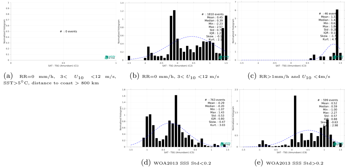
Figure 15: Normalized histogram of \Delta SSS (Aquarius SSS L3 CAP v5 - Monthly (JPL) - TSG (Amundsen)) for 5 different subdatasets corresponding to: RR=0 mm/h, 3 < U_{10} < 12 m/s, SST>5°C, distance to coast > 800 km (a), RR=0 mm/h, 3 < U_{10} < 12 m/s (b), RR>1mm/h and U_{10} < 4 m/s (c), WOA2013 SSS Std<0.2 (d), WOA2013 SSS Std>0.2 (e).
