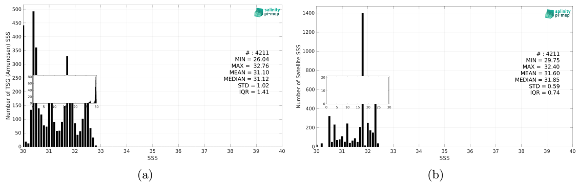
Figure 3: Histograms of SSS from TSG (Amundsen) (a) and Aquarius SSS L3 CAP v5 - Monthly (JPL) (b) considering all match-up pairs per bins of 0.1 over the Arctic Ocean Pi-MEP region and for the full satellite product period.
