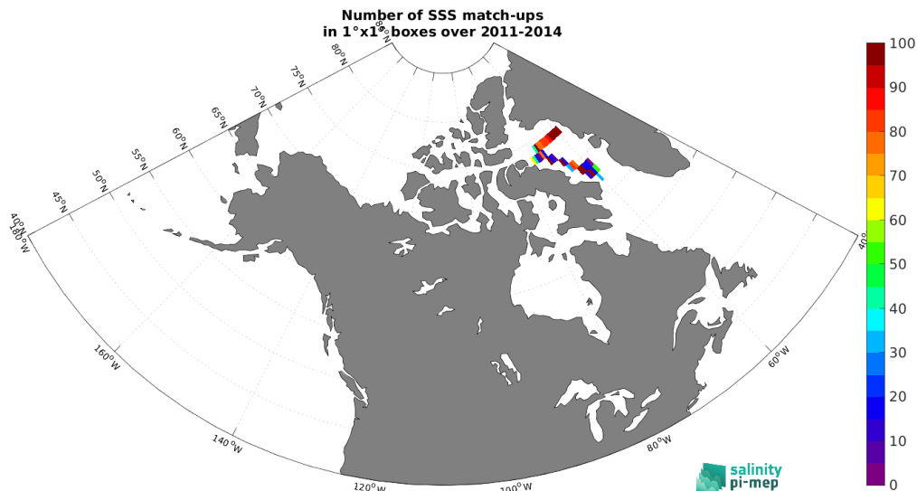
Figure 5: Number of SSS match-ups between TSG (Amundsen) SSS and the Aquarius SSS L3 CAP v5 - Monthly (JPL) SSS product for the Arctic Ocean Pi-MEP region over 1^\circ \times 1^\circ boxes and for the full satellite product period.
