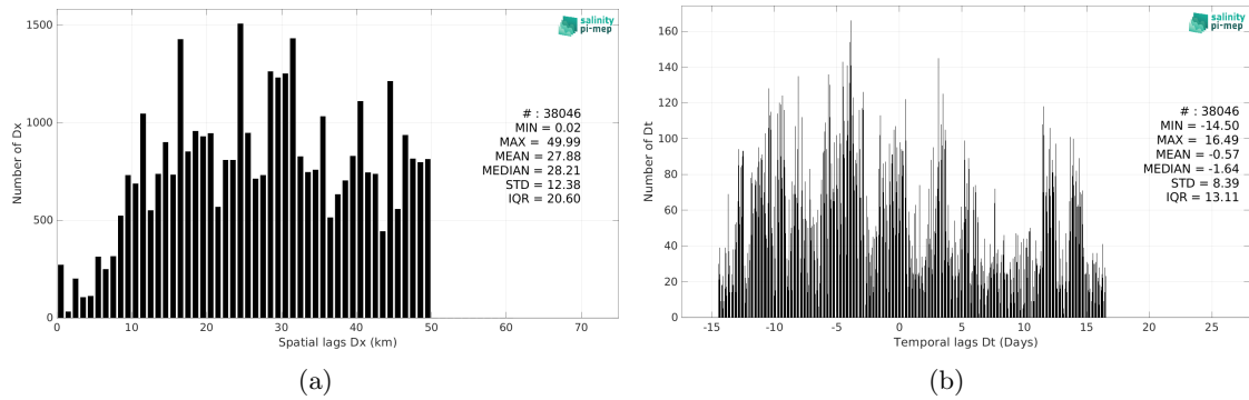
Figure 6: Histograms of the spatial (a) and temporal (b) lags between the location/time of the ICES measurement and the date of the corresponding Aquarius SSS L3 CAP v5 - Monthly (JPL) SSS pixel.
