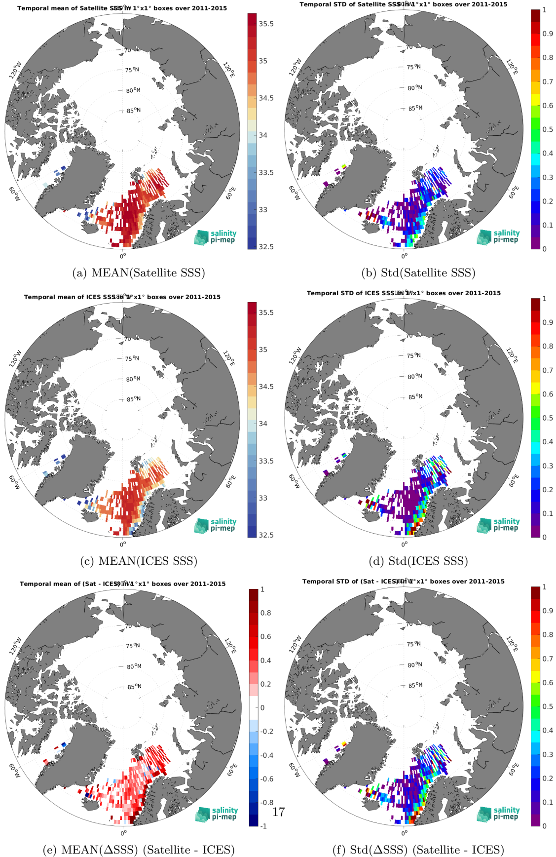
Figure 7: Temporal mean (left) and Std (right) of SSS from Aquarius SSS L3 CAP v5 - Monthly (JPL) (top), ICES (middle), and of \Delta SSS (Satellite - ICES). Only match-up pairs are used to generate these maps.
