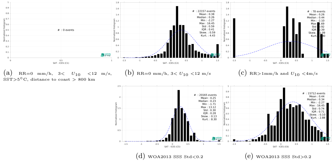
Figure 15: Normalized histogram of \Delta SSS (Aquarius SSS L3 CAP v5 - Monthly (JPL) - ICES) for 5 different subdatasets corresponding to: RR=0 mm/h, 3 < U_{10} < 12 m/s, SST > 5°C, distance to coast > 800 km (a), RR=0 mm/h, 3 < U_{10} < 12 m/s (b), RR > 1mm/h and U_{10} < 4 m/s (c), WOA2013 SSS Std < 0.2 (d), WOA2013 SSS Std > 0.2 (e).
