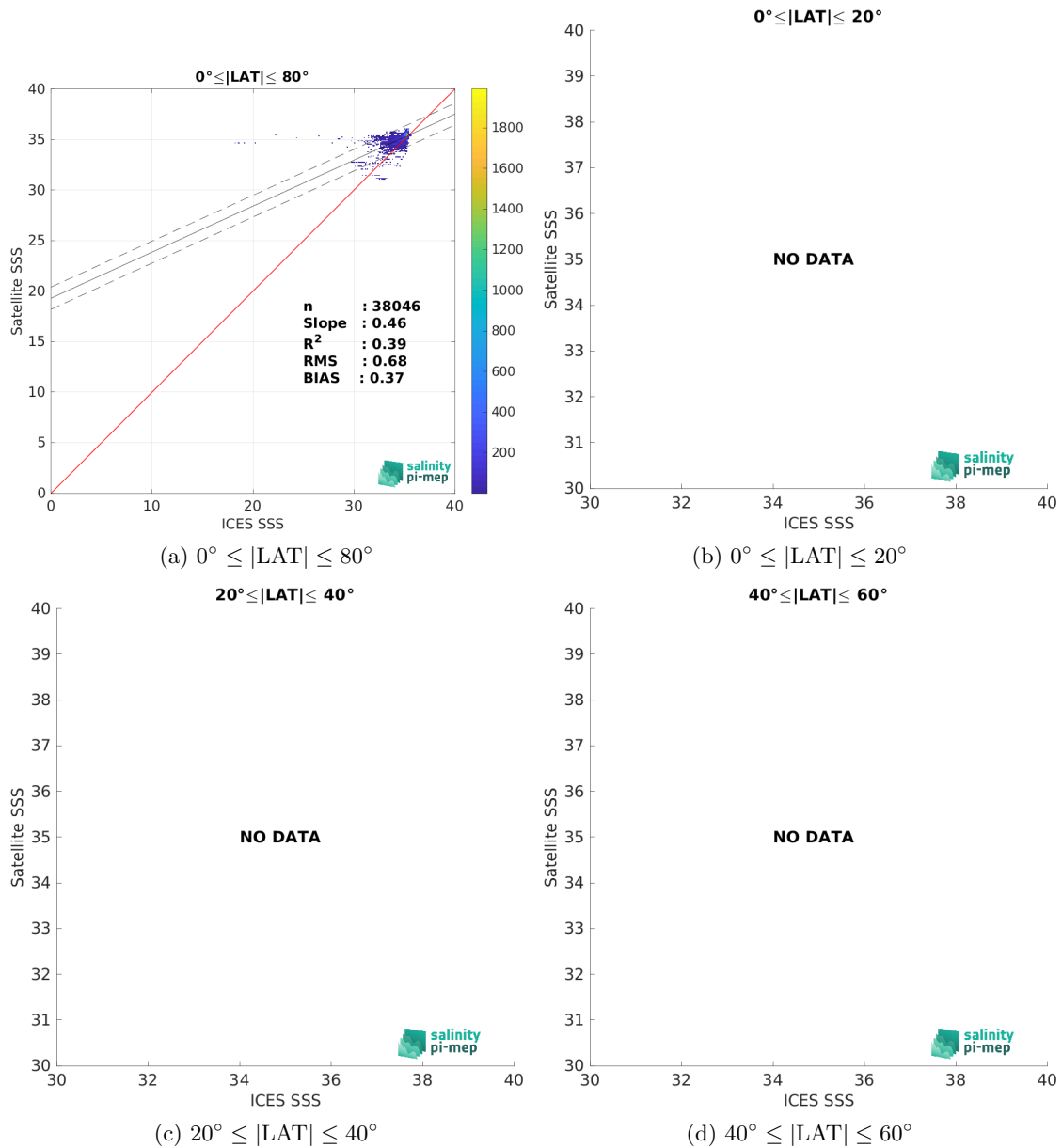
Figure 10: Contour maps of the concentration of Aquarius SSS L3 CAP v5 - Monthly (JPL) SSS (y-axis) versus ICES SSS (x-axis) at match-up pairs for different latitude bands. For each plot, the red line shows x=y . The black thin and dashed lines indicate a linear fit through the data cloud and the \pm 95\% confidence levels, respectively. The number match-up pairs n , the slope and R^2 coefficient of the linear fit, the root mean square (RMS) and the mean bias between satellite and in situ data are indicated for each latitude band in each plots.
