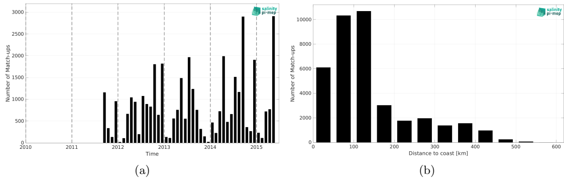
Figure 2: Number of match-ups between ICES and Aquarius SSS L3 CAP v5 - Monthly (JPL) SSS as a function of time (a) and as function of the distance to coast (b) over the Arctic Ocean Pi-MEP region and for the full satellite product period.
