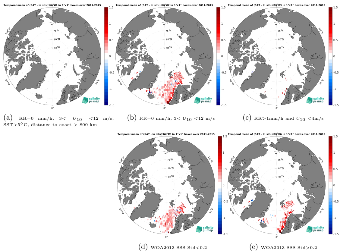
Figure 14: Temporal mean gridded over spatial boxes of size 1^\circ \times 1^\circ of \Delta SSS (Aquarius SSS L3 CAP v5 - Monthly (JPL) - ICES) for 5 different subdatasets corresponding to: RR=0 mm/h, 3 < U_{10} < 12 m/s, SST > 5°C, distance to coast > 800 km (a), RR=0 mm/h, 3 < U_{10} < 12 m/s (b), RR > 1mm/h and U_{10} < 4 m/s (c), WOA2013 SSS Std < 0.2 (d), WOA2013 SSS Std > 0.2 (e).
