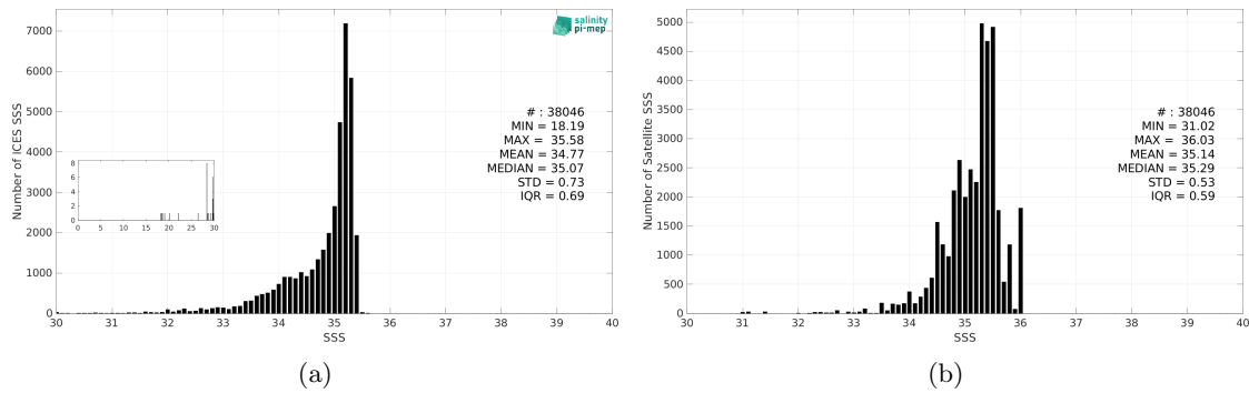
Figure 3: Histograms of SSS from ICES (a) and Aquarius SSS L3 CAP v5 - Monthly (JPL) (b) considering all match-up pairs per bins of 0.1 over the Arctic Ocean Pi-MEP region and for the full satellite product period.
