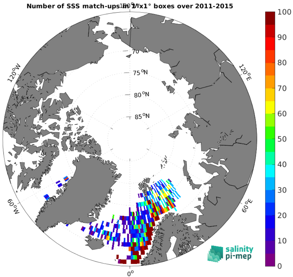
Figure 5: Number of SSS match-ups between ICES SSS and the Aquarius SSS L3 CAP v5 - Monthly (JPL) SSS product for the Arctic Ocean Pi-MEP region over 1^\circ \times 1^\circ boxes and for the full satellite product period.
