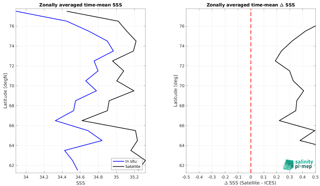
Figure 9: Left panel: Zonal mean SSS from Aquarius SSS L3 CAP v5 - Monthly (JPL) satellite product (black) and from ICES (blue). Right panel: Zonal mean of \Delta SSS (Satellite - ICES) for all the collected Pi-MEP match-up pairs estimated over the full satellite product period.
