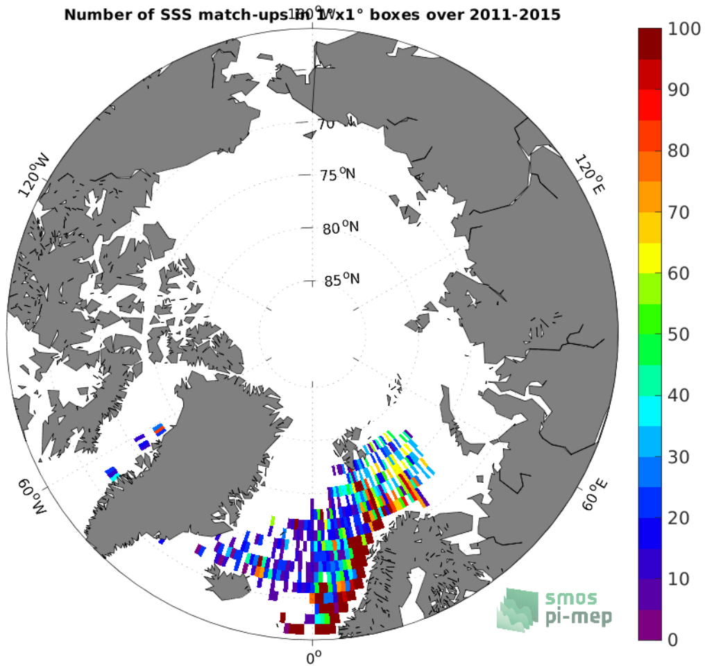
Figure 4: Number of SSS match-ups between ICES SSS and the Aquarius SSS L3 CAP v5 - Monthly (JPL) SSS product for the Arctic Ocean Pi-MEP region over 1^{\circ} \times 1^{\circ} boxes and for the full satellite product period.
