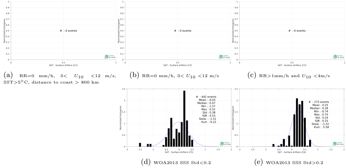
Figure 12: Normalized histogram of \Delta\text{SSS} (Aquarius SSS L3 CAP v5 - Monthly (JPL) - Surface drifters) for 5 different subdatasets corresponding to: RR=0 mm/h, 3 < U_{10} < 12 m/s, SST > 5^\circ\text{C} , distance to coast > 800 km (a), RR=0 mm/h, 3 < U_{10} < 12 m/s (b), RR > 1\text{mm/h} and U_{10} < 4\text{m/s} (c), WOA2013 SSS Std < 0.2 (d), WOA2013 SSS Std > 0.2 (e).
