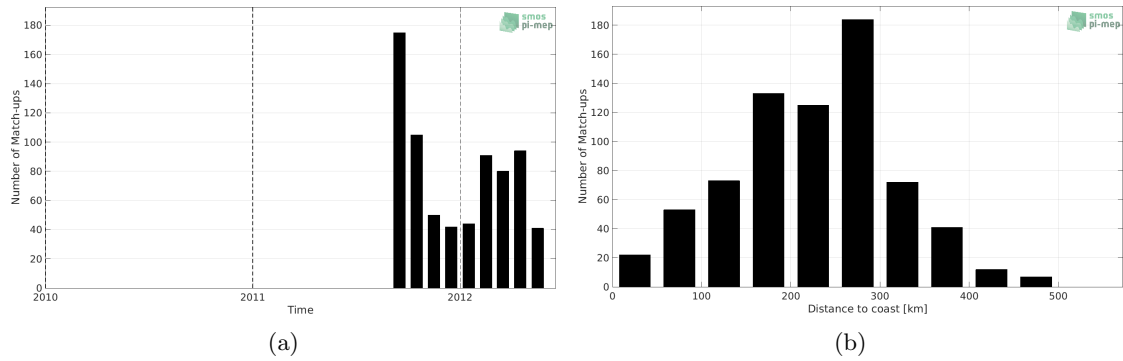
Figure 1: Number of match-ups between Surface drifters and Aquarius SSS L3 CAP v5 - Monthly (JPL) SSS as a function of time (a) and as function of the distance to coast (b) over the Arctic Ocean Pi-MEP region and for the full satellite product period.
