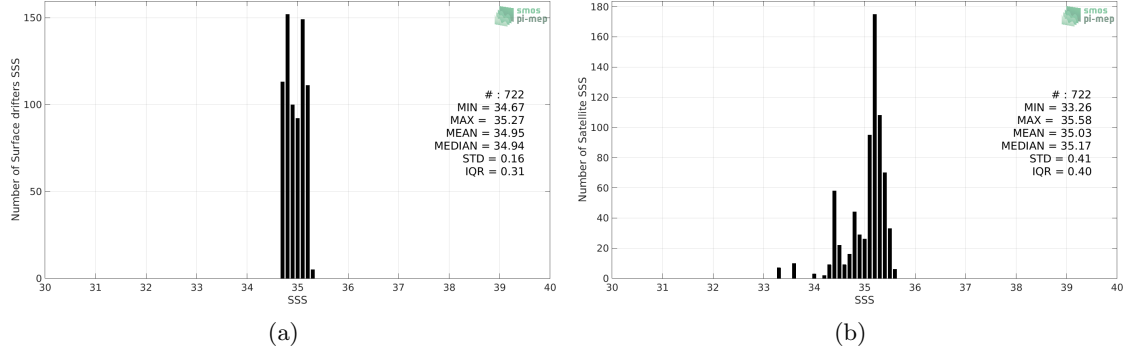
Figure 2: Histograms of SSS from Surface drifters (a) and Aquarius SSS L3 CAP v5 - Monthly (JPL) (b) considering all match-up pairs per bins of 0.1 over the Arctic Ocean Pi-MEP region and for the full satellite product period.
