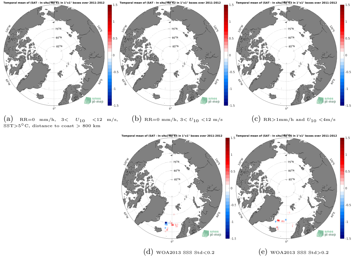
Figure 11: Temporal mean gridded over spatial boxes of size 1^{\circ}\times 1^{\circ} of \Delta\text{SSS} (Aquarius SSS L3 CAP v5 - Monthly (JPL) - Surface drifters) for 5 different subdatasets corresponding to: RR=0 mm/h, 3 < U_{10} < 12 m/s, SST >5^{\circ}\text{C} , distance to coast > 800 km (a), RR=0 mm/h, 3 < U_{10} < 12 m/s (b), RR >1 mm/h and U_{10} < 4 m/s (c), WOA2013 SSS Std <0.2 (d), WOA2013 SSS Std >0.2 (e).
