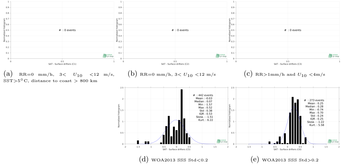
Figure 12: Normalized histogram of \Delta\text{SSS} (Aquarius-L3-JPL-V5-MONTHLY - Surface drifters) for 5 different subdatasets corresponding to: RR=0 mm/h, 3 < U_{10} < 12 m/s, SST >5^{\circ}\text{C} , distance to coast > 800 km (a), RR=0 mm/h, 3 < U_{10} < 12 m/s (b), RR>1\text{mm/h} and U_{10} < 4\text{m/s} (c), WOA2013 SSS Std <0.2 (d), WOA2013 SSS Std >0.2 (e).
