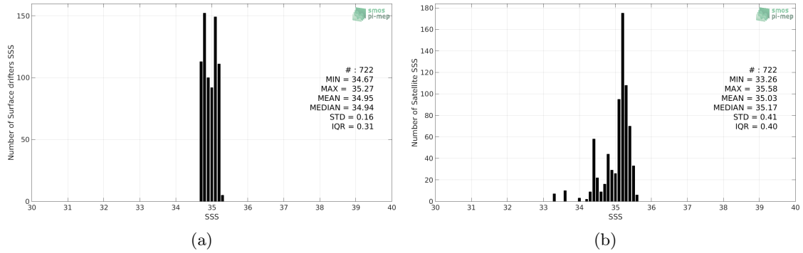
Figure 2: Histograms of SSS from Surface drifters (a) and Aquarius-L3-JPL-V5-MONTHLY (b) considering all match-up pairs per bins of 0.1 over the Arctic Ocean Pi-MEP region and for the full satellite product period.
