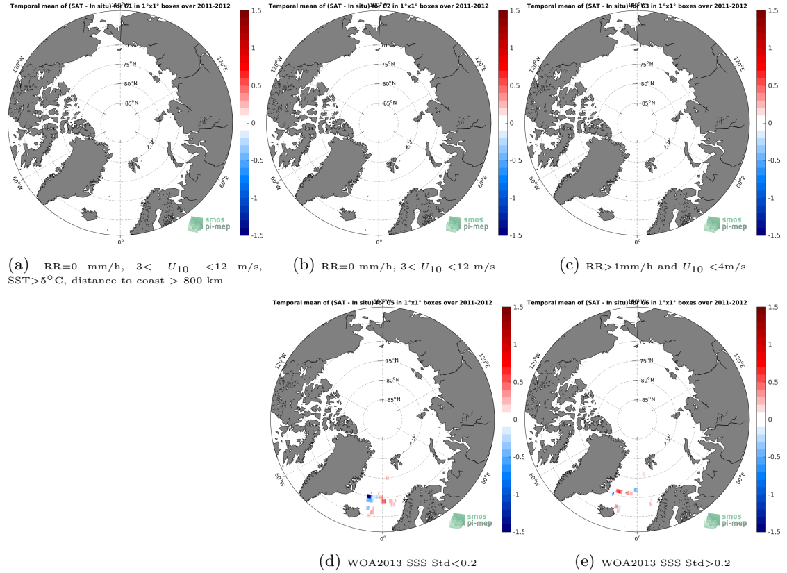
Figure 11: Temporal mean gridded over spatial boxes of size 1^{\circ}\times 1^{\circ} of \Delta\text{SSS} (Aquarius-L3-JPL-V5-MONTHLY - Surface drifters) for 5 different subdatasets corresponding to:RR=0 mm/h, 3 < U_{10} < 12 m/s, SST >5^{\circ}\text{C} , distance to coast > 800 km (a), RR=0 mm/h, 3 < U_{10} < 12 m/s (b), RR >1 mm/h and U_{10} < 4 m/s (c), WOA2013 SSS Std <0.2 (d), WOA2013 SSS Std >0.2 (e).
