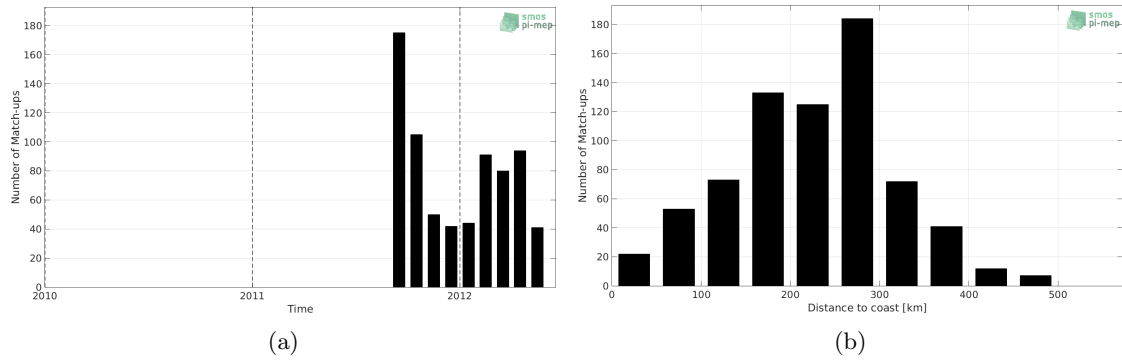
Figure 1: Number of match-ups between Surface drifters and Aquarius-L3-JPL-V5-MONTHLY SSS as a function of time (a) and as function of the distance to coast (b) over the Arctic Ocean Pi-MEP region and for the full satellite product period.
