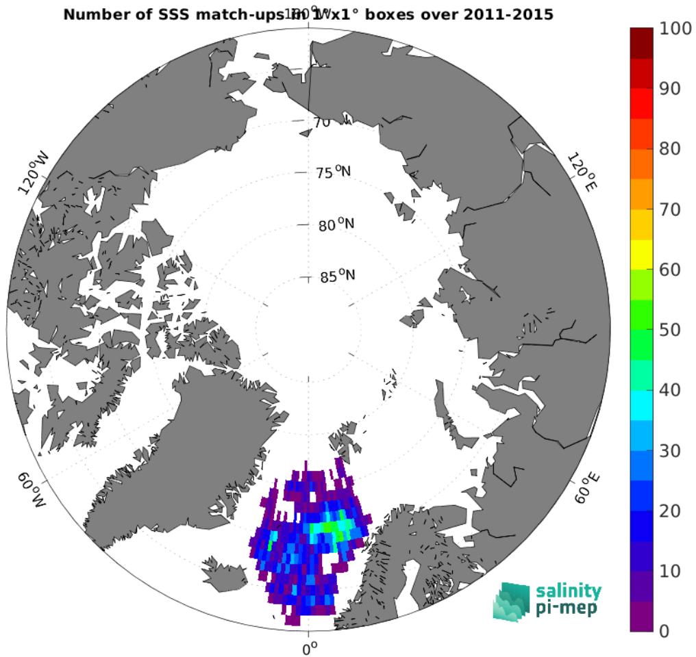
Figure 4: Number of SSS match-ups between Argo SSS and the Aquarius SSS L3 CAP v5 - Monthly (JPL) SSS product for the Arctic Ocean Pi-MEP region over 1^\circ \times 1^\circ boxes and for the full satellite product period.
