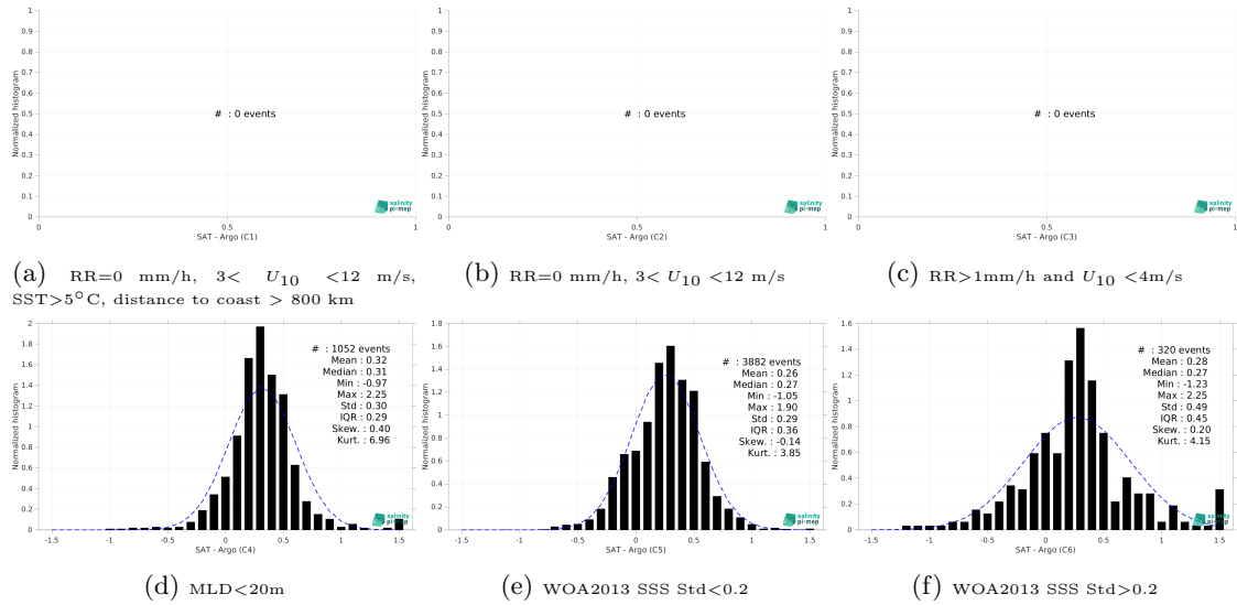
Figure 13: Normalized histogram of \Delta\text{SSS} (Aquarius SSS L3 CAP v5 - Monthly (JPL) - Argo) for 6 different subdatasets corresponding to: RR=0 mm/h, 3 < U_{10} < 12 m/s, SST > 5^{\circ}\text{C} , distance to coast > 800 km (a), RR=0 mm/h, 3 < U_{10} < 12 m/s (b), RR > 1\text{mm/h} and U_{10} < 4\text{m/s} (c), MLD < 20\text{m} (d), WOA2013 SSS Std < 0.2 (e), WOA2013 SSS Std > 0.2 (f).
