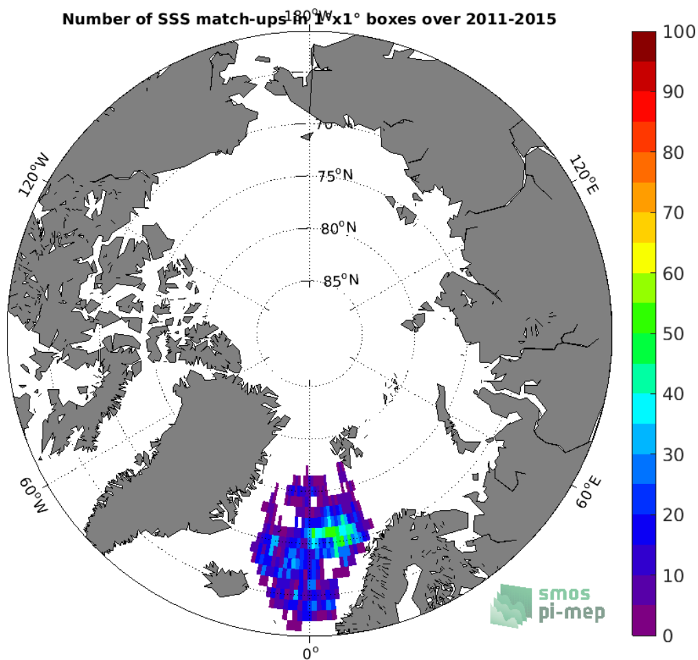
Figure 4: Number of SSS match-ups between Argo SSS and the Aquarius SSS L3 CAP v5 - Monthly (JPL) SSS product for the Arctic Ocean Pi-MEP region over 1°x1° boxes and for the full satellite product period.
