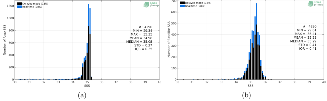
Figure 2: Histograms of SSS from Argo (a) and Aquarius SSS L3 CAP v5 - Monthly (JPL) (b) considering all match-up pairs per bins of 0.1 over the Arctic Ocean Pi-MEP region and for the full satellite product period.
