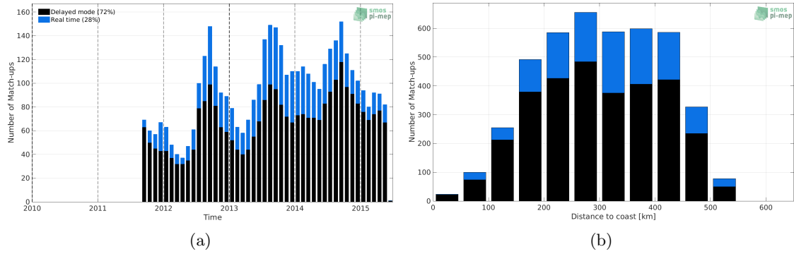
Figure 1: Number of match-ups between Argo and Aquarius SSS L3 CAP v5 - Monthly (JPL) SSS as a function of time (a) and as function of the distance to coast (b) over the Arctic Ocean Pi-MEP region and for the full satellite product period.
