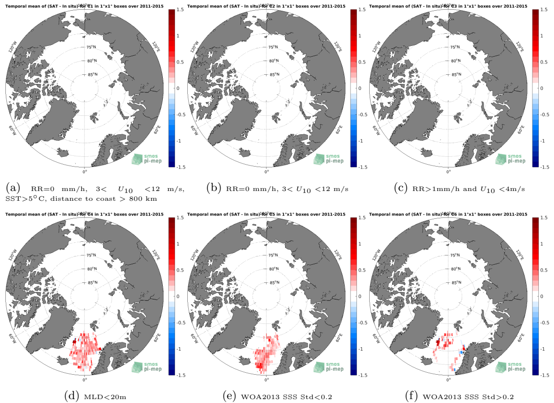
Figure 12: Temporal mean gridded over spatial boxes of size 1^{\circ}\times 1^{\circ} of \Delta\text{SSS} (Aquarius SSS L3 CAP v5 - Monthly (JPL) - Argo) for 6 different subdatasets corresponding to: RR=0 mm/h, 3 < U_{10} < 12 m/s, SST > 5^{\circ}\text{C} , distance to coast > 800 km (a), RR=0 mm/h, 3 < U_{10} < 12 m/s (b), RR > 1 mm/h and U_{10} < 4 m/s (c), MLD < 20\text{m} (d), WOA2013 SSS Std < 0.2 (e), WOA2013 SSS Std > 0.2 (f).
