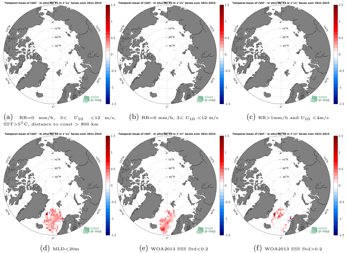
Figure 12: Temporal mean gridded over spatial boxes of size 1^{\circ}\times 1^{\circ} of \Delta\text{SSS} (Aquarius-L3-JPL-V5-MONTHLY - Argo) for 6 different subdatasets corresponding to: RR=0 mm/h, 3 < U_{10} < 12 m/s, SST > 5^{\circ}\text{C} , distance to coast > 800 km (a), RR=0 mm/h, 3 < U_{10} < 12 m/s (b), RR > 1 mm/h and U_{10} < 4 m/s (c), MLD < 20\text{m} (d), WOA2013 SSS Std < 0.2 (e), WOA2013 SSS Std > 0.2 (f).
