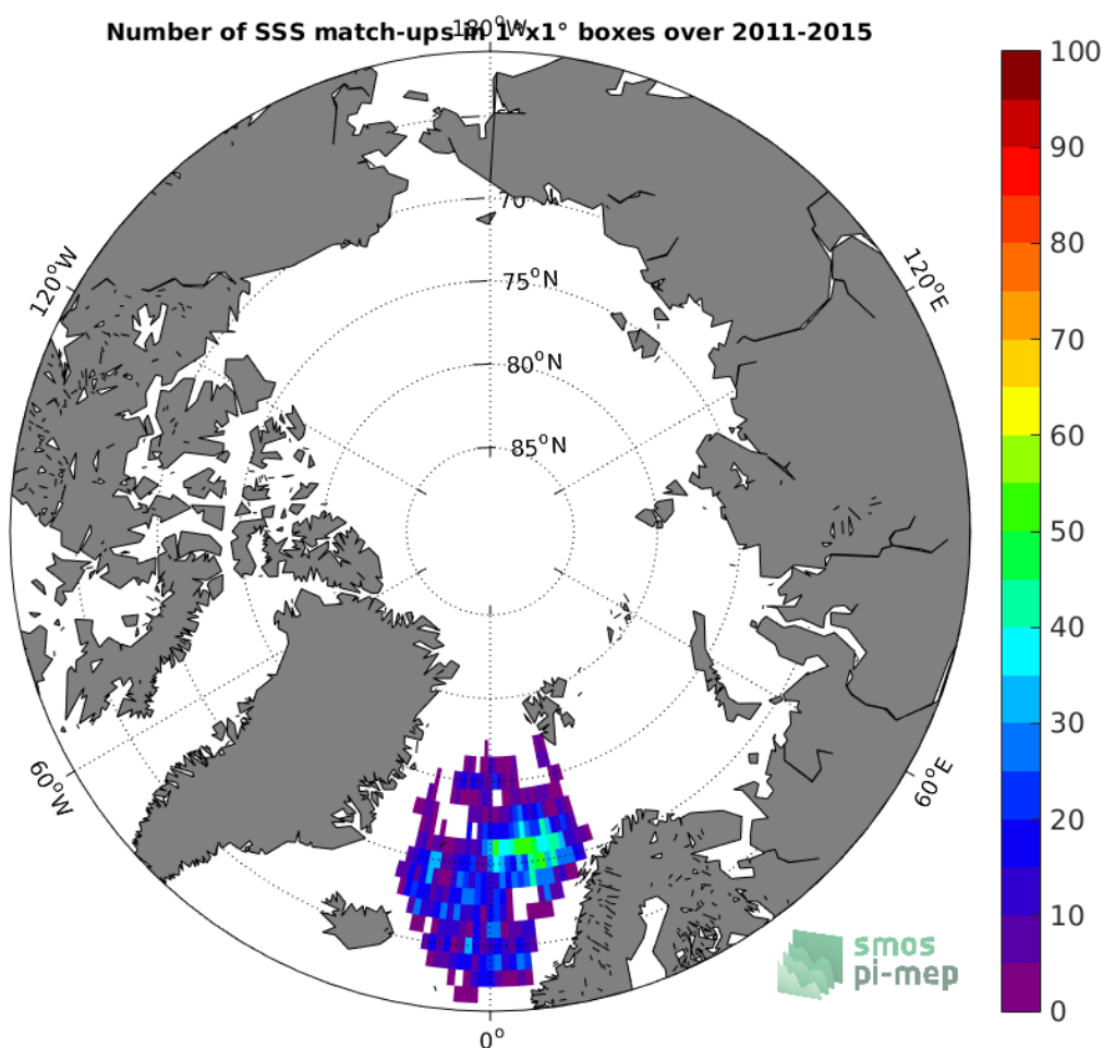
Figure 4: Number of SSS match-ups between Argo SSS and the Aquarius-L3-JPL-V5-MONTHLY SSS product for the Arctic Ocean Pi-MEP region over 1°x1° boxes and for the full satellite product period.
