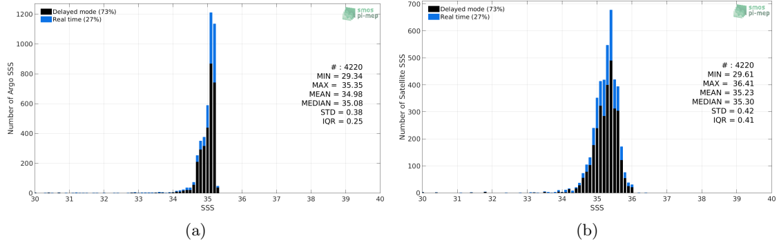
Figure 2: Histograms of SSS from Argo (a) and Aquarius-L3-JPL-V5-MONTHLY (b) considering all match-up pairs per bins of 0.1 over the Arctic Ocean Pi-MEP region and for the full satellite product period.
