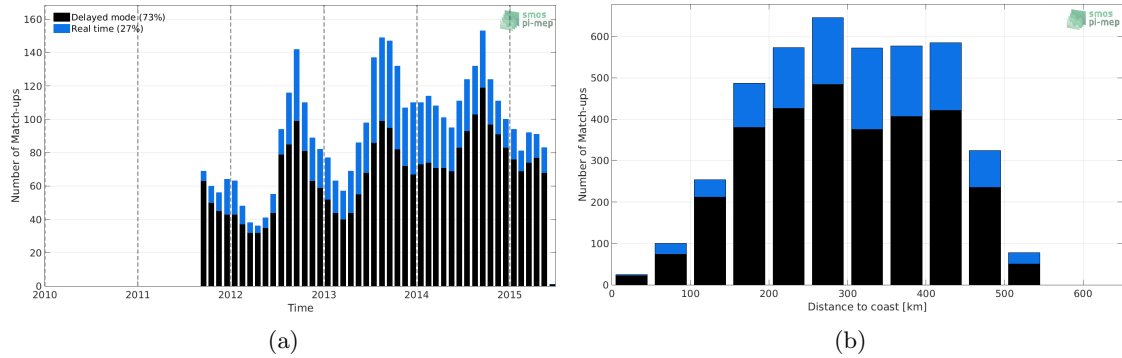
Figure 1: Number of match-ups between Argo and Aquarius-L3-JPL-V5-MONTHLY SSS as a function of time (a) and as function of the distance to coast (b) over the Arctic Ocean Pi-MEP region and for the full satellite product period.
