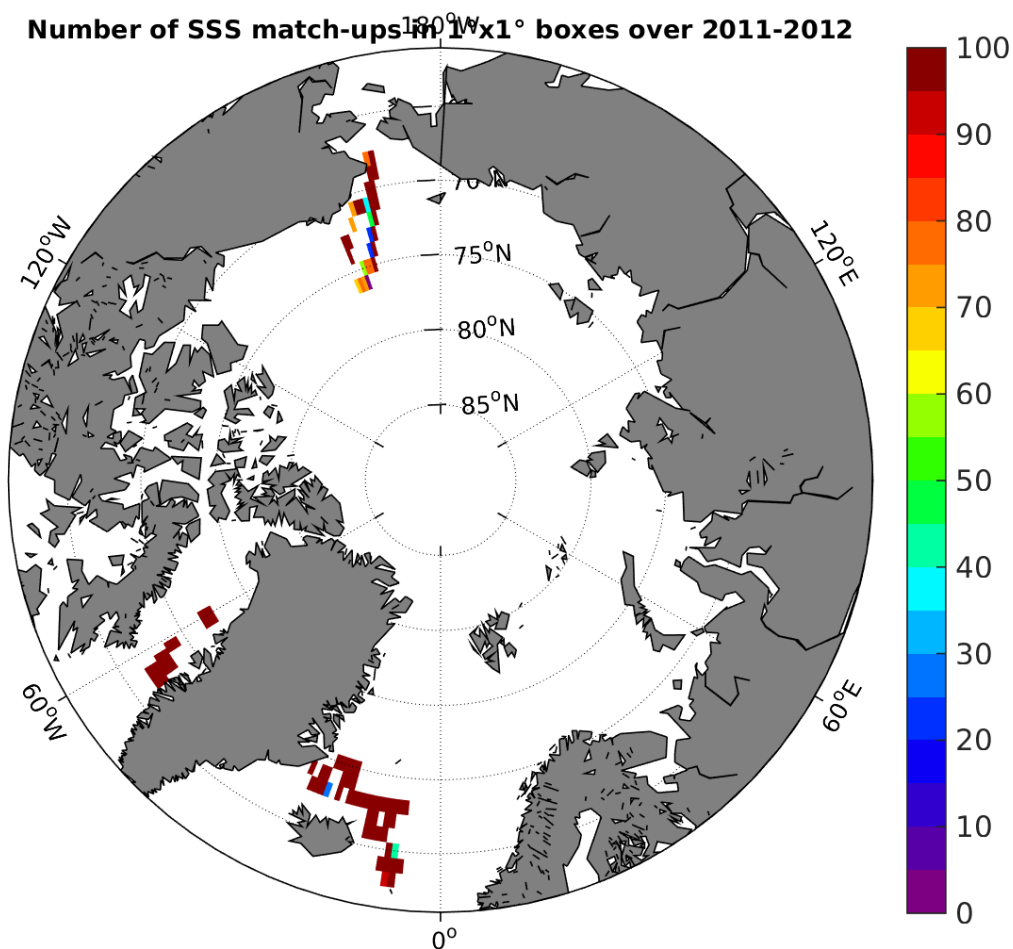
Figure 4: Number of SSS match-ups between TSG-SAMOS SSS and the Aquarius-L3-JPL-V4-7DAY-RUNNING SSS product for the Arctic Ocean Pi-MEP region over 1°x1° boxes and for the full satellite product period.
