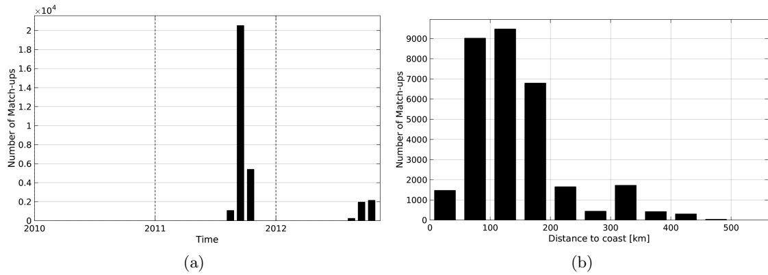
Figure 1: Number of match-ups between TSG-SAMOS and Aquarius-L3-JPL-V4-7DAY-RUNNING SSS as a function of time (a) and as function of the distance to coast (b) over the Arctic Ocean Pi-MEP region and for the full satellite product period.
