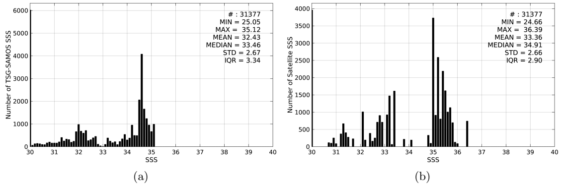
Figure 2: Histograms of SSS from TSG-SAMOS (a) and Aquarius-L3-JPL-V4-7DAY-RUNNING (b) considering all match-up pairs per bins of 0.1 over the Arctic Ocean Pi-MEP region and for the full satellite product period.
