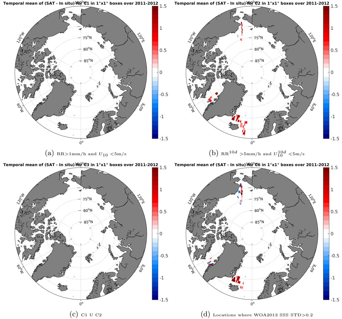
Figure 12: Temporal mean gridded over spatial boxes of size 1^\circ \times 1^\circ of \Delta SSS (Aquarius-L3-JPL-V4-7DAY-RUNNING - TSG-SAMOS) for 4 different subdatasets corresponding to: RR > 1\text{mm/h} and U_{10} < 5\text{m/s} (a), RR^{10d} > 5\text{mm/h} and U_{10}^{10d} < 5\text{m/s} (b), C1 U C2 (c), Locations where WOA2013 SSS STD > 0.2 (d).
