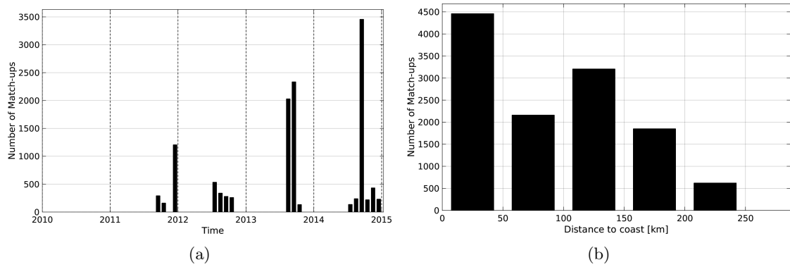
Figure 1: Number of match-ups between TSG-LEGOS-DM and Aquarius-L3-JPL-V4-7DAY-RUNNING SSS as a function of time (a) and as function of the distance to coast (b) over the Arctic Ocean Pi-MEP region and for the full satellite product period.
