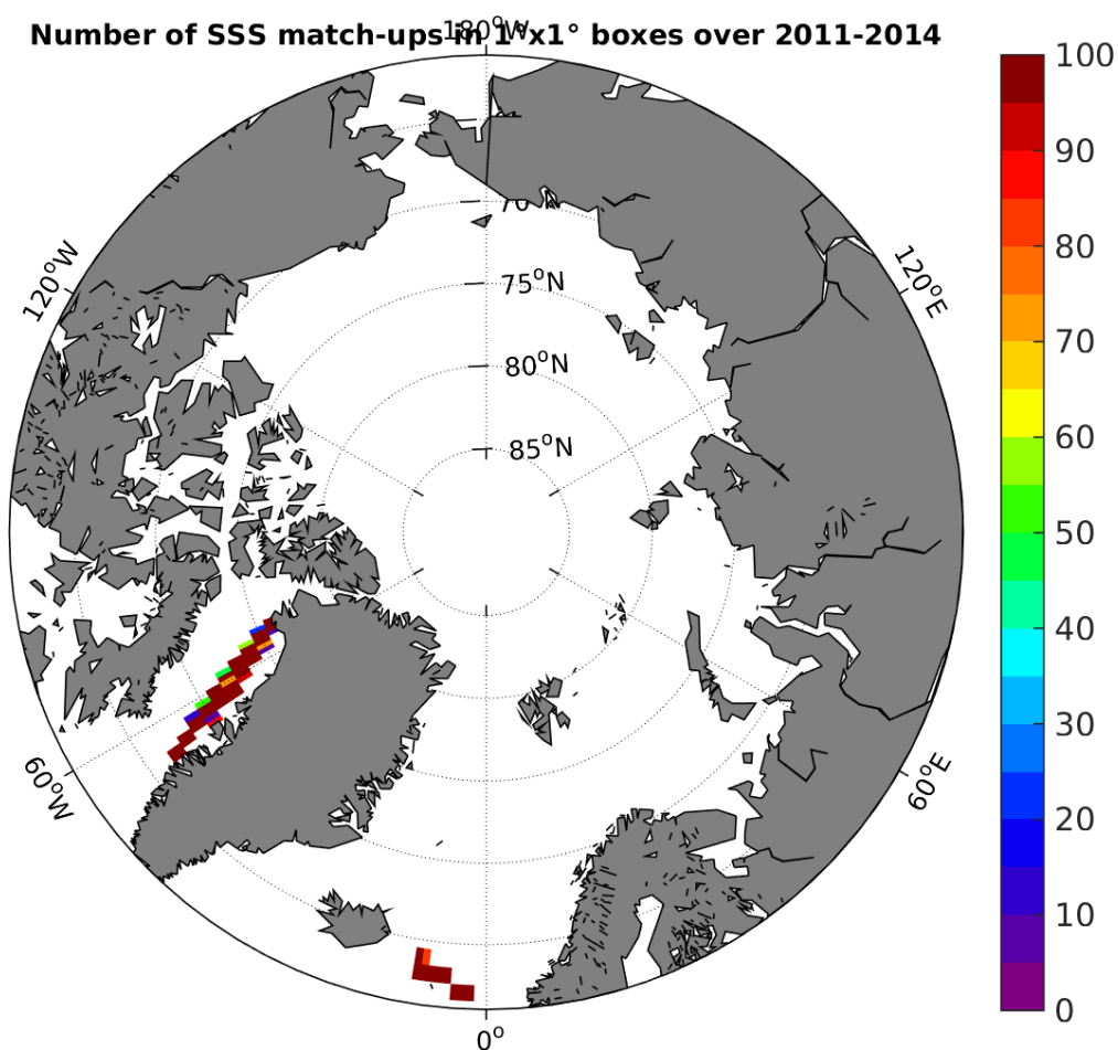
Figure 4: Number of SSS match-ups between TSG-LEGOS-DM SSS and the Aquarius-L3-JPL-V4-7DAY-RUNNING SSS product for the Arctic Ocean Pi-MEP region over 1^\circ \times 1^\circ boxes and for the full satellite product period.
