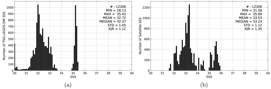
Figure 2: Histograms of SSS from TSG-LEGOS-DM (a) and Aquarius-L3-JPL-V4-7DAY-RUNNING (b) considering all match-up pairs per bins of 0.1 over the Arctic Ocean Pi-MEP region and for the full satellite product period.
