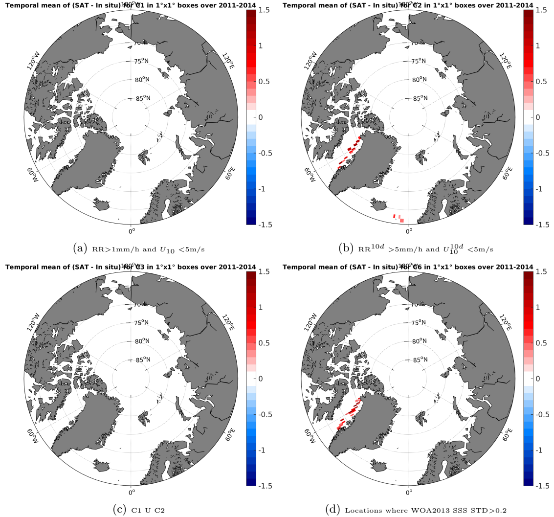
Figure 12: Temporal mean gridded over spatial boxes of size 1^\circ \times 1^\circ of \Delta SSS (Aquarius-L3-JPL-V4-7DAY-RUNNING - TSG-LEGOS-DM) for 4 different subdatasets corresponding to: RR > 1 mm/h and U_{10} < 5 m/s (a), RR 10d > 5 mm/h and U_{10}^{10d} < 5 m/s (b), C1 U C2 (c), Locations where WOA2013 SSS STD > 0.2 (d).
