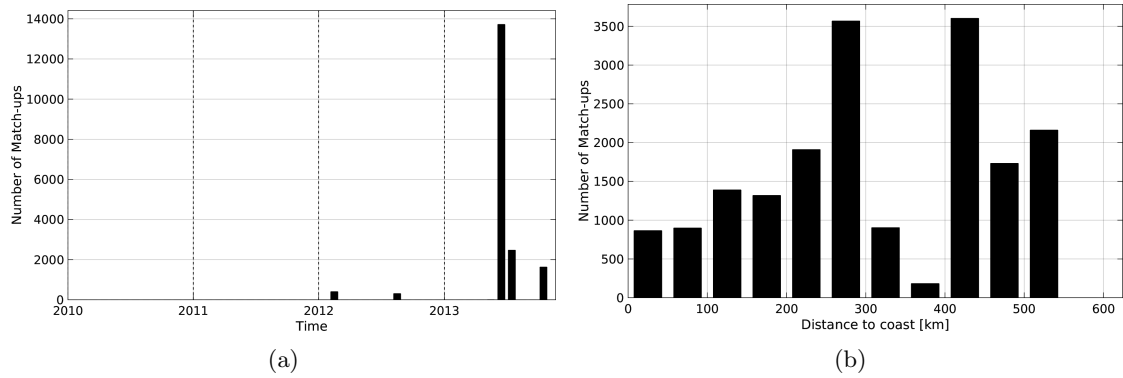
Figure 1: Number of match-ups between TSG-GOSUD-Sailing-ship and Aquarius-L3-JPL-V4-7DAY-RUNNING SSS as a function of time (a) and as function of the distance to coast (b) over the Arctic Ocean Pi-MEP region and for the full satellite product period.
