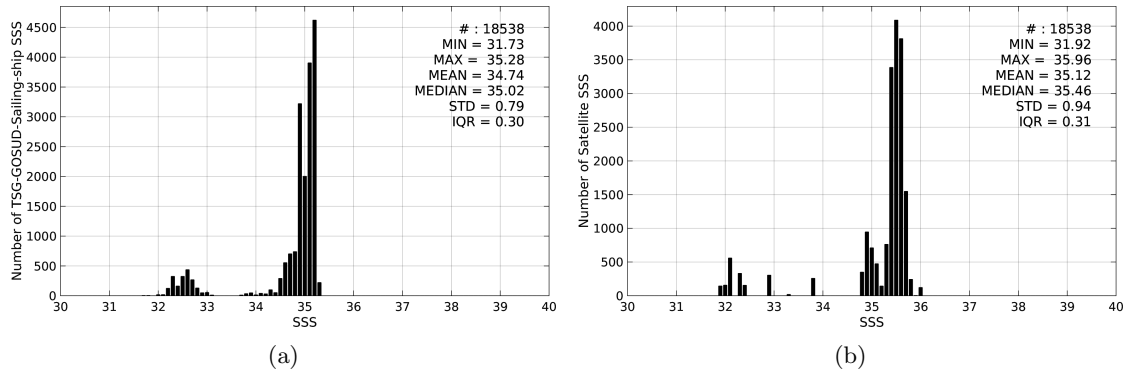
Figure 2: Histograms of SSS from TSG-GOSUD-Sailing-ship (a) and Aquarius-L3-JPL-V4-7DAY-RUNNING (b) considering all match-up pairs per bins of 0.1 over the Arctic Ocean Pi-MEP region and for the full satellite product period.
