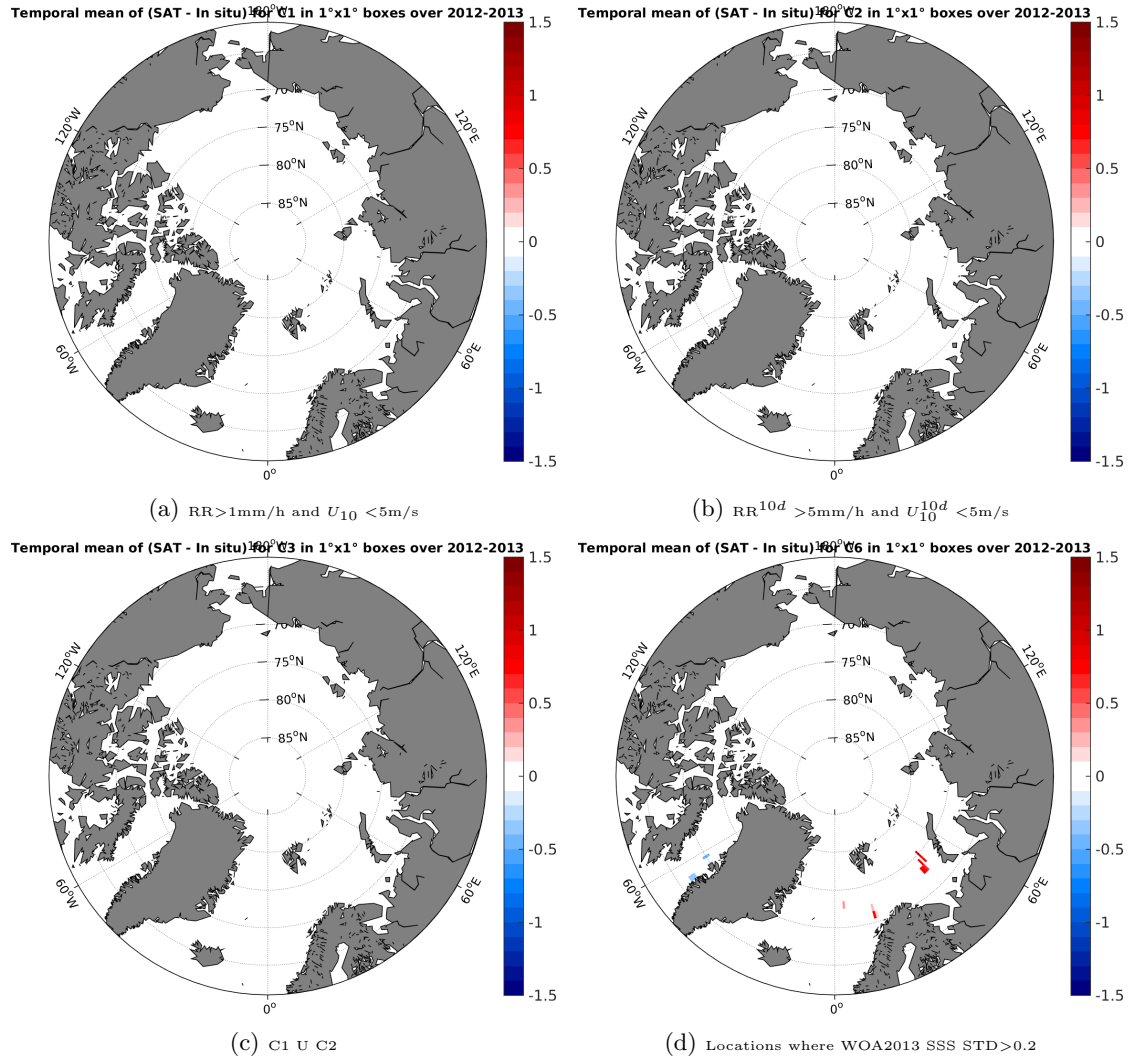
Figure 12: Temporal mean gridded over spatial boxes of size 1^\circ \times 1^\circ of \Delta SSS (Aquarius-L3-JPL-V4-7DAY-RUNNING - TSG-GOSUD-Sailing-ship) for 4 different subdatasets corresponding to: RR > 1mm/h and U_{10} < 5 m/s (a), RR^{10d} > 5 mm/h and U_{10}^{10d} < 5 m/s (b), C1 U C2 (c), Locations where WOA2013 SSS STD > 0.2 (d).
