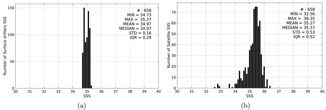
Figure 2: Histograms of SSS from Surface drifters (a) and Aquarius-L3-JPL-V4-7DAY-RUNNING (b) considering all match-up pairs per bins of 0.1 over the Arctic Ocean Pi-MEP region and for the full satellite product period.
