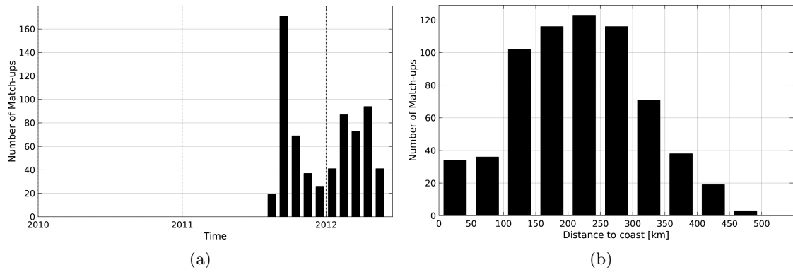
Figure 1: Number of match-ups between Surface drifters and Aquarius-L3-JPL-V4-7DAY-RUNNING SSS as a function of time (a) and as function of the distance to coast (b) over the Arctic Ocean Pi-MEP region and for the full satellite product period.
