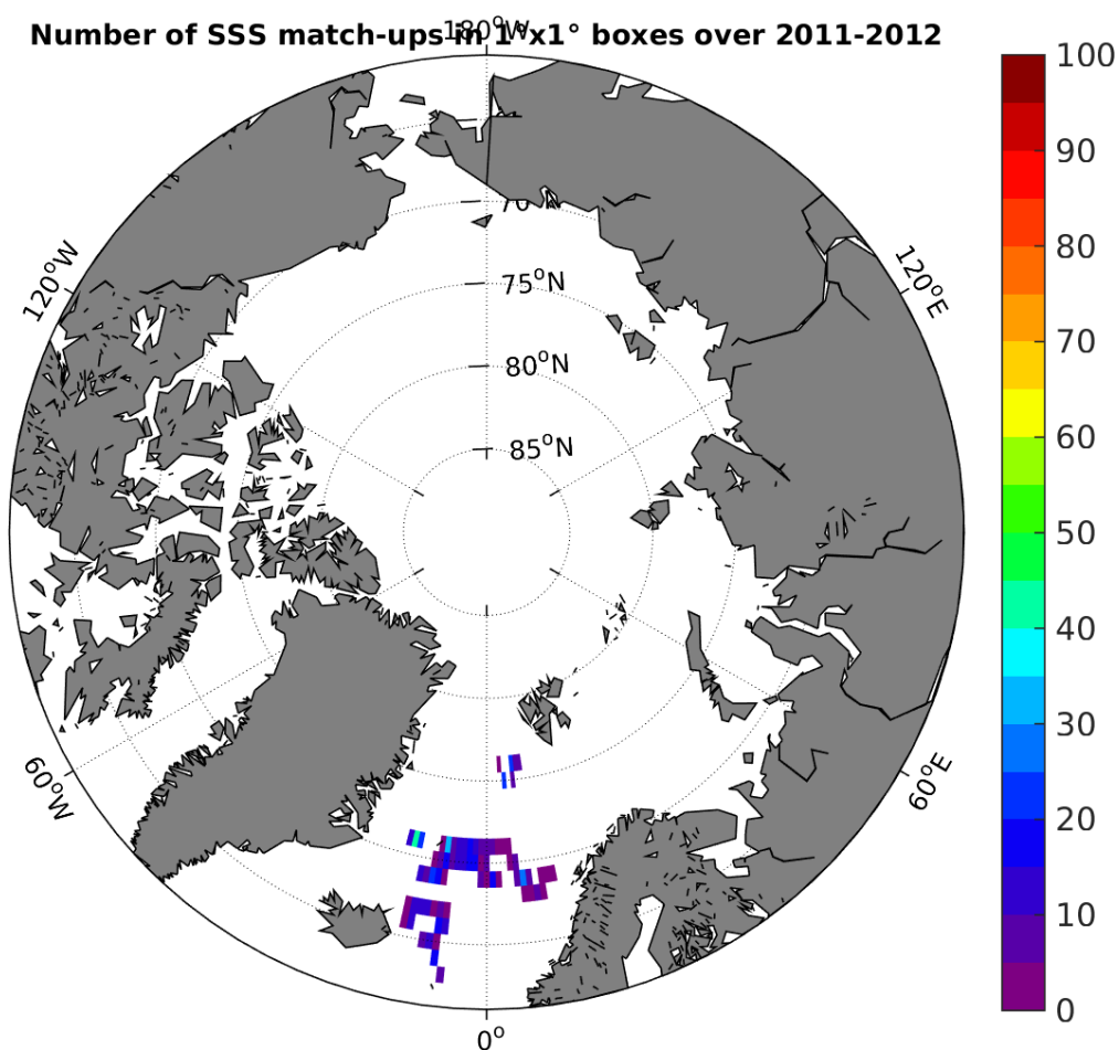
Figure 3: Number of SSS match-ups between Surface drifters SSS and the Aquarius-L3-JPL-V4-7DAY-RUNNING SSS product for the Arctic Ocean Pi-MEP region over 1^\circ \times 1^\circ boxes and for the full satellite product period.
