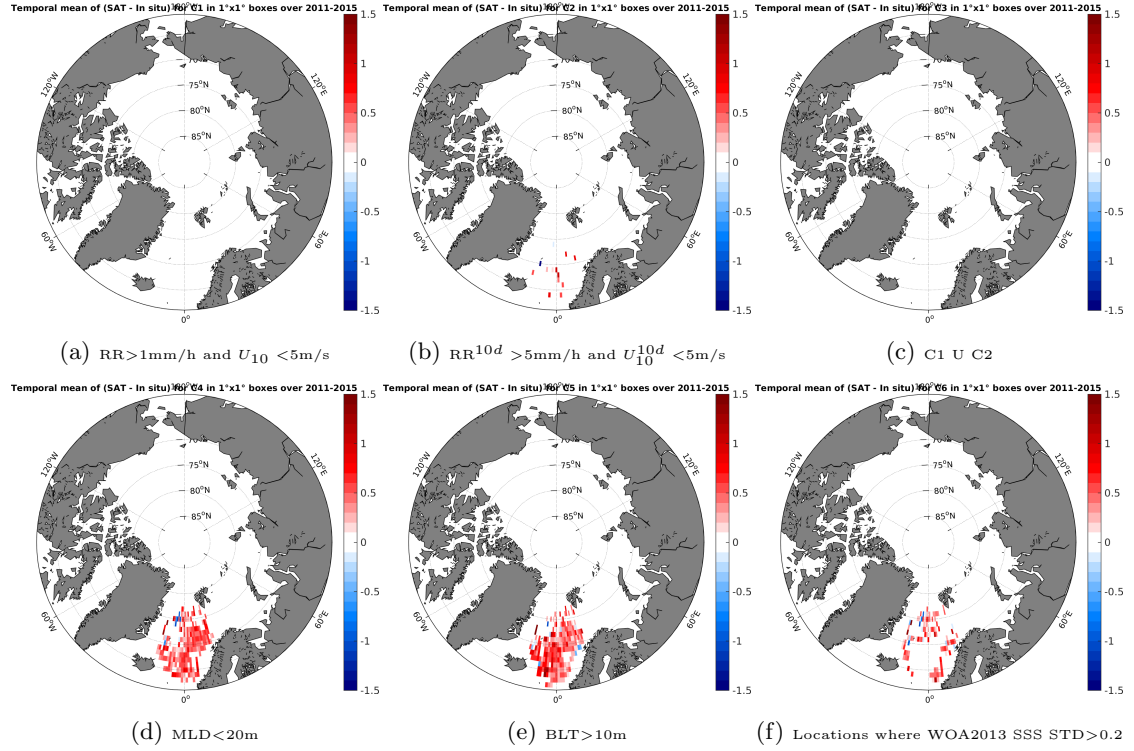
Figure 12: Temporal mean gridded over spatial boxes of size 1^\circ \times 1^\circ of \Delta SSS (Aquarius-L3-JPL-V4-7DAY-RUNNING - Argo) for 6 different subdatasets corresponding to: RR > 1mm/h and U_{10} < 5 m/s (a), RR^{10d} > 5 mm/h and U_{10}^{10d} < 5 m/s (b), C1 U C2 (c), MLD < 20m (d), BLT > 10m (e), Locations where WOA2013 SSS STD > 0.2 (f).
