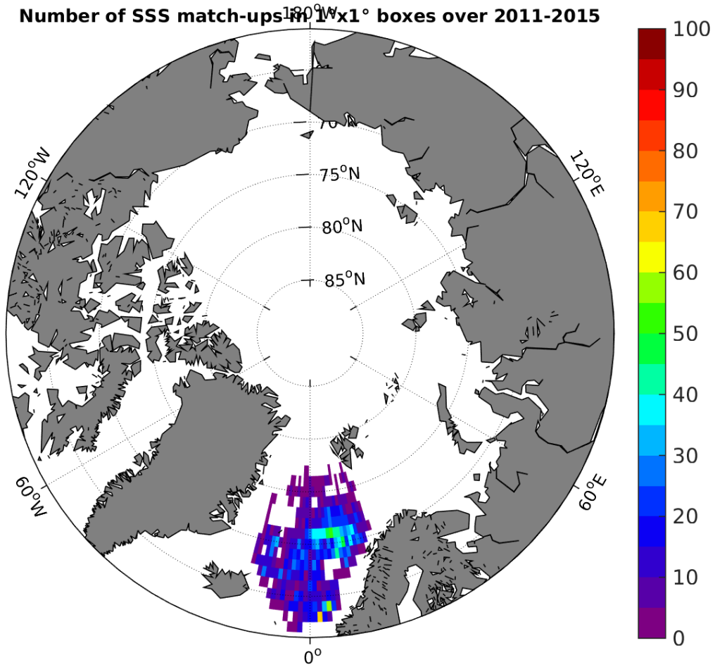
Figure 4: Number of SSS match-ups between Argo SSS and the Aquarius-L3-JPL-V4-7DAY-RUNNING SSS product for the Arctic Ocean Pi-MEP region over 1°x1° boxes and for the full satellite product period.
