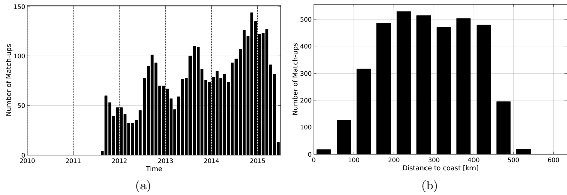
Figure 1: Number of match-ups between Argo and Aquarius-L3-JPL-V4-7DAY-RUNNING SSS as a function of time (a) and as function of the distance to coast (b) over the Arctic Ocean Pi-MEP region and for the full satellite product period.
