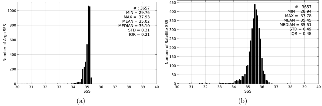
Figure 2: Histograms of SSS from Argo (a) and Aquarius-L3-JPL-V4-7DAY-RUNNING (b) considering all match-up pairs per bins of 0.1 over the Arctic Ocean Pi-MEP region and for the full satellite product period.
