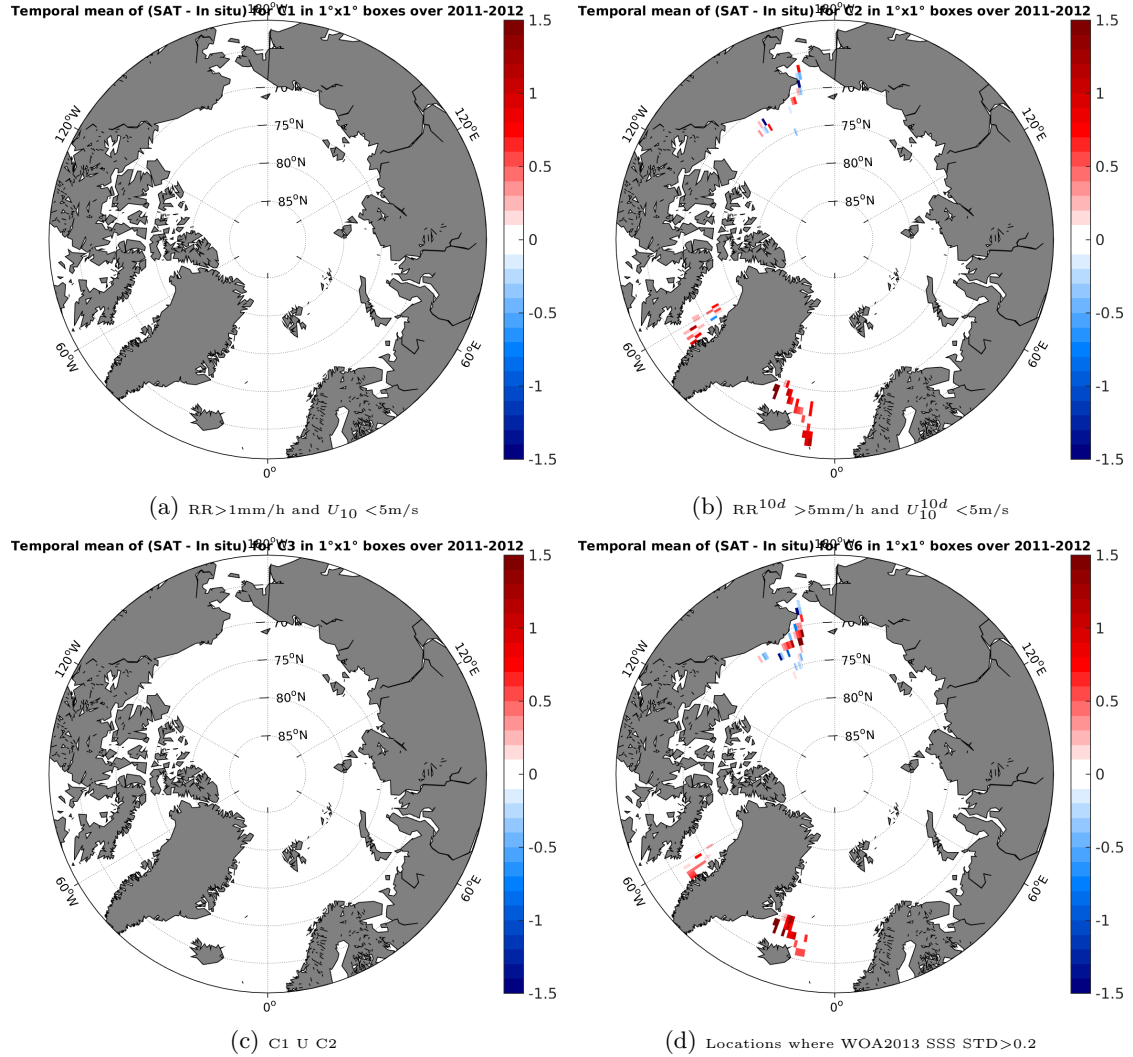
Figure 12: Temporal mean gridded over spatial boxes of size 1^\circ \times 1^\circ of \Delta SSS (Aquarius-L3-JPL-V4-MONTHLY - TSG-SAMOS) for 4 different subdatasets corresponding to: RR > 1\text{mm/h} and U_{10} < 5\text{m/s} (a), RR^{10d} > 5\text{mm/h} and U_{10}^{10d} < 5\text{m/s} (b), C1 U C2 (c), Locations where WOA2013 SSS STD > 0.2 (d).
