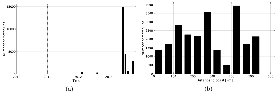
Figure 1: Number of match-ups between TSG-GOSUD-Sailing-ship and Aquarius-L3-JPL-V4-MONTHLY SSS as a function of time (a) and as function of the distance to coast (b) over the Arctic Ocean Pi-MEP region and for the full satellite product period.
