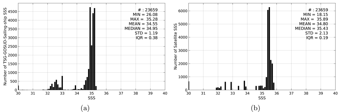
Figure 2: Histograms of SSS from TSG-GOSUD-Sailing-ship (a) and Aquarius-L3-JPL-V4-MONTHLY (b) considering all match-up pairs per bins of 0.1 over the Arctic Ocean Pi-MEP region and for the full satellite product period.
