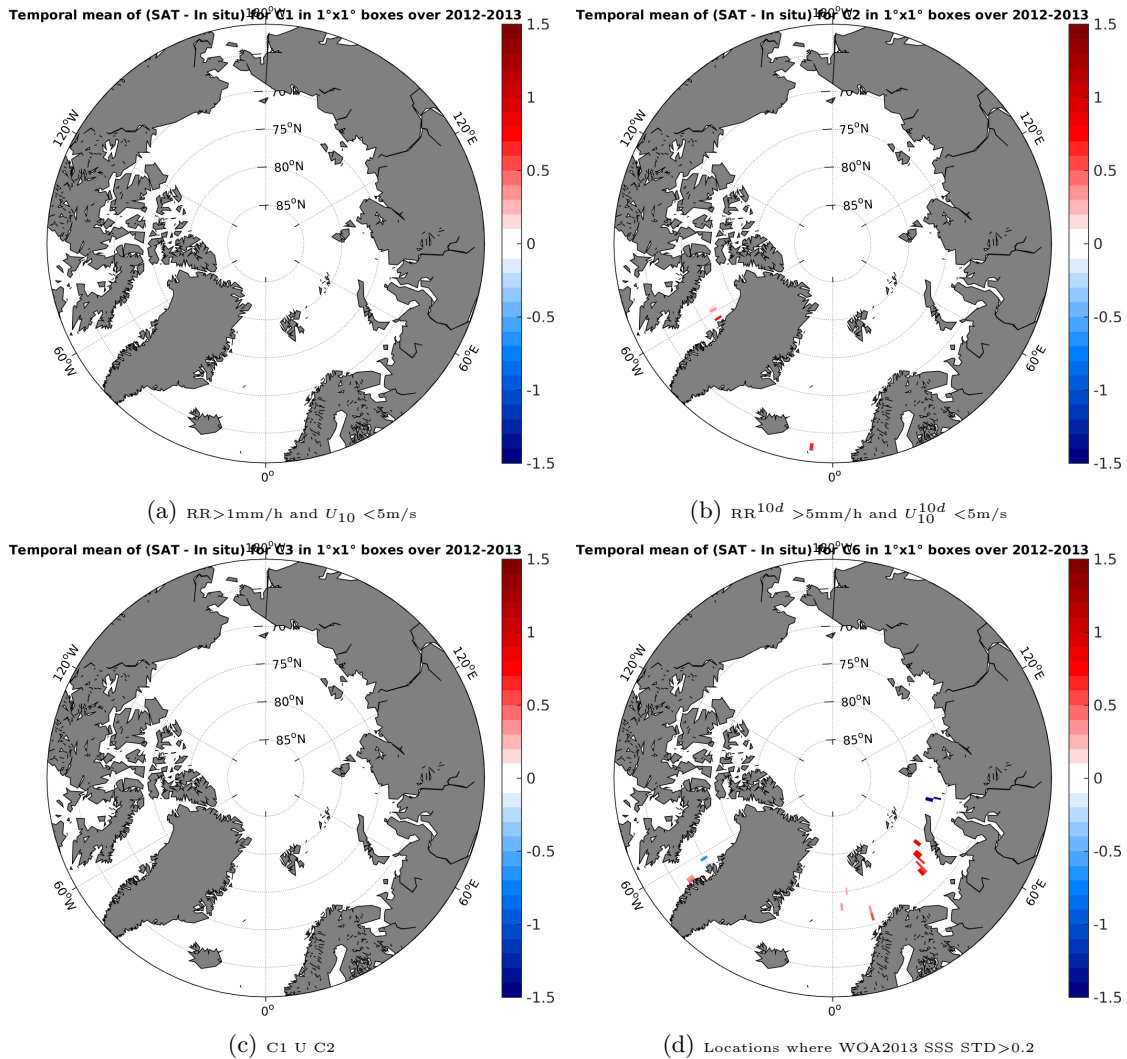
Figure 12: Temporal mean gridded over spatial boxes of size 1^\circ \times 1^\circ of \Delta SSS (Aquarius-L3-JPL-V4-MONTHLY - TSG-GOSUD-Sailing-ship) for 4 different subdatasets corresponding to: RR > 1 mm/h and U_{10} < 5 m/s (a), RR^{10d} > 5 mm/h and U_{10}^{10d} < 5 m/s (b), C1 U C2 (c), Locations where WOA2013 SSS STD > 0.2 (d).
