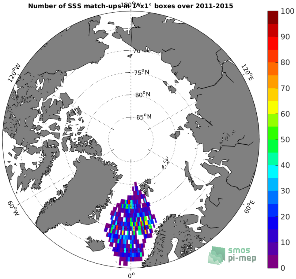
Figure 4: Number of SSS match-ups between Argo SSS and the Aquarius SSS L2-AVERAGED OR v5 (NASA-GSFC) SSS product for the Arctic Ocean Pi-MEP region over 1^\circ \times 1^\circ boxes and for the full satellite product period.
