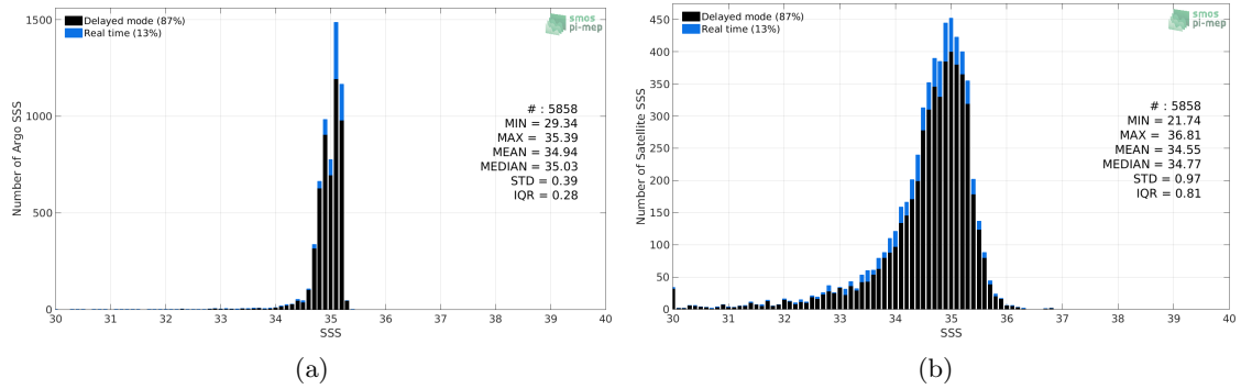
Figure 2: Histograms of SSS from Argo (a) and Aquarius SSS L2-AVERAGED OR v5 (NASA-GSFC) (b) considering all match-up pairs per bins of 0.1 over the Arctic Ocean Pi-MEP region and for the full satellite product period.
