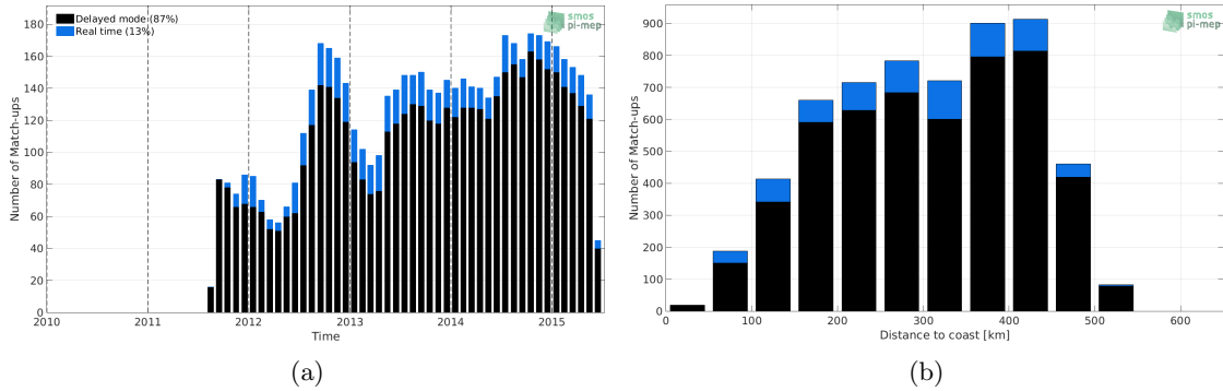
Figure 1: Number of match-ups between Argo and Aquarius SSS L2-AVERAGED OR v5 (NASA-GSFC) SSS as a function of time (a) and as function of the distance to coast (b) over the Arctic Ocean Pi-MEP region and for the full satellite product period.
