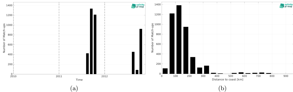
Figure 2: Number of match-ups between TSG (SAMOS) and Aquarius SSS L2 OR v5 (NASA-GSFC) SSS as a function of time (a) and as function of the distance to coast (b) over the Arctic Ocean Pi-MEP region and for the full satellite product period.
