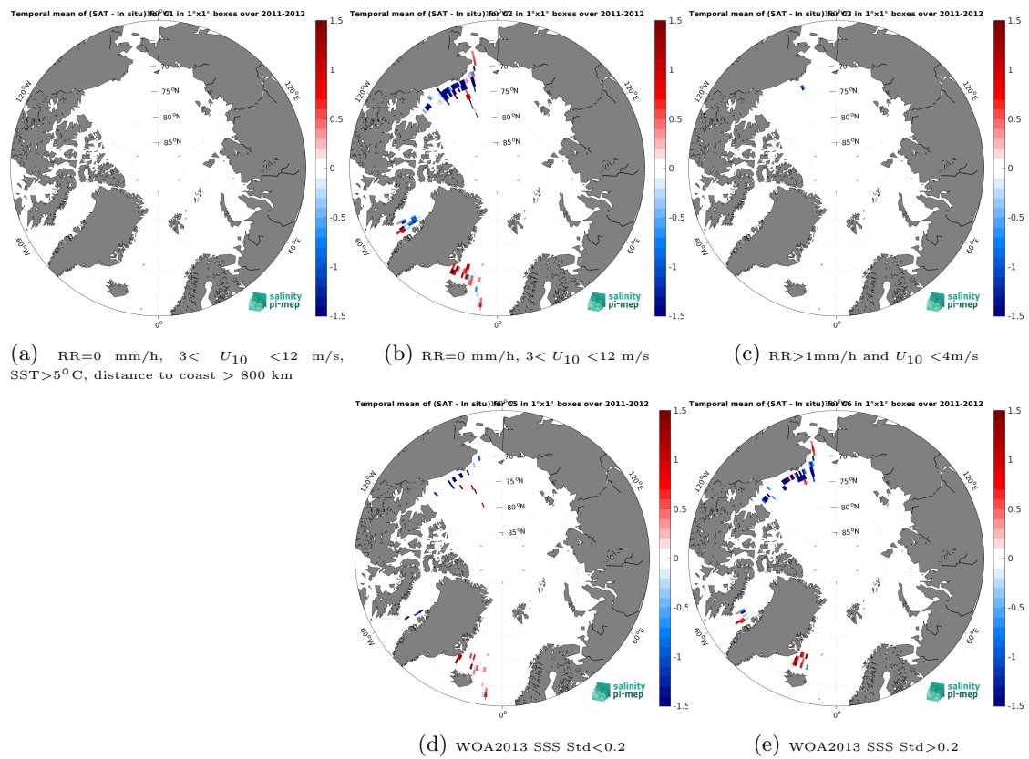
Figure 14: Temporal mean gridded over spatial boxes of size 1^\circ \times 1^\circ of \Delta\text{SSS} (Aquarius SSS L2 OR v5 (NASA-GSFC) - TSG (SAMOS)) for 5 different subdatasets corresponding to:RR=0 mm/h, 3 < U_{10} < 12 m/s, SST > 5°C, distance to coast > 800 km (a), RR=0 mm/h, 3 < U_{10} < 12 m/s (b), RR > 1mm/h and U_{10} < 4 m/s (c), WOA2013 SSS Std < 0.2 (d), WOA2013 SSS Std > 0.2 (e).
