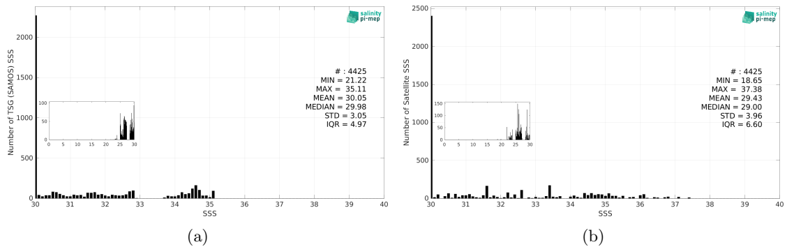
Figure 3: Histograms of SSS from TSG (SAMOS) (a) and Aquarius SSS L2 OR v5 (NASA-GSFC) (b) considering all match-up pairs per bins of 0.1 over the Arctic Ocean Pi-MEP region and for the full satellite product period.
