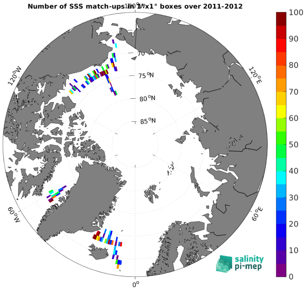
Figure 5: Number of SSS match-ups between TSG (SAMOS) SSS and the Aquarius SSS L2 OR v5 (NASA-GSFC) SSS product for the Arctic Ocean Pi-MEP region over 1^\circ \times 1^\circ boxes and for the full satellite product period.
