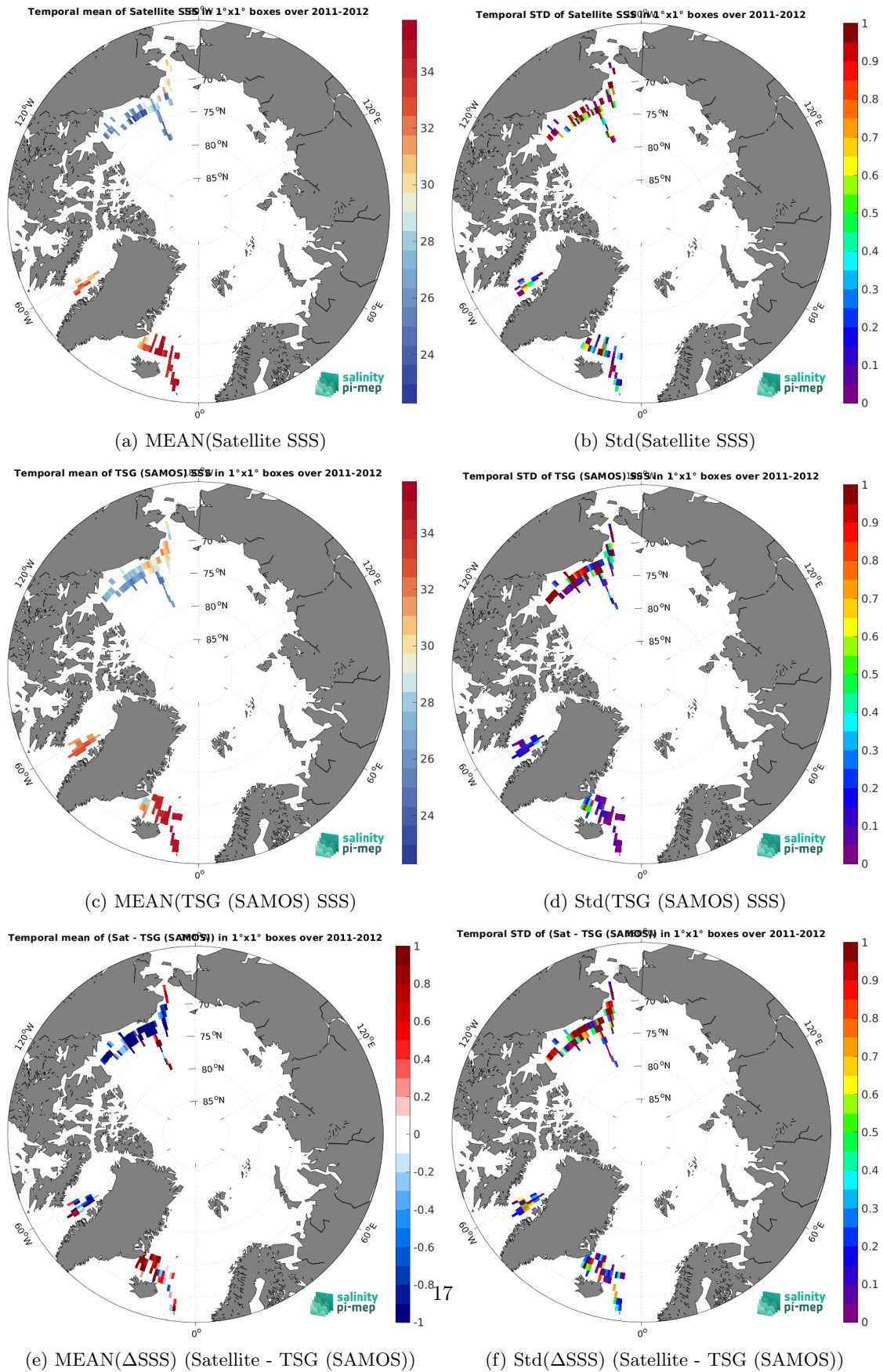
Figure 7: Temporal mean (left) and Std (right) of SSS from Aquarius SSS L2 OR v5 (NASA-GSFC) (top), TSG (SAMOS) (middle), and of \Delta SSS (Satellite - TSG (SAMOS)). Only match-up pairs are used to generate these maps.
