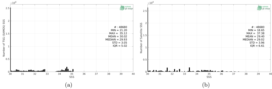
Figure 2: Histograms of SSS from TSG (SAMOS) (a) and Aquarius SSS L2 OR v5 (NASA-GSFC) (b) considering all match-up pairs per bins of 0.1 over the Arctic Ocean Pi-MEP region and for the full satellite product period.
