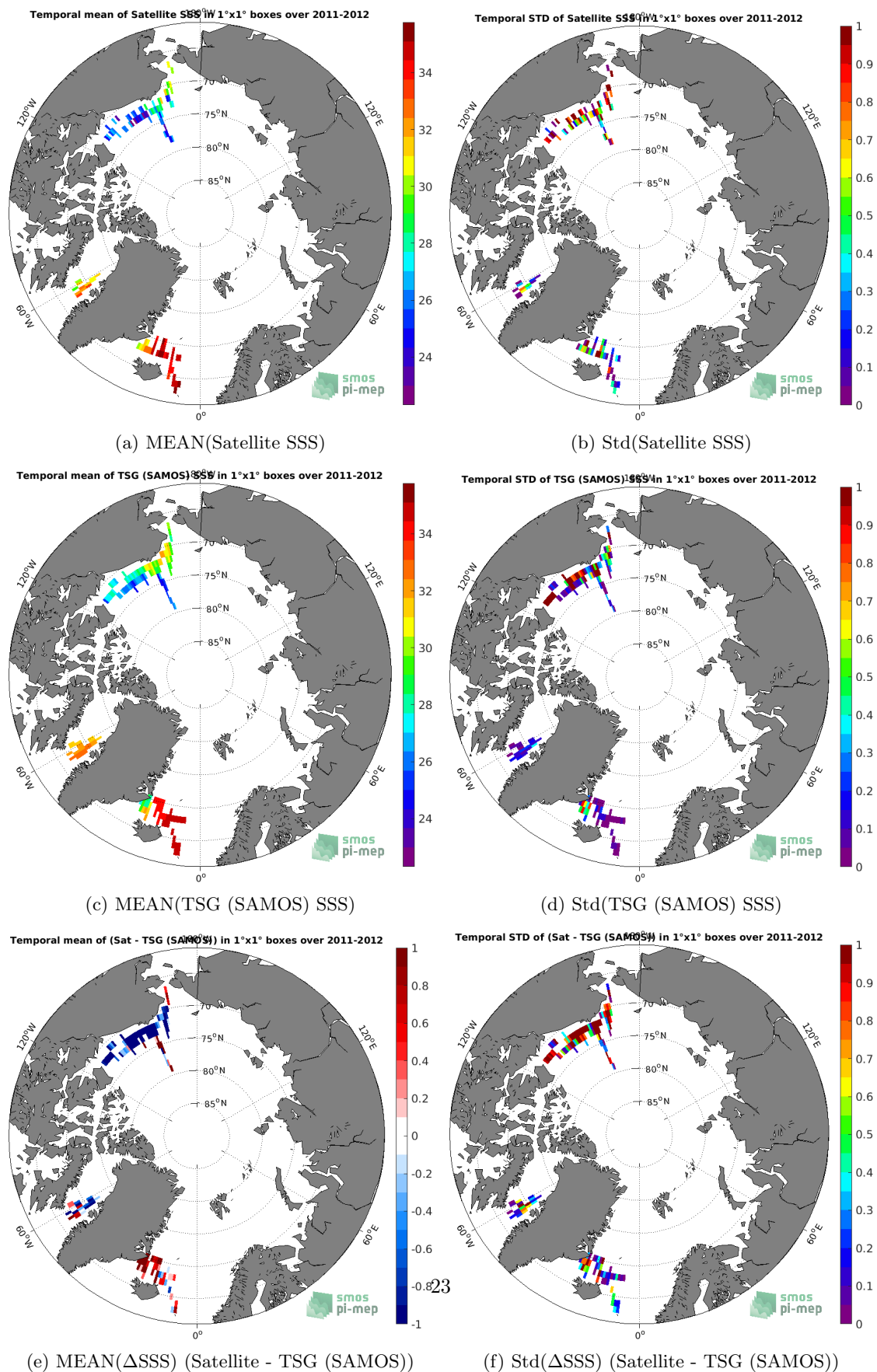
Figure 6: Temporal mean (left) and Std (right) of SSS from Aquarius SSS L2 OR v5 (NASA-GSFC) (top), TSG (SAMOS) (middle), and of \Delta SSS (Satellite - TSG (SAMOS)). Only match-up pairs are used to generate these maps.
