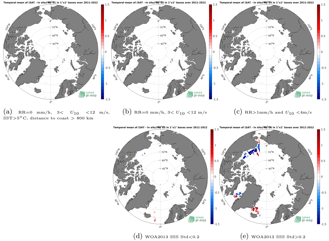
Figure 12: Temporal mean gridded over spatial boxes of size 1^{\circ}\times 1^{\circ} of \Delta\text{SSS} (Aquarius SSS L2 OR v5 (NASA-GSFC) - TSG (SAMOS)) for 5 different subdatasets corresponding to: RR=0 mm/h, 3 < U_{10} < 12 m/s, SST >5^{\circ}\text{C} , distance to coast > 800 km (a), RR=0 mm/h, 3 < U_{10} < 12 m/s (b), RR >1 mm/h and U_{10} < 4 m/s (c), WOA2013 SSS Std <0.2 (d), WOA2013 SSS Std >0.2 (e).
