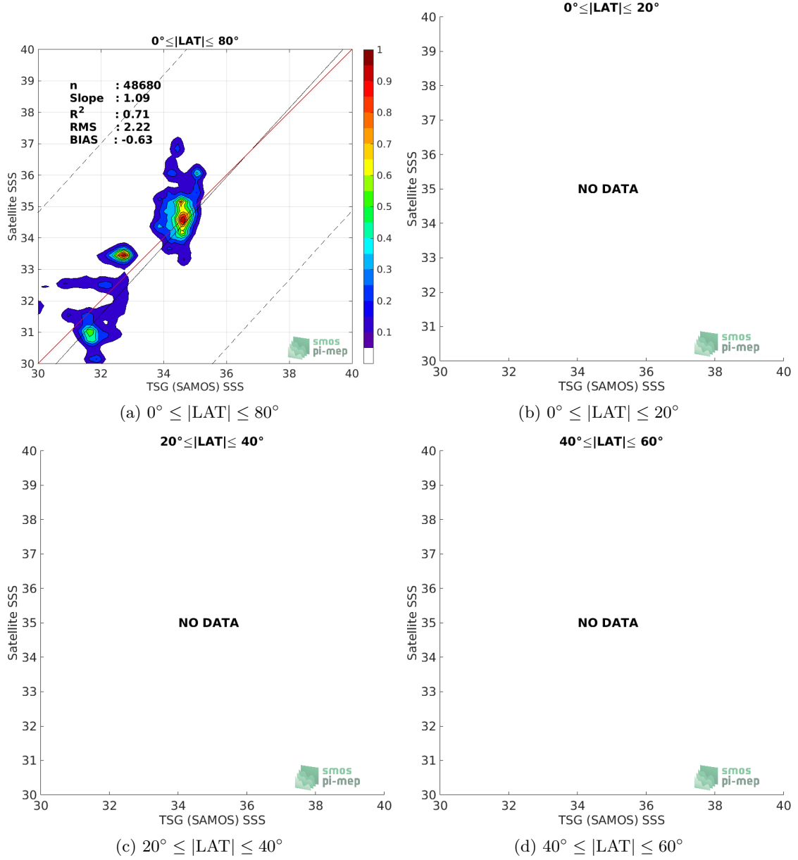
Figure 9: Contour maps of the concentration of Aquarius SSS L2 OR v5 (NASA-GSFC) SSS (y-axis) versus TSG (SAMOS) SSS (x-axis) at match-up pairs for different latitude bands. For each plot, the red line shows x=y . The black thin and dashed lines indicate a linear fit through the data cloud and the \pm 95\% confidence levels, respectively. The number match-up pairs n , the slope and R^2 coefficient of the linear fit, the root mean square (RMS) and the mean bias between satellite and in situ data are indicated for each latitude band in each plots.
