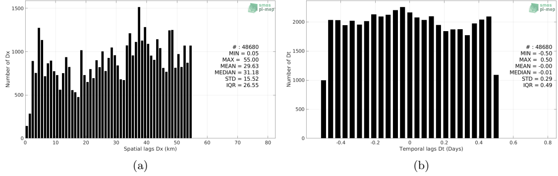
Figure 5: Histograms of the spatial (a) and temporal (b) lags between the location/time of the TSG (SAMOS) measurement and the date of the corresponding Aquarius SSS L2 OR v5 (NASA-GSFC) SSS pixel.
