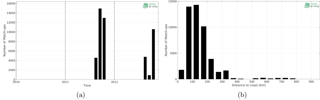
Figure 1: Number of match-ups between TSG (SAMOS) and Aquarius SSS L2 OR v5 (NASA-GSFC) SSS as a function of time (a) and as function of the distance to coast (b) over the Arctic Ocean Pi-MEP region and for the full satellite product period.
