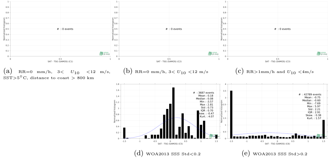
Figure 13: Normalized histogram of \Delta\text{SSS} (Aquarius SSS L2 OR v5 (NASA-GSFC) - TSG (SAMOS)) for 5 different subdatasets corresponding to: RR=0 mm/h, 3 < U_{10} < 12 m/s, SST > 5^\circ\text{C} , distance to coast > 800 km (a), RR=0 mm/h, 3 < U_{10} < 12 m/s (b), RR > 1 mm/h and U_{10} < 4 m/s (c), WOA2013 SSS Std < 0.2 (d), WOA2013 SSS Std > 0.2 (e).
