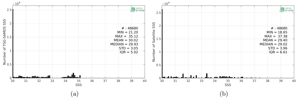
Figure 2: Histograms of SSS from TSG-SAMOS (a) and Aquarius-L2-OR-V5 (b) considering all match-up pairs per bins of 0.1 over the Arctic Ocean Pi-MEP region and for the full satellite product period.
