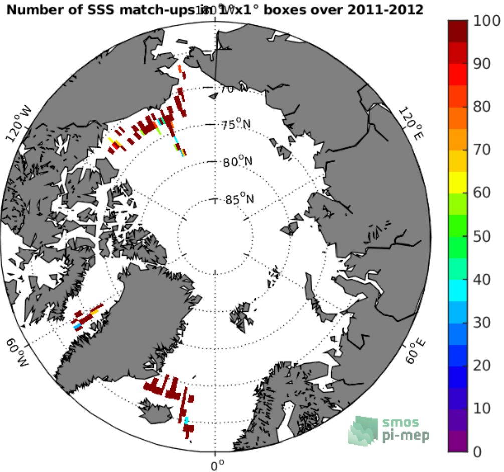
Figure 4: Number of SSS match-ups between TSG-SAMOS SSS and the Aquarius-L2-OR-V5 SSS product for the Arctic Ocean Pi-MEP region over 1°x1° boxes and for the full satellite product period.
