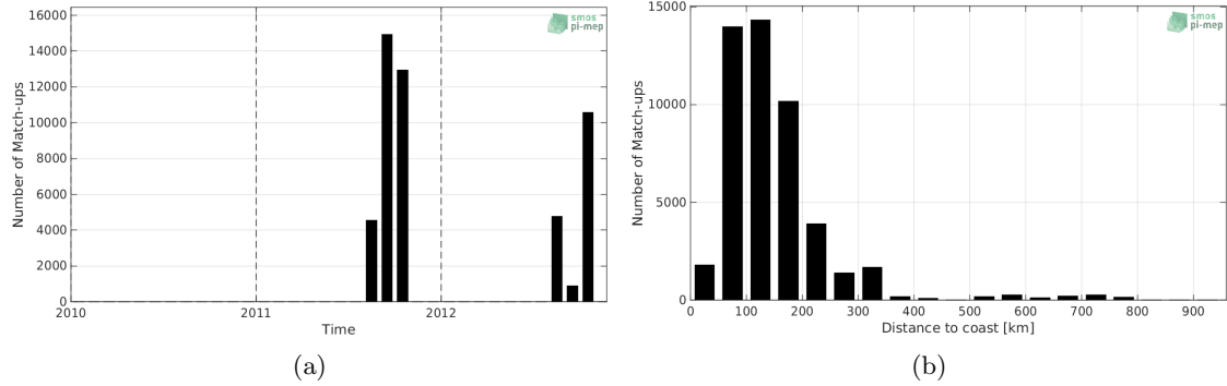
Figure 1: Number of match-ups between TSG-SAMOS and Aquarius-L2-OR-V5 SSS as a function of time (a) and as function of the distance to coast (b) over the Arctic Ocean Pi-MEP region and for the full satellite product period.
