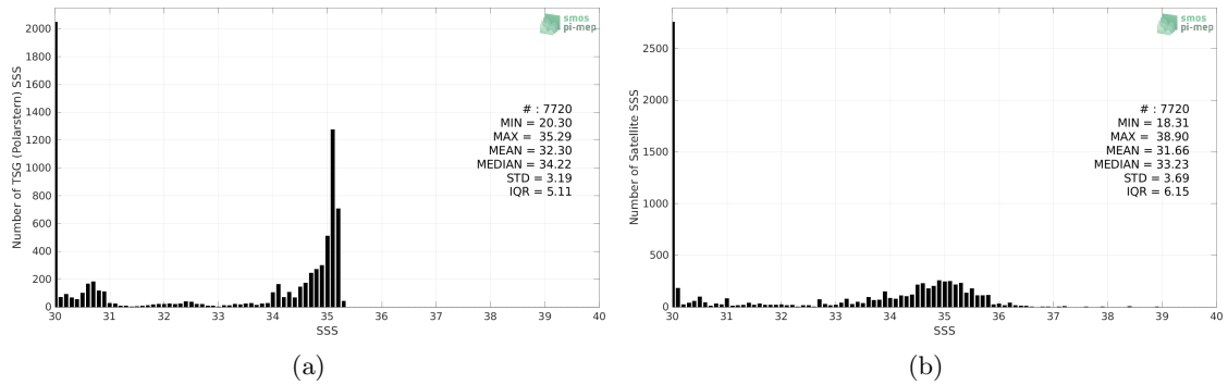
Figure 2: Histograms of SSS from TSG (Polarstern) (a) and Aquarius SSS L2 OR v5 (NASA-GSFC) (b) considering all match-up pairs per bins of 0.1 over the Arctic Ocean Pi-MEP region and for the full satellite product period.
