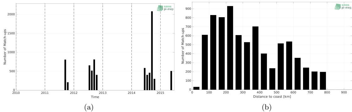
Figure 1: Number of match-ups between TSG (Polarstern) and Aquarius SSS L2 OR v5 (NASA-GSFC) SSS as a function of time (a) and as function of the distance to coast (b) over the Arctic Ocean Pi-MEP region and for the full satellite product period.
