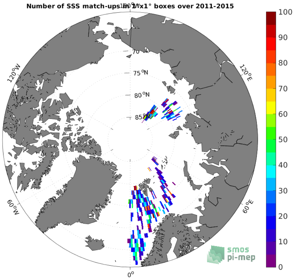
Figure 4: Number of SSS match-ups between TSG (Polarstern) SSS and the Aquarius SSS L2 OR v5 (NASA-GSFC) SSS product for the Arctic Ocean Pi-MEP region over 1^\circ \times 1^\circ boxes and for the full satellite product period.
