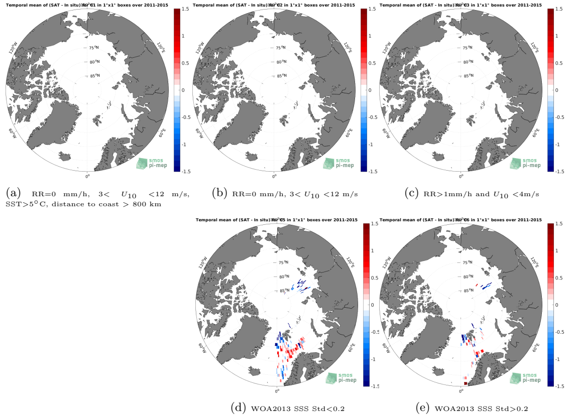
Figure 12: Temporal mean gridded over spatial boxes of size 1^{\circ}\times 1^{\circ} of \Delta\text{SSS} (Aquarius SSS L2 OR v5 (NASA-GSFC) - TSG (Polarstern)) for 5 different subdatasets corresponding to:RR=0 mm/h, 3 < U_{10} < 12 m/s, SST > 5^{\circ}\text{C} , distance to coast > 800 km (a), RR=0 mm/h, 3 < U_{10} < 12 m/s (b), RR > 1 mm/h and U_{10} < 4 m/s (c), WOA2013 SSS Std < 0.2 (d), WOA2013 SSS Std > 0.2 (e).
