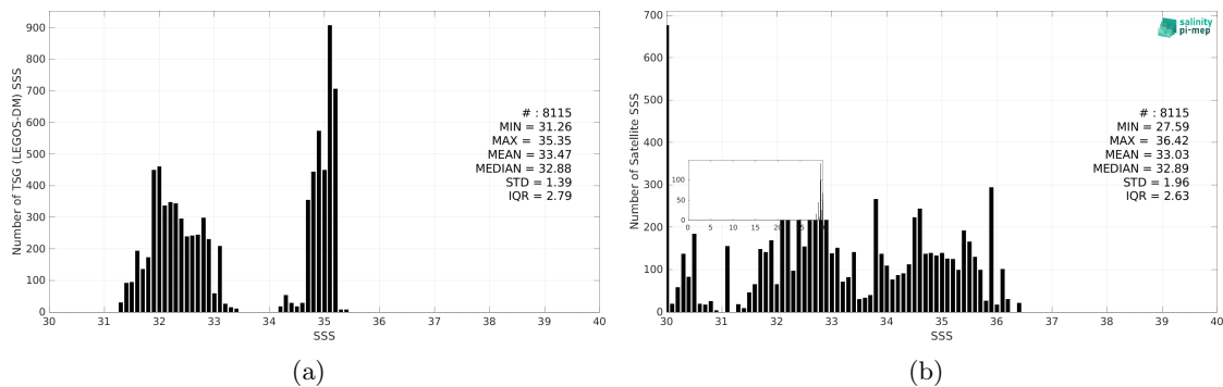
Figure 3: Histograms of SSS from TSG (LEGOS-DM) (a) and Aquarius SSS L2 OR v5 (NASA-GSFC) (b) considering all match-up pairs per bins of 0.1 over the Arctic Ocean Pi-MEP region and for the full satellite product period.
