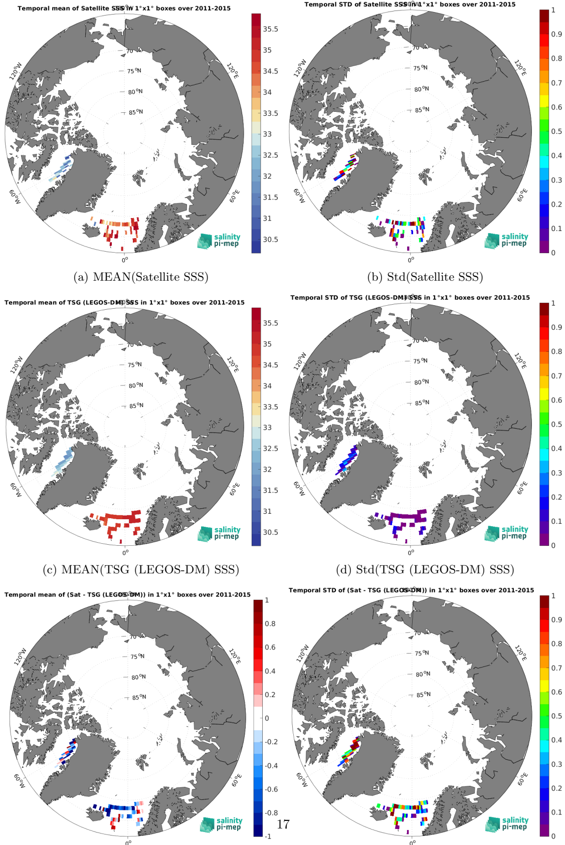
(e) MEAN( \Delta SSS) (Satellite - TSG (LEGOS-DM)) (f) Std( \Delta SSS) (Satellite - TSG (LEGOS-DM)) Figure 7: Temporal mean (left) and Std (right) of SSS from Aquarius SSS L2 OR v5 (NASA-GSFC) (top), TSG (LEGOS-DM) (middle), and of \Delta SSS (Satellite - TSG (LEGOS-DM)). Only match-up pairs are used to generate these maps.
