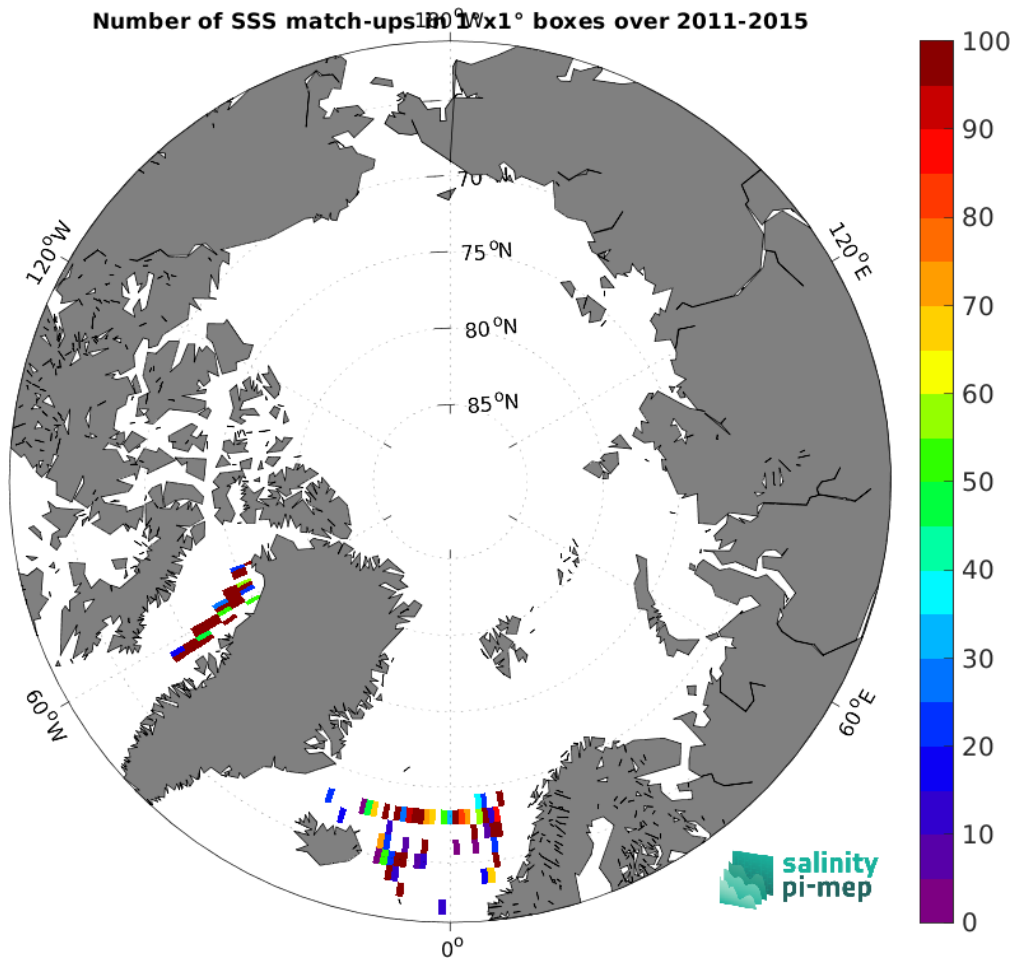
Figure 5: Number of SSS match-ups between TSG (LEGOS-DM) SSS and the Aquarius SSS L2 OR v5 (NASA-GSFC) SSS product for the Arctic Ocean Pi-MEP region over 1^\circ \times 1^\circ boxes and for the full satellite product period.
