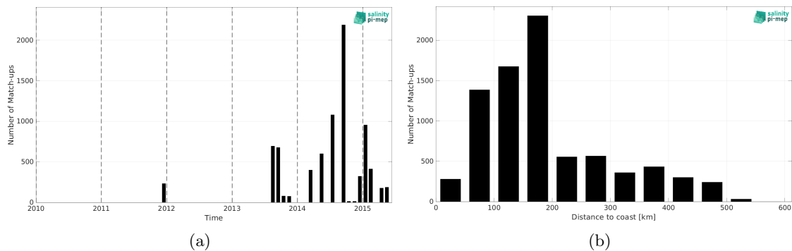
Figure 2: Number of match-ups between TSG (LEGOS-DM) and Aquarius SSS L2 OR v5 (NASA-GSFC) SSS as a function of time (a) and as function of the distance to coast (b) over the Arctic Ocean Pi-MEP region and for the full satellite product period.
