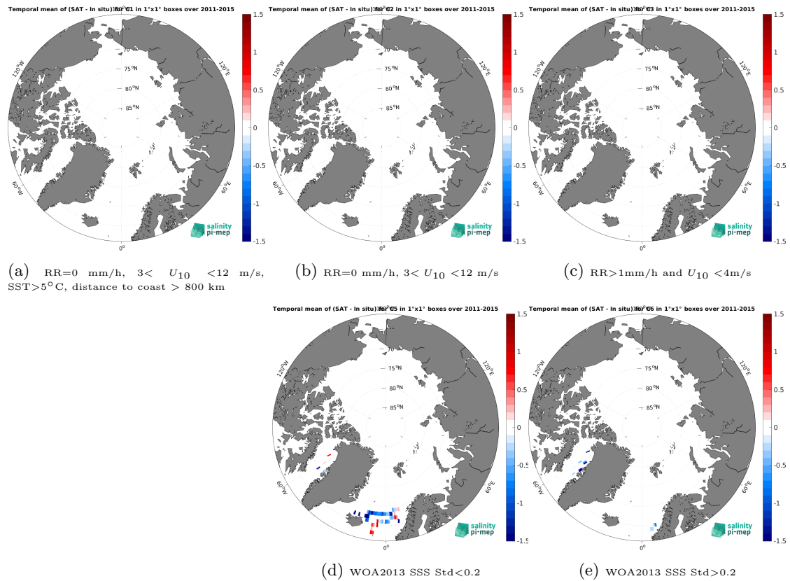
Figure 12: Temporal mean gridded over spatial boxes of size 1^{\circ}\times 1^{\circ} of \Delta\text{SSS} (Aquarius SSS L2 OR v5 (NASA-GSFC) - TSG (LEGOS-DM)) for 5 different subdatasets corresponding to:RR=0 mm/h, 3 < U_{10} < 12 m/s, SST > 5^{\circ}\text{C} , distance to coast > 800 km (a), RR=0 mm/h, 3 < U_{10} < 12 m/s (b), RR > 1 mm/h and U_{10} < 4 m/s (c), WOA2013 SSS Std < 0.2 (d), WOA2013 SSS Std > 0.2 (e).
