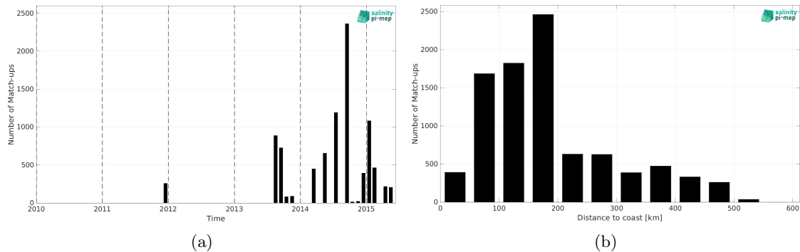
Figure 1: Number of match-ups between TSG (LEGOS-DM) and Aquarius SSS L2 OR v5 (NASA-GSFC) SSS as a function of time (a) and as function of the distance to coast (b) over the Arctic Ocean Pi-MEP region and for the full satellite product period.
