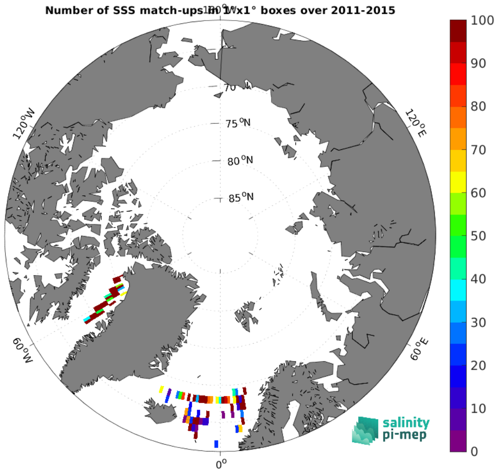
Figure 4: Number of SSS match-ups between TSG (LEGOS-DM) SSS and the Aquarius SSS L2 OR v5 (NASA-GSFC) SSS product for the Arctic Ocean Pi-MEP region over 1^\circ \times 1^\circ boxes and for the full satellite product period.
