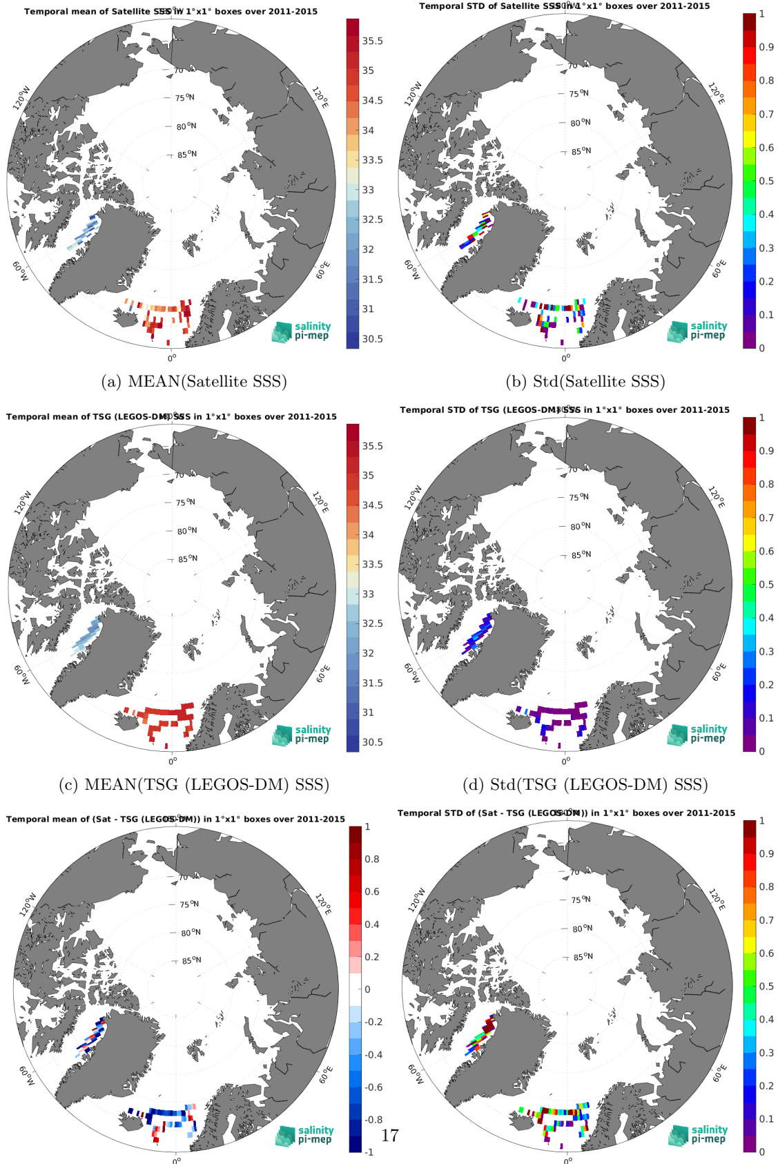
Figure 6: Temporal mean (left) and Std (right) of SSS from Aquarius SSS L2 OR v5 (NASA-GSFC) (top), TSG (LEGOS-DM) (middle), and of \Delta SSS (Satellite - TSG (LEGOS-DM)). Only match-up pairs are used to generate these maps.
