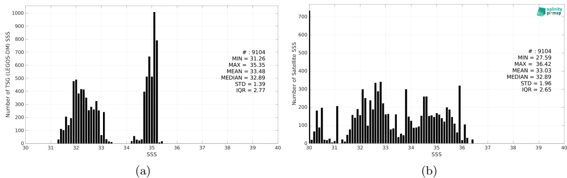
Figure 2: Histograms of SSS from TSG (LEGOS-DM) (a) and Aquarius SSS L2 OR v5 (NASA-GSFC) (b) considering all match-up pairs per bins of 0.1 over the Arctic Ocean Pi-MEP region and for the full satellite product period.
