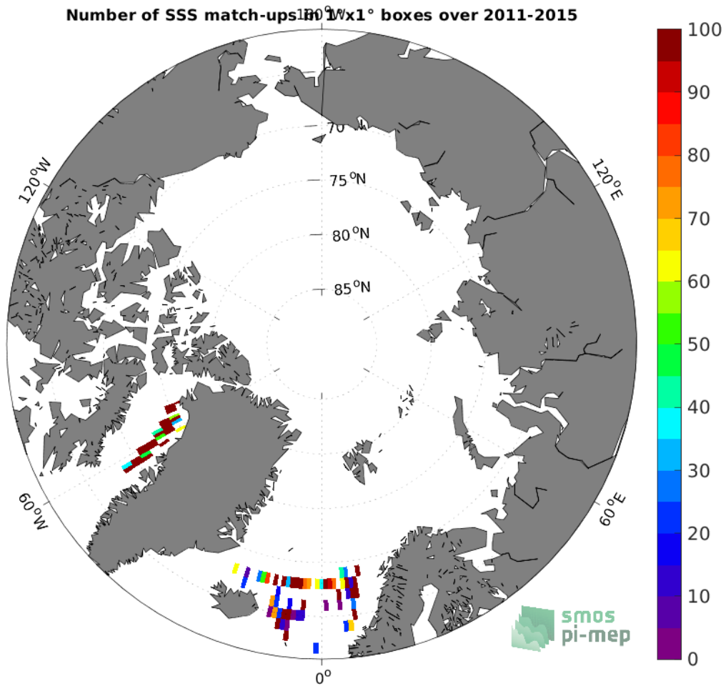
Figure 4: Number of SSS match-ups between TSG (LEGOS-DM) SSS and the Aquarius SSS L2 OR v5 (NASA-GSFC) SSS product for the Arctic Ocean Pi-MEP region over 1^{\circ} \times 1^{\circ} boxes and for the full satellite product period.
