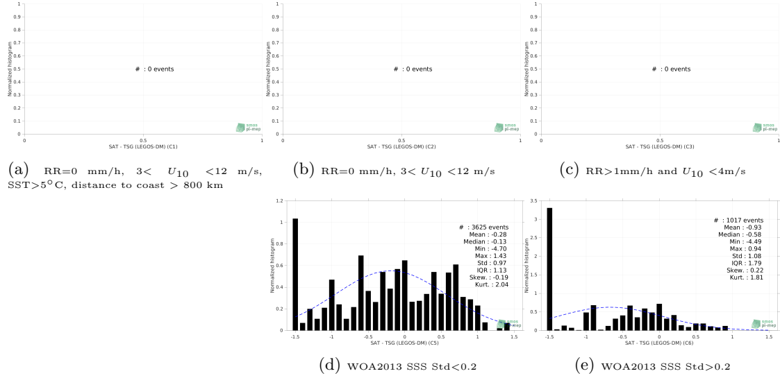
Figure 13: Normalized histogram of \Delta SSS (Aquarius SSS L2 OR v5 (NASA-GSFC) - TSG (LEGOS-DM)) for 5 different subdatasets corresponding to: RR=0 mm/h, 3 < U_{10} < 12 m/s, SST >5^{\circ} C, distance to coast > 800 km (a), RR=0 mm/h, 3 < U_{10} < 12 m/s (b), RR >1 mm/h and U_{10} < 4 m/s (c), WOA2013 SSS Std <0.2 (d), WOA2013 SSS Std >0.2 (e).
