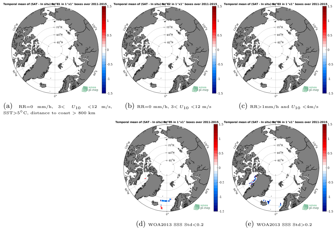
Figure 12: Temporal mean gridded over spatial boxes of size 1^\circ \times 1^\circ of \Delta SSS (Aquarius-L2-OR-V5 - TSG-LEGOS-DM) for 5 different subdatasets corresponding to:RR=0 mm/h, 3 < U_{10} < 12 m/s, SST > 5^\circ\text{C} , distance to coast > 800 km (a), RR=0 mm/h, 3 < U_{10} < 12 m/s (b), RR > 1 mm/h and U_{10} < 4 m/s (c), WOA2013 SSS Std < 0.2 (d), WOA2013 SSS Std > 0.2 (e).
