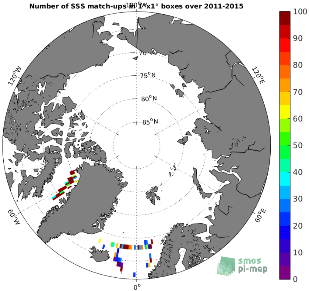
Figure 4: Number of SSS match-ups between TSG-LEGOS-DM SSS and the Aquarius-L2-OR-V5 SSS product for the Arctic Ocean Pi-MEP region over 1°x1° boxes and for the full satellite product period.
