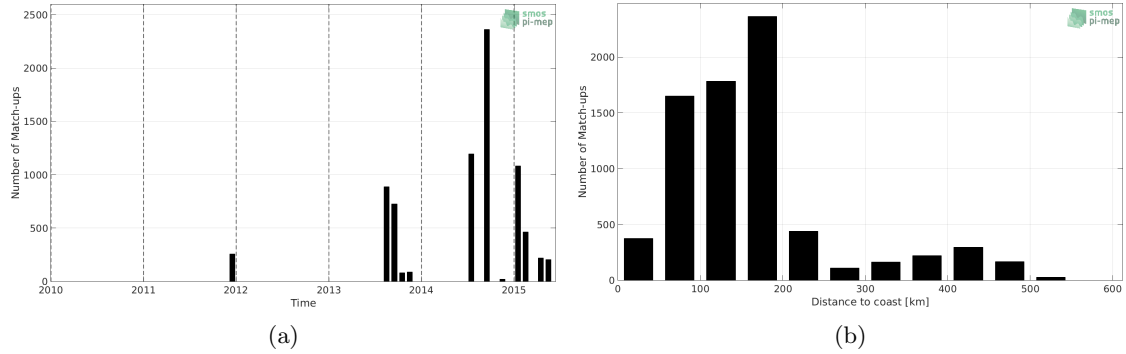
Figure 1: Number of match-ups between TSG-LEGOS-DM and Aquarius-L2-OR-V5 SSS as a function of time (a) and as function of the distance to coast (b) over the Arctic Ocean Pi-MEP region and for the full satellite product period.
