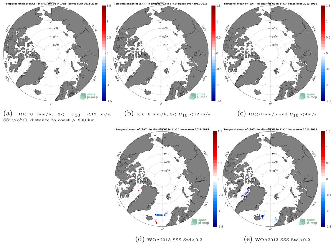
Figure 12: Temporal mean gridded over spatial boxes of size 1^\circ \times 1^\circ of \Delta SSS (Aquarius-L2-OR-V5 - TSG-LEGOS-DM) for 5 different subdatasets corresponding to:RR=0 mm/h, 3 < U_{10} < 12 m/s, SST >5^\circ\text{C} , distance to coast > 800 km (a), RR=0 mm/h, 3 < U_{10} < 12 m/s (b), RR >1 mm/h and U_{10} < 4 m/s (c), WOA2013 SSS Std <0.2 (d), WOA2013 SSS Std >0.2 (e).
