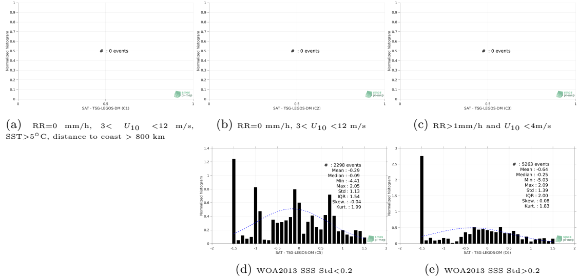
Figure 13: Normalized histogram of \Delta SSS (Aquarius-L2-OR-V5 - TSG-LEGOS-DM) for 5 different subdatasets corresponding to: RR=0 mm/h, 3 < U_{10} < 12 m/s, SST > 5°C, distance to coast > 800 km (a), RR=0 mm/h, 3 < U_{10} < 12 m/s (b), RR > 1mm/h and U_{10} < 4 m/s (c), WOA2013 SSS Std < 0.2 (d), WOA2013 SSS Std > 0.2 (e).
