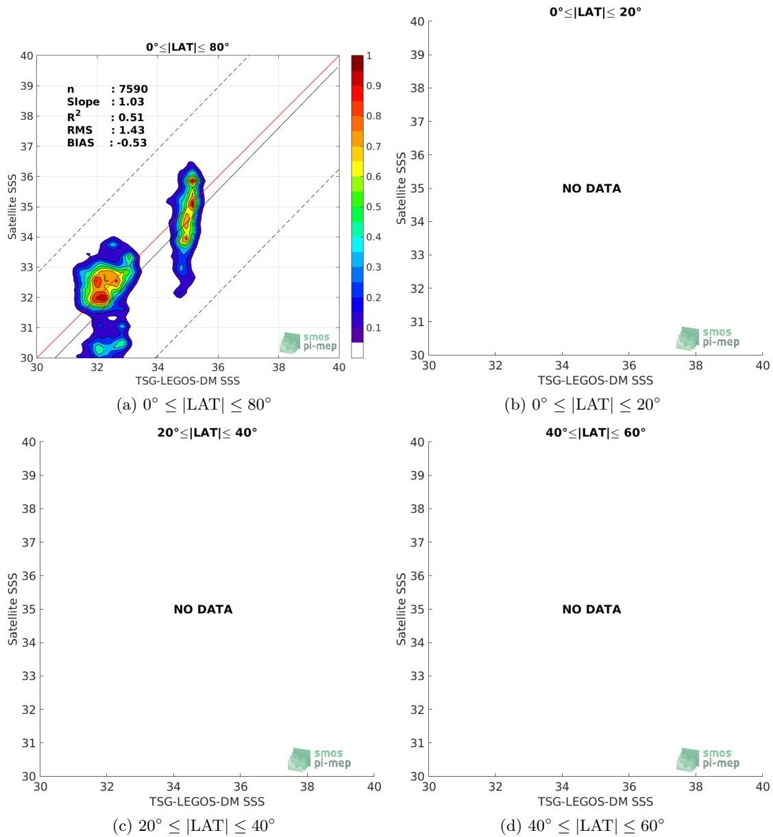
Figure 9: Contour maps of the concentration of Aquarius-L2-OR-V5 SSS (y-axis) versus TSG-LEGOS-DM SSS (x-axis) at match-up pairs for different latitude bands. For each plot, the red line shows x=y . The black thin and dashed lines indicate a linear fit through the data cloud and the \pm 95\% confidence levels, respectively. The number match-up pairs n , the slope and R^2 coefficient of the linear fit, the root mean square (RMS) and the mean bias between satellite and in situ data are indicated for each latitude band in each plots.
