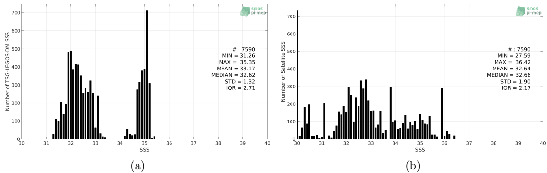
Figure 2: Histograms of SSS from TSG-LEGOS-DM (a) and Aquarius-L2-OR-V5 (b) considering all match-up pairs per bins of 0.1 over the Arctic Ocean Pi-MEP region and for the full satellite product period.
