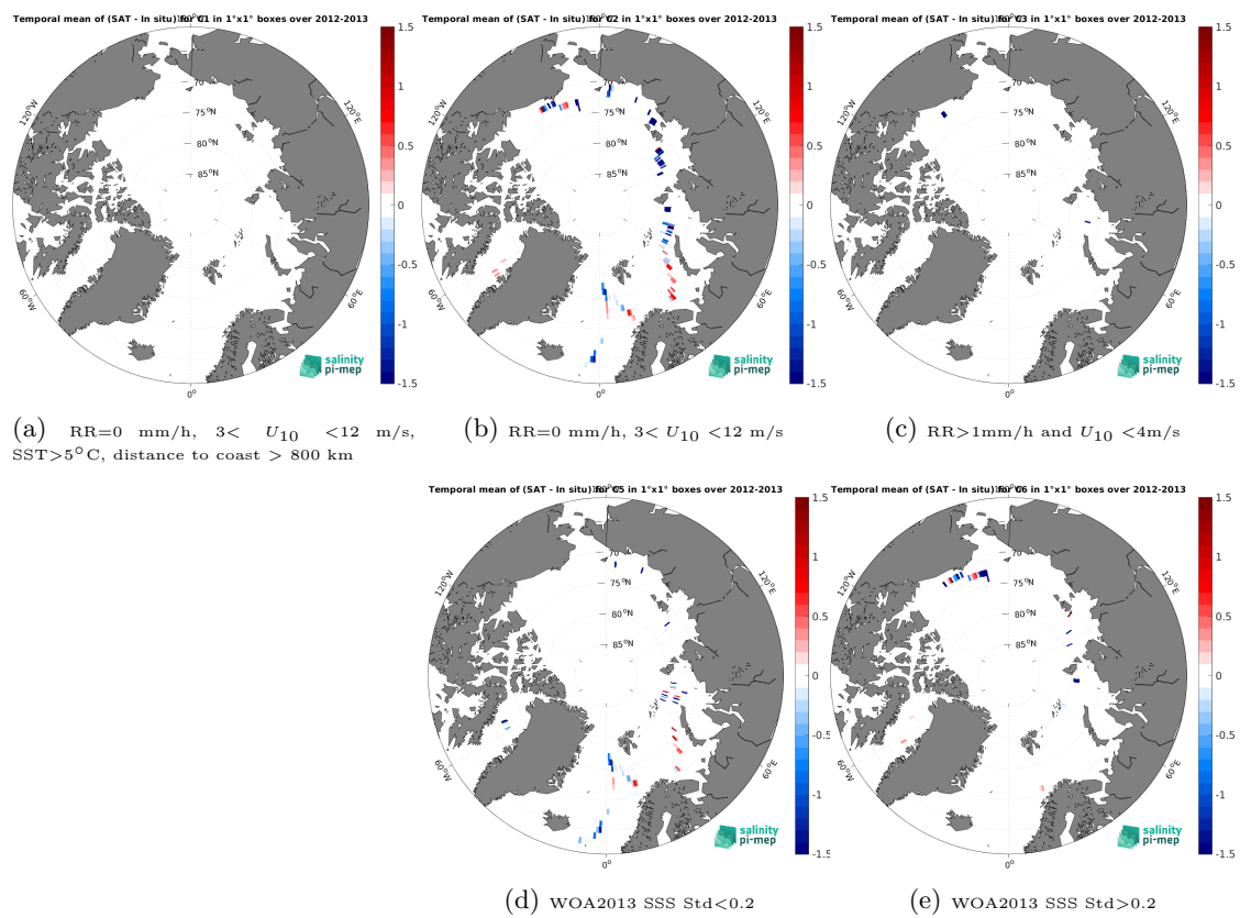
Figure 14: Temporal mean gridded over spatial boxes of size 1^\circ \times 1^\circ of \Delta\text{SSS} (Aquarius SSS L2 OR v5 (NASA-GSFC) - TSG (GOSUD-Sailing-ship)) for 5 different subdatasets corresponding to: RR=0 mm/h, 3 < U_{10} < 12 m/s, SST > 5°C, distance to coast > 800 km (a), RR=0 mm/h, 3 < U_{10} < 12 m/s (b), RR > 1mm/h and U_{10} < 4 m/s (c), WOA2013 SSS Std < 0.2 (d), WOA2013 SSS Std > 0.2 (e).
