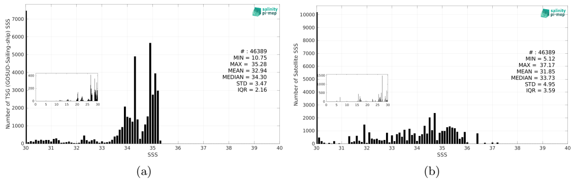
Figure 3: Histograms of SSS from TSG (GOSUD-Sailing-ship) (a) and Aquarius SSS L2 OR v5 (NASA-GSFC) (b) considering all match-up pairs per bins of 0.1 over the Arctic Ocean Pi-MEP region and for the full satellite product period.
