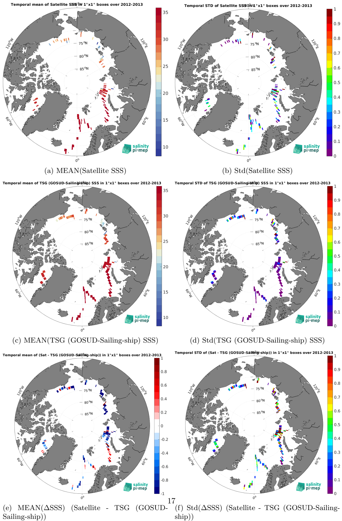
Figure 7: Temporal mean (left) and Std (right) of SSS from Aquarius SSS L2 OR v5 (NASA-GSFC) (top), TSG (GOSUD-Sailing-ship) (middle), and of \Delta SSS (Satellite - TSG (GOSUD-Sailing-ship)). Only match-up pairs are used to generate these maps.
