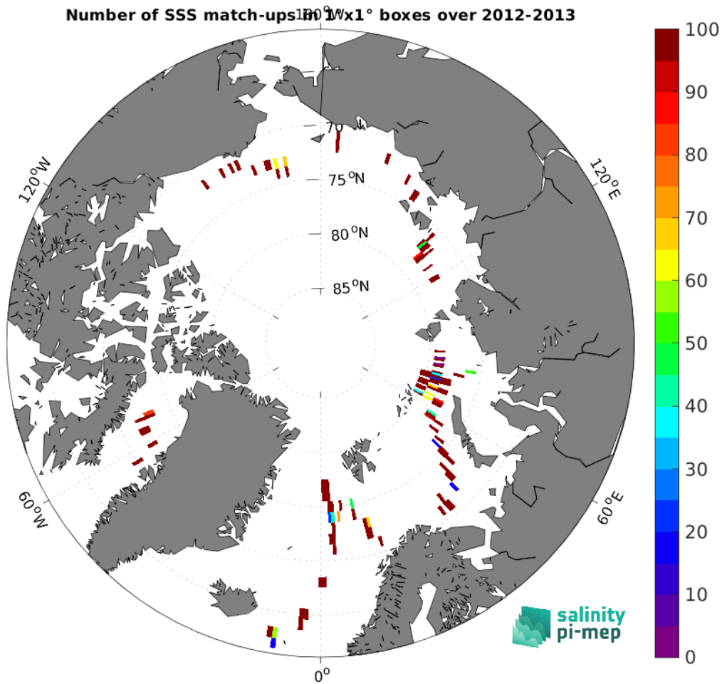
Figure 5: Number of SSS match-ups between TSG (GOSUD-Sailing-ship) SSS and the Aquarius SSS L2 OR v5 (NASA-GSFC) SSS product for the Arctic Ocean Pi-MEP region over 1^\circ \times 1^\circ boxes and for the full satellite product period.
