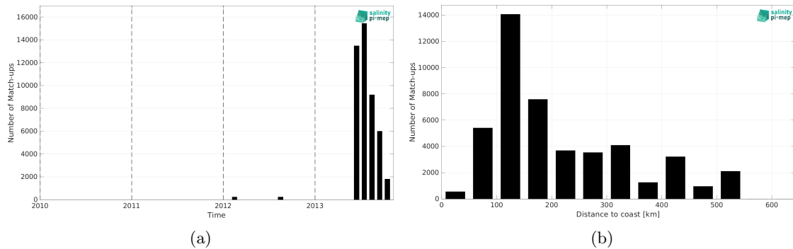
Figure 2: Number of match-ups between TSG (GOSUD-Sailing-ship) and Aquarius SSS L2 OR v5 (NASA-GSFC) SSS as a function of time (a) and as function of the distance to coast (b) over the Arctic Ocean Pi-MEP region and for the full satellite product period.
