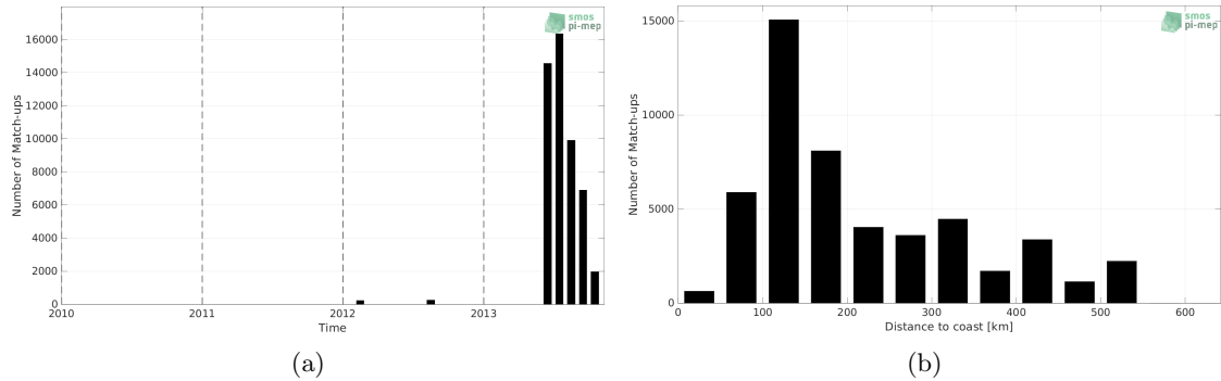
Figure 1: Number of match-ups between TSG (GOSUD-Sailing-ship) and Aquarius SSS L2 OR v5 (NASA-GSFC) SSS as a function of time (a) and as function of the distance to coast (b) over the Arctic Ocean Pi-MEP region and for the full satellite product period.
