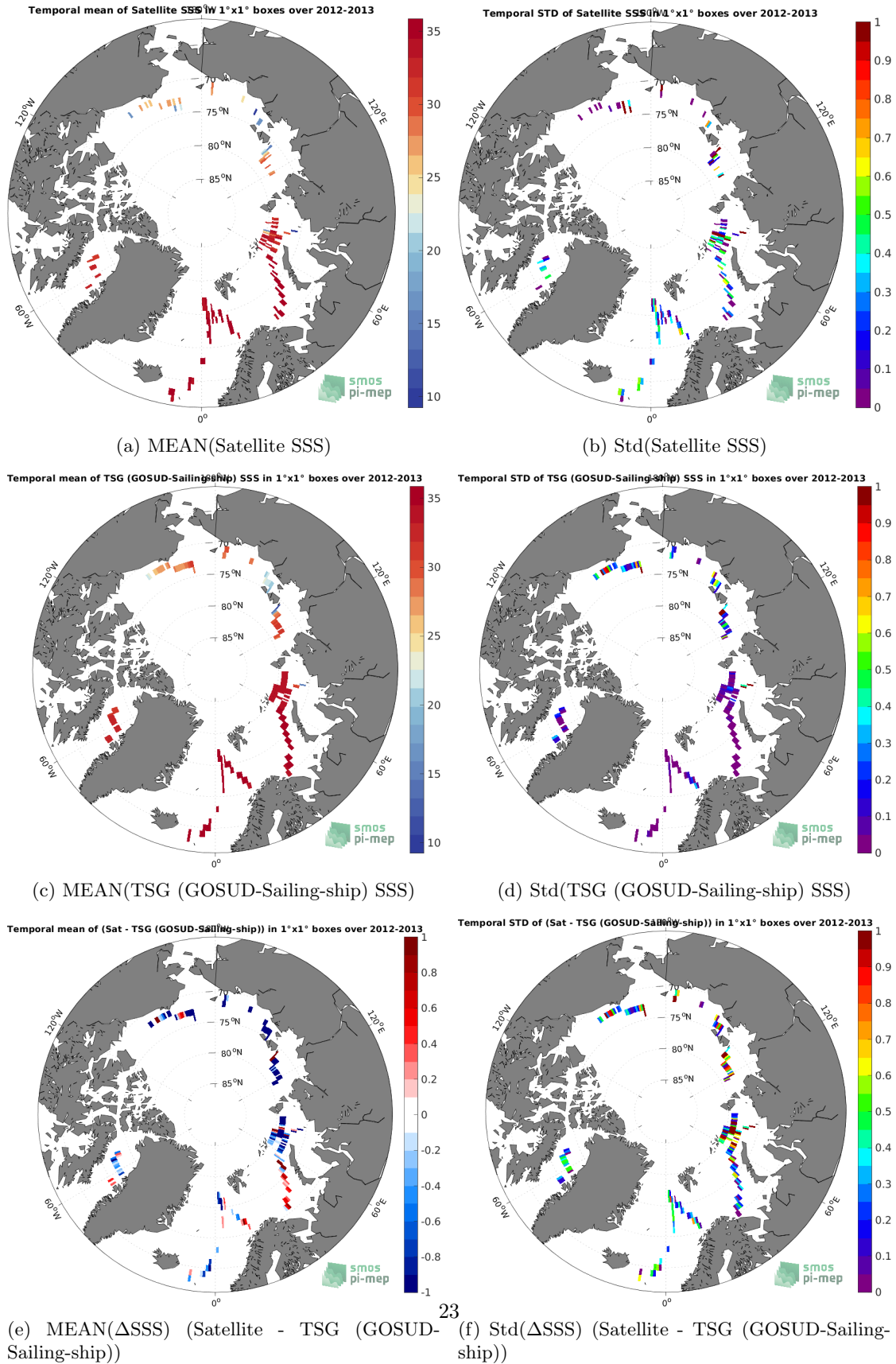
Figure 6: Temporal mean (left) and Std (right) of SSS from Aquarius SSS L2 OR v5 (NASA-GSFC) (top), TSG (GOSUD-Sailing-ship) (middle), and of \Delta SSS (Satellite - TSG (GOSUD-Sailing-ship)). Only match-up pairs are used to generate these maps.
