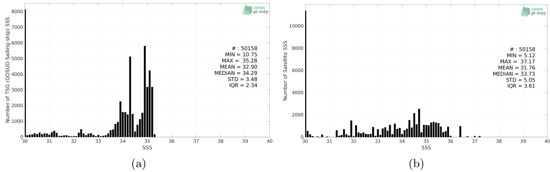
Figure 2: Histograms of SSS from TSG (GOSUD-Sailing-ship) (a) and Aquarius SSS L2 OR v5 (NASA-GSFC) (b) considering all match-up pairs per bins of 0.1 over the Arctic Ocean Pi-MEP region and for the full satellite product period.
