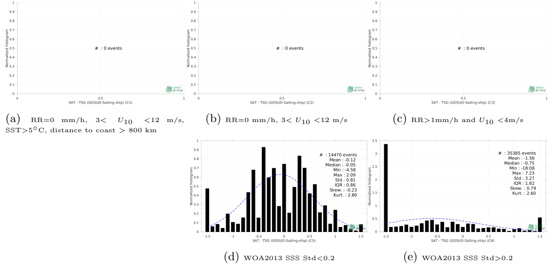
Figure 13: Normalized histogram of \Delta SSS (Aquarius SSS L2 OR v5 (NASA-GSFC) - TSG (GOSUD-Sailing-ship)) for 5 different subdatasets corresponding to: RR=0 mm/h, 3 < U_{10} < 12 m/s, SST>5°C, distance to coast > 800 km (a), RR=0 mm/h, 3 < U_{10} < 12 m/s (b), RR>1mm/h and U_{10} < 4 m/s (c), WOA2013 SSS Std<0.2 (d), WOA2013 SSS Std>0.2 (e).
