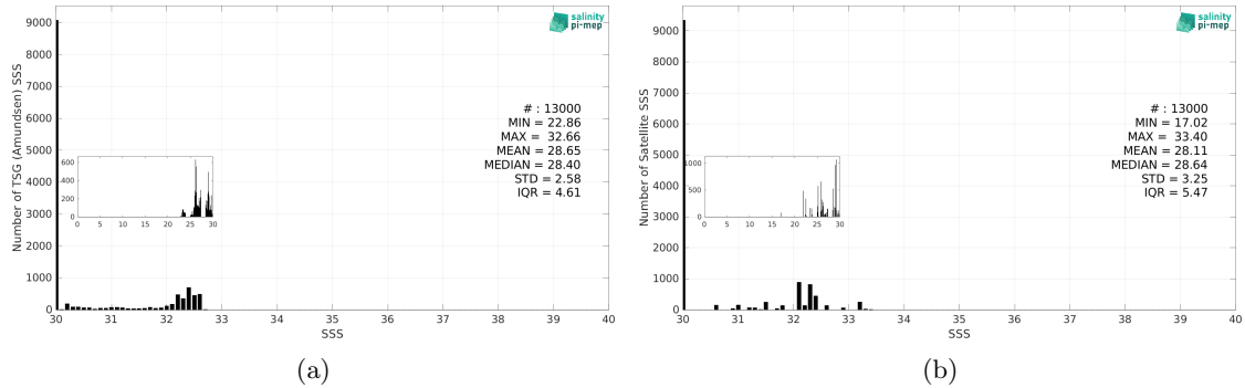
Figure 3: Histograms of SSS from TSG (Amundsen) (a) and Aquarius SSS L2 OR v5 (NASA-GSFC) (b) considering all match-up pairs per bins of 0.1 over the Arctic Ocean Pi-MEP region and for the full satellite product period.
