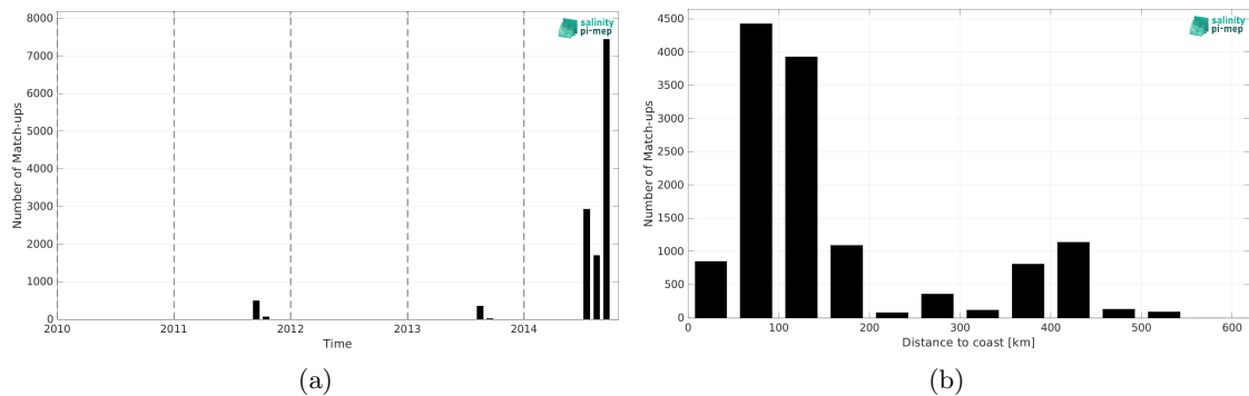
Figure 2: Number of match-ups between TSG (Amundsen) and Aquarius SSS L2 OR v5 (NASA-GSFC) SSS as a function of time (a) and as function of the distance to coast (b) over the Arctic Ocean Pi-MEP region and for the full satellite product period.
