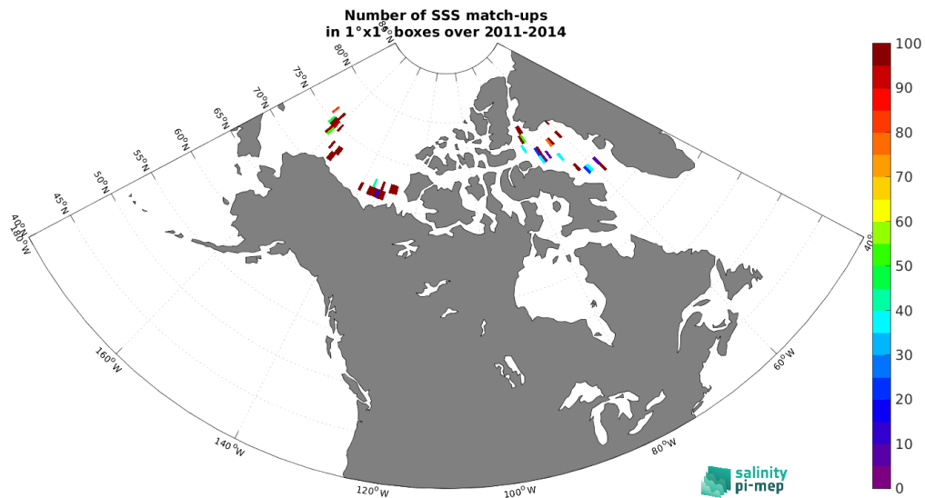
Figure 5: Number of SSS match-ups between TSG (Amundsen) SSS and the Aquarius SSS L2 OR v5 (NASA-GSFC) SSS product for the Arctic Ocean Pi-MEP region over 1^\circ \times 1^\circ boxes and for the full satellite product period.
