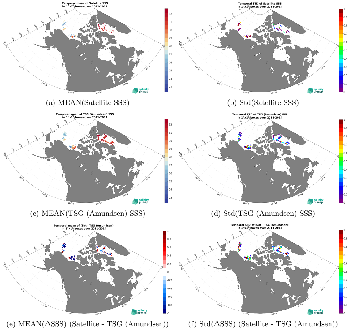
Figure 6: Temporal mean (left) and Std (right) of SSS from Aquarius SSS L2 OR v5 (NASA-GSFC) (top), TSG (Amundsen) (middle), and of \Delta SSS (Satellite - TSG (Amundsen)). Only match-up pairs are used to generate these maps.
