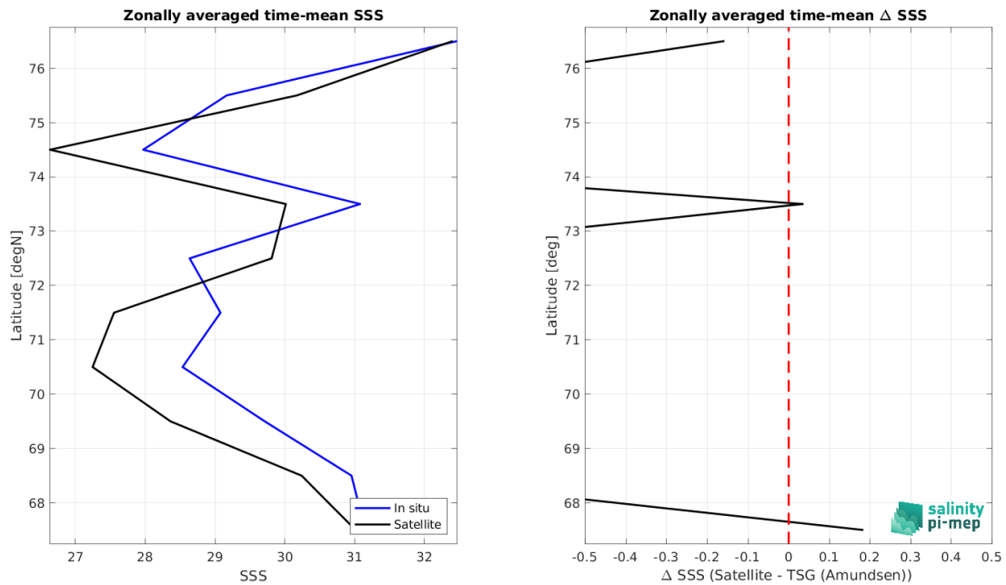
Figure 8: Left panel: Zonal mean SSS from Aquarius SSS L2 OR v5 (NASA-GSFC) satellite product (black) and from TSG (Amundsen) (blue). Right panel: Zonal mean of \Delta SSS (Satellite - TSG (Amundsen)) for all the collected Pi-MEP match-up pairs estimated over the full satellite product period.
