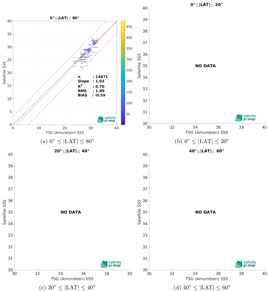
Figure 9: Contour maps of the concentration of Aquarius SSS L2 OR v5 (NASA-GSFC) SSS (y-axis) versus TSG (Amundsen) SSS (x-axis) at match-up pairs for different latitude bands. For each plot, the red line shows x=y . The black thin and dashed lines indicate a linear fit through the data cloud and the \pm 95\% confidence levels, respectively. The number match-up pairs n , the slope and R^2 coefficient of the linear fit, the root mean square (RMS) and the mean bias between satellite and in situ data are indicated for each latitude band in each plots.
