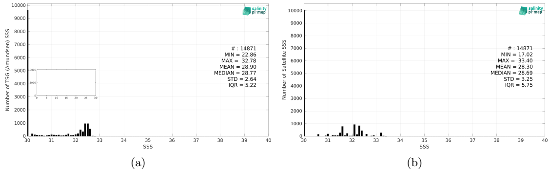
Figure 2: Histograms of SSS from TSG (Amundsen) (a) and Aquarius SSS L2 OR v5 (NASA-GSFC) (b) considering all match-up pairs per bins of 0.1 over the Arctic Ocean Pi-MEP region and for the full satellite product period.
