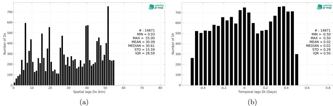
Figure 5: Histograms of the spatial (a) and temporal (b) lags between the location/time of the TSG (Amundsen) measurement and the date of the corresponding Aquarius SSS L2 OR v5 (NASA-GSFC) SSS pixel.
