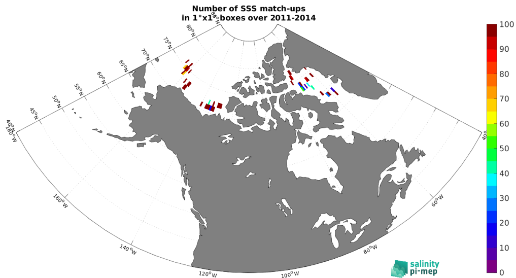
Figure 4: Number of SSS match-ups between TSG (Amundsen) SSS and the Aquarius SSS L2 OR v5 (NASA-GSFC) SSS product for the Arctic Ocean Pi-MEP region over 1^\circ \times 1^\circ boxes and for the full satellite product period.
