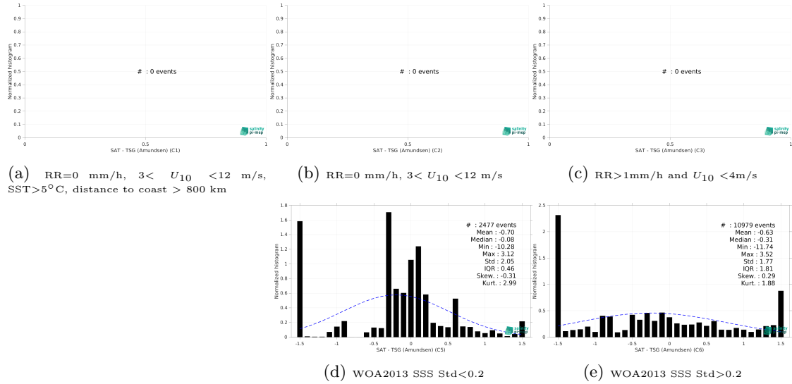
Figure 13: Normalized histogram of \Delta SSS (Aquarius SSS L2 OR v5 (NASA-GSFC) - TSG (Amundsen)) for 5 different subdatasets corresponding to: RR=0 mm/h, 3 < U_{10} < 12 m/s, SST>5°C, distance to coast > 800 km (a), RR=0 mm/h, 3 < U_{10} < 12 m/s (b), RR>1mm/h and U_{10} < 4 m/s (c), WOA2013 SSS Std<0.2 (d), WOA2013 SSS Std>0.2 (e).
