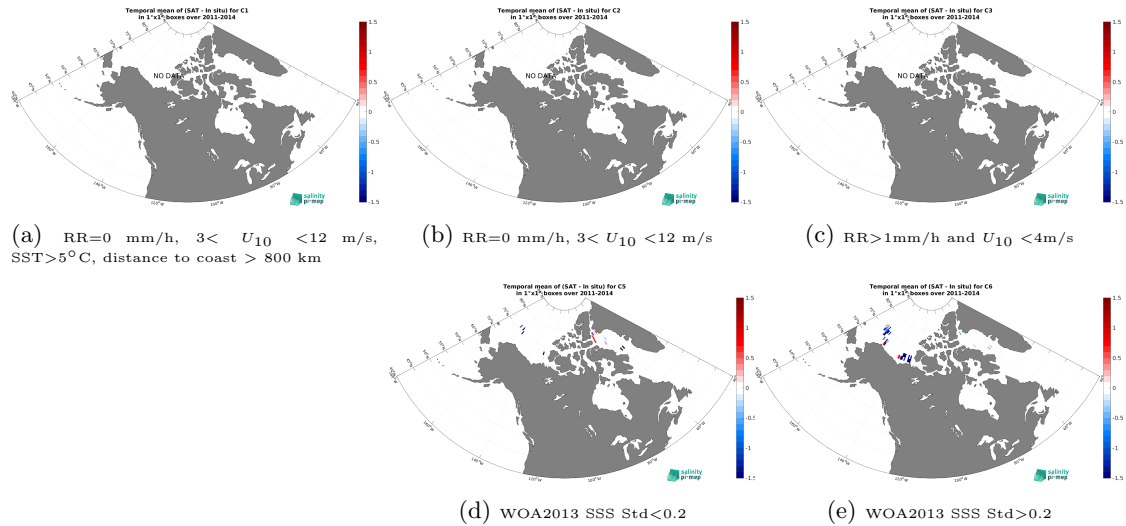
Figure 12: Temporal mean gridded over spatial boxes of size 1^{\circ}\times 1^{\circ} of \Delta\text{SSS} (Aquarius SSS L2 OR v5 (NASA-GSFC) - TSG (Amundsen)) for 5 different subdatasets corresponding to:RR=0 mm/h, 3 < U_{10} < 12 m/s, SST > 5^{\circ}\text{C} , distance to coast > 800 km (a), RR=0 mm/h, 3 < U_{10} < 12 m/s (b), RR > 1 mm/h and U_{10} < 4 m/s (c), WOA2013 SSS Std < 0.2 (d), WOA2013 SSS Std > 0.2 (e).
