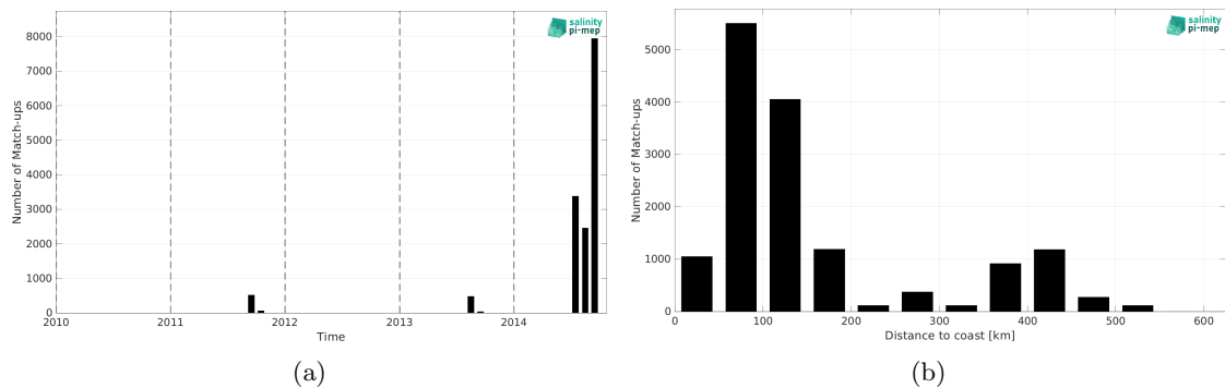
Figure 1: Number of match-ups between TSG (Amundsen) and Aquarius SSS L2 OR v5 (NASA-GSFC) SSS as a function of time (a) and as function of the distance to coast (b) over the Arctic Ocean Pi-MEP region and for the full satellite product period.
