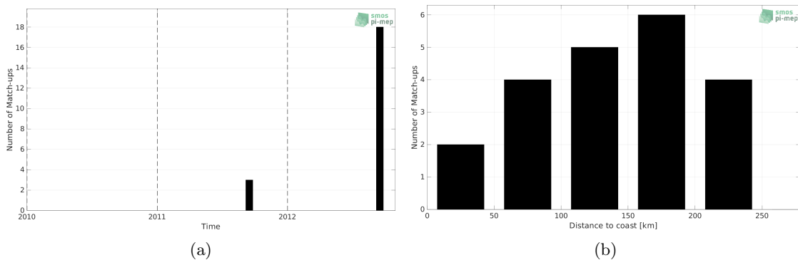
Figure 1: Number of match-ups between Marine mammals and Aquarius SSS L2 OR v5 (NASA-GSFC) SSS as a function of time (a) and as function of the distance to coast (b) over the Arctic Ocean Pi-MEP region and for the full satellite product period.
