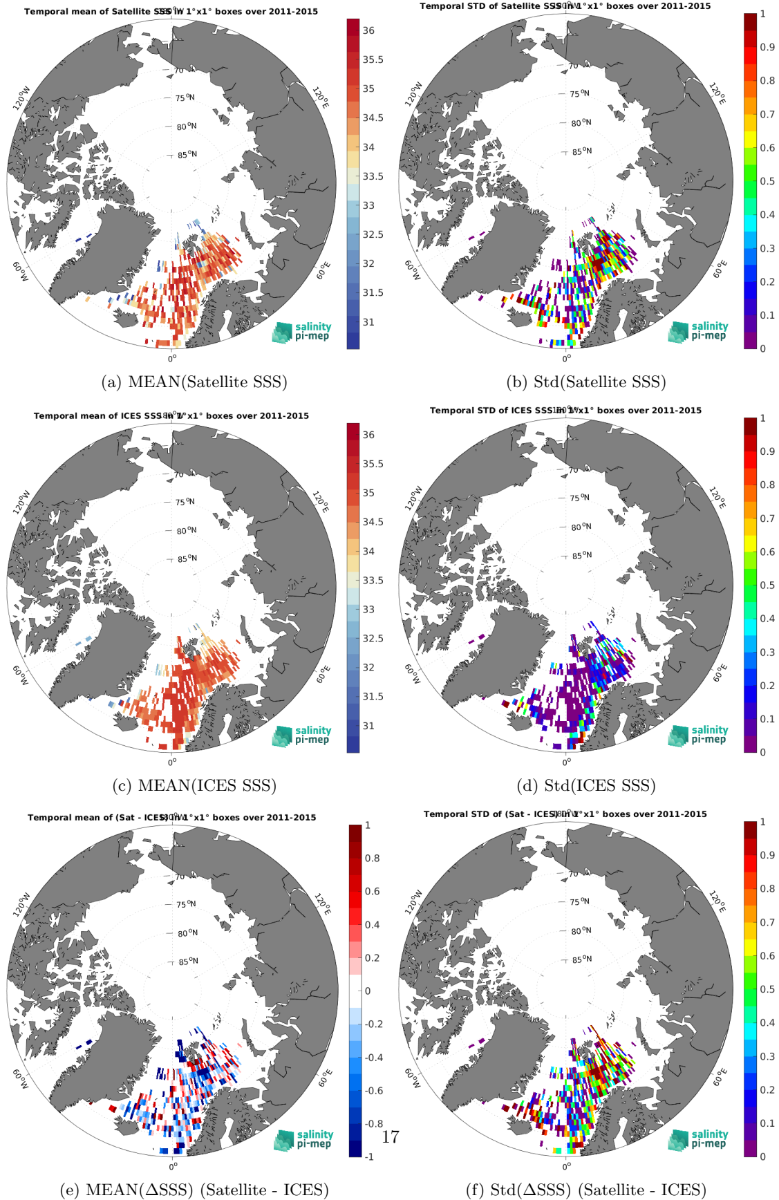
Figure 7: Temporal mean (left) and Std (right) of SSS from Aquarius SSS L2 OR v5 (NASA-GSFC) (top), ICES (middle), and of \Delta SSS (Satellite - ICES). Only match-up pairs are used to generate these maps.
