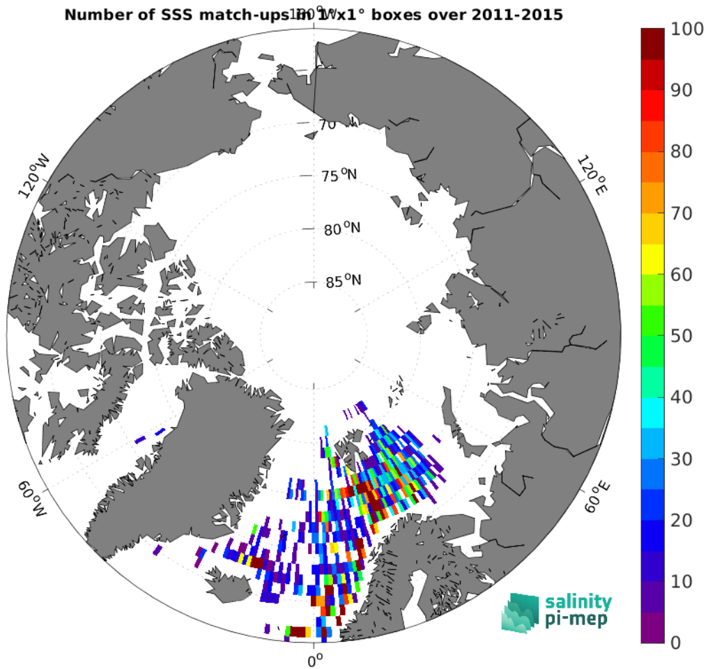
Figure 5: Number of SSS match-ups between ICES SSS and the Aquarius SSS L2 OR v5 (NASA-GSFC) SSS product for the Arctic Ocean Pi-MEP region over 1^\circ \times 1^\circ boxes and for the full satellite product period.
