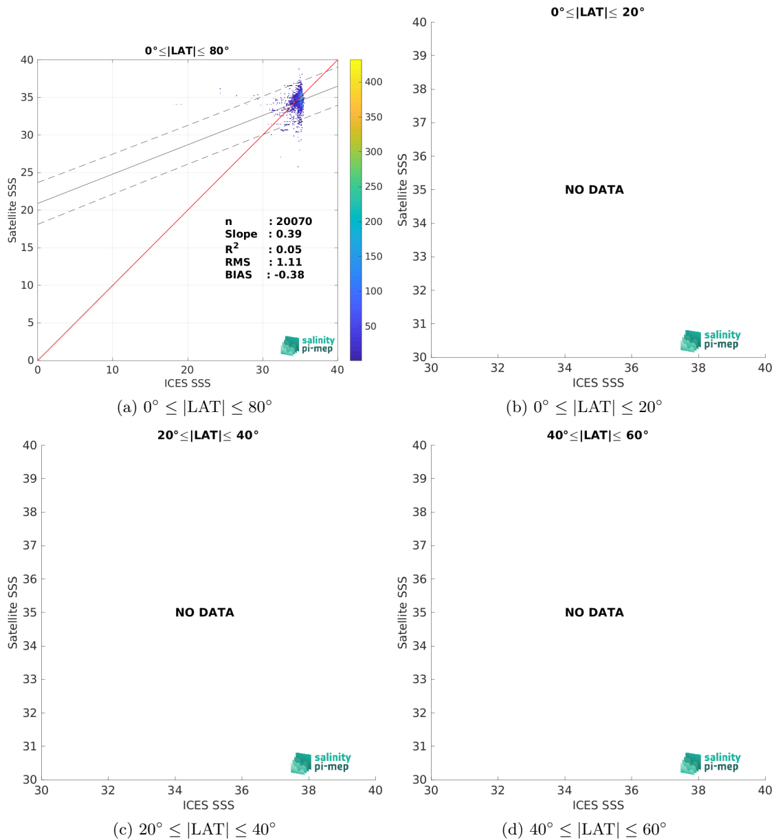
Figure 10: Contour maps of the concentration of Aquarius SSS L2 OR v5 (NASA-GSFC) SSS (y-axis) versus ICES SSS (x-axis) at match-up pairs for different latitude bands. For each plot, the red line shows x=y . The black thin and dashed lines indicate a linear fit through the data cloud and the \pm 95\% confidence levels, respectively. The number match-up pairs n , the slope and R^2 coefficient of the linear fit, the root mean square (RMS) and the mean bias between satellite and in situ data are indicated for each latitude band in each plots.
