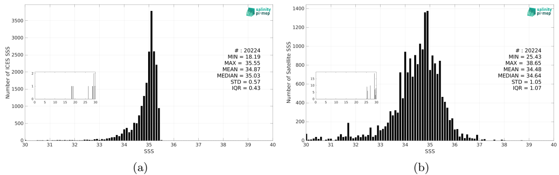
Figure 3: Histograms of SSS from ICES (a) and Aquarius SSS L2 OR v5 (NASA-GSFC) (b) considering all match-up pairs per bins of 0.1 over the Arctic Ocean Pi-MEP region and for the full satellite product period.
