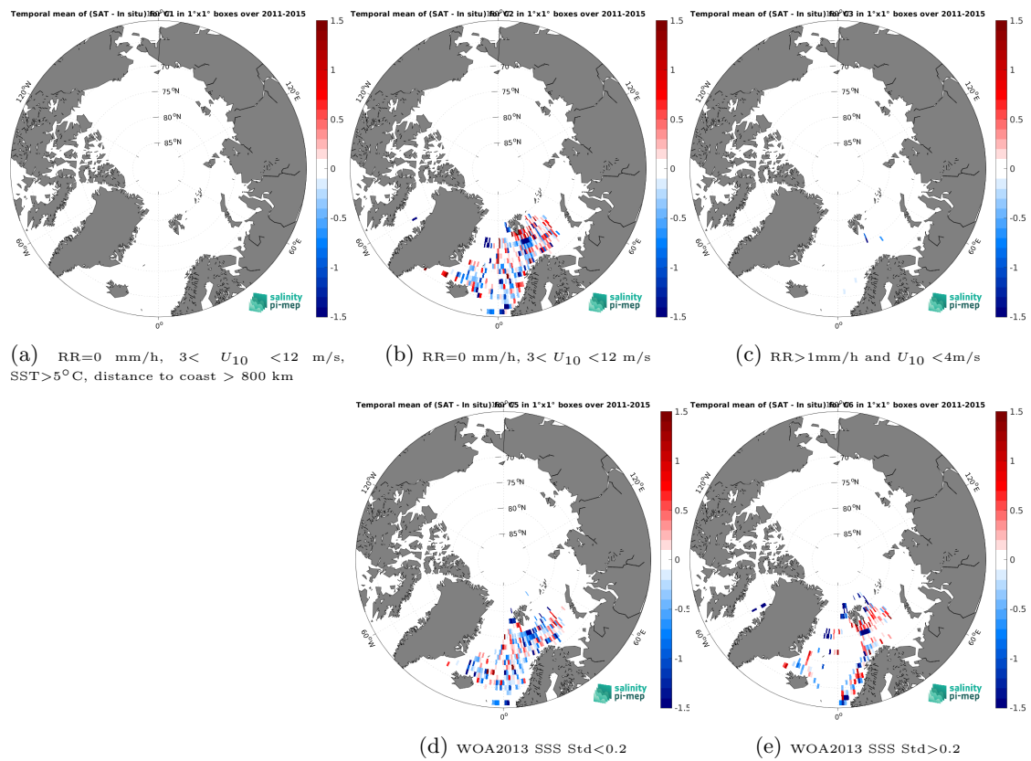
Figure 14: Temporal mean gridded over spatial boxes of size 1^\circ \times 1^\circ of \Delta SSS (Aquarius SSS L2 OR v5 (NASA-GSFC) - ICES) for 5 different subdatasets corresponding to: RR=0 mm/h, 3 < U_{10} < 12 m/s, SST > 5°C, distance to coast > 800 km (a), RR=0 mm/h, 3 < U_{10} < 12 m/s (b), RR > 1mm/h and U_{10} < 4 m/s (c), WOA2013 SSS Std < 0.2 (d), WOA2013 SSS Std > 0.2 (e).
