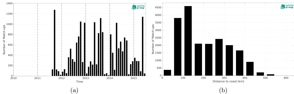
Figure 2: Number of match-ups between ICES and Aquarius SSS L2 OR v5 (NASA-GSFC) SSS as a function of time (a) and as function of the distance to coast (b) over the Arctic Ocean Pi-MEP region and for the full satellite product period.
