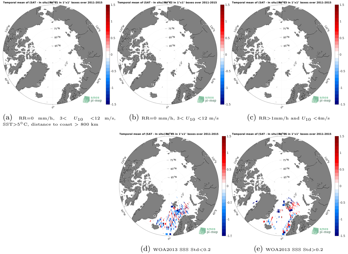
Figure 12: Temporal mean gridded over spatial boxes of size 1^{\circ}\times 1^{\circ} of \Delta\text{SSS} (Aquarius SSS L2 OR v5 (NASA-GSFC) - ICES) for 5 different subdatasets corresponding to:RR=0 mm/h, 3 < U_{10} < 12 m/s, SST >5^{\circ}\text{C} , distance to coast > 800 km (a), RR=0 mm/h, 3 < U_{10} < 12 m/s (b), RR >1 mm/h and U_{10} < 4 m/s (c), WOA2013 SSS Std <0.2 (d), WOA2013 SSS Std >0.2 (e).
