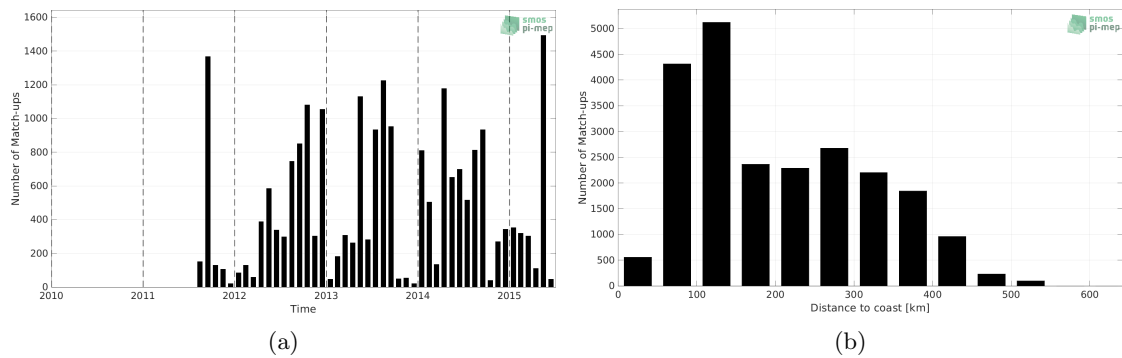
Figure 1: Number of match-ups between ICES and Aquarius SSS L2 OR v5 (NASA-GSFC) SSS as a function of time (a) and as function of the distance to coast (b) over the Arctic Ocean Pi-MEP region and for the full satellite product period.
