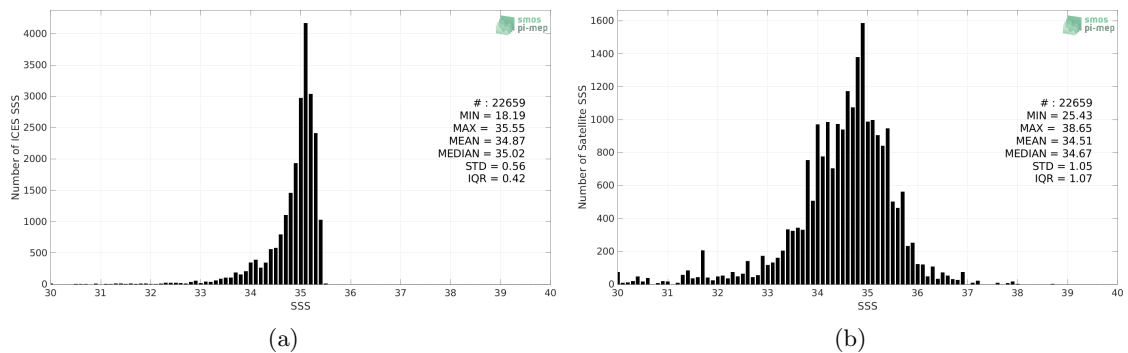
Figure 2: Histograms of SSS from ICES (a) and Aquarius SSS L2 OR v5 (NASA-GSFC) (b) considering all match-up pairs per bins of 0.1 over the Arctic Ocean Pi-MEP region and for the full satellite product period.
