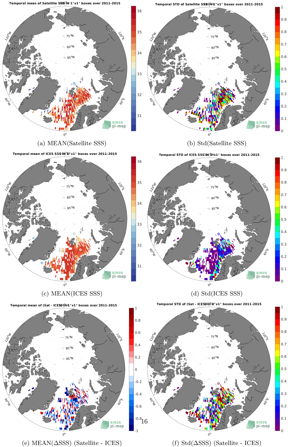
Figure 6: Temporal mean (left) and Std (right) of SSS from Aquarius SSS L2 OR v5 (NASA-GSFC) (top), ICES (middle), and of \Delta SSS (Satellite - ICES). Only match-up pairs are used to generate these maps.
