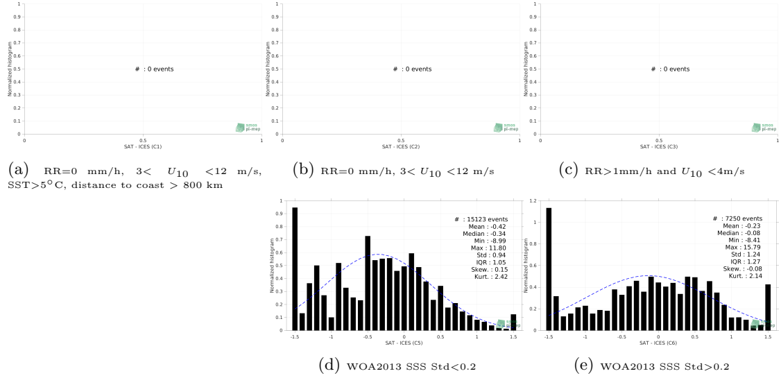
Figure 13: Normalized histogram of \Delta SSS (Aquarius SSS L2 OR v5 (NASA-GSFC) - ICES) for 5 different subdatasets corresponding to: RR=0 mm/h, 3 < U_{10} < 12 m/s, SST > 5°C, distance to coast > 800 km (a), RR=0 mm/h, 3 < U_{10} < 12 m/s (b), RR > 1mm/h and U_{10} < 4 m/s (c), WOA2013 SSS Std < 0.2 (d), WOA2013 SSS Std > 0.2 (e).
