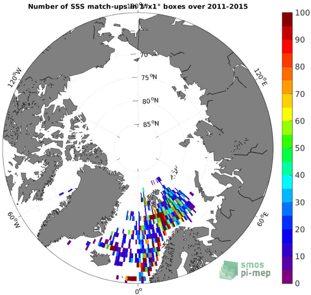
Figure 4: Number of SSS match-ups between ICES SSS and the Aquarius SSS L2 OR v5 (NASA-GSFC) SSS product for the Arctic Ocean Pi-MEP region over 1^\circ \times 1^\circ boxes and for the full satellite product period.
