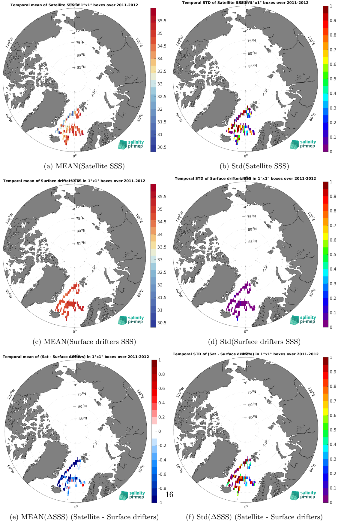
Figure 6: Temporal mean (left) and Std (right) of SSS from Aquarius SSS L2 OR v5 (NASA-GSFC) (top), Surface drifters (middle), and of \Delta SSS (Satellite - Surface drifters). Only match-up pairs are used to generate these maps.
