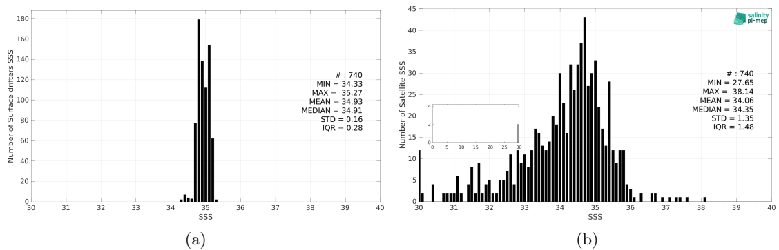
Figure 3: Histograms of SSS from Surface drifters (a) and Aquarius SSS L2 OR v5 (NASA-GSFC) (b) considering all match-up pairs per bins of 0.1 over the Arctic Ocean Pi-MEP region and for the full satellite product period.
