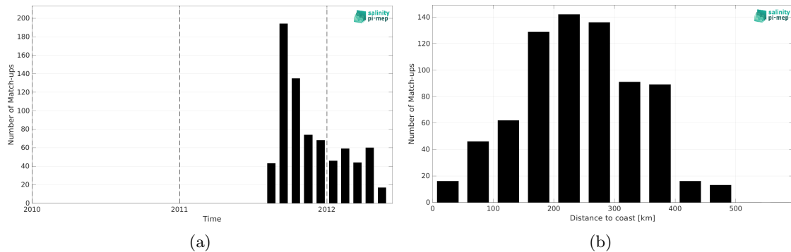
Figure 2: Number of match-ups between Surface drifters and Aquarius SSS L2 OR v5 (NASA-GSFC) SSS as a function of time (a) and as function of the distance to coast (b) over the Arctic Ocean Pi-MEP region and for the full satellite product period.
