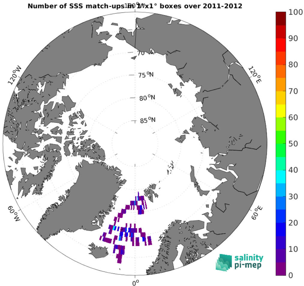
Figure 4: Number of SSS match-ups between Surface drifters SSS and the Aquarius SSS L2 OR v5 (NASA-GSFC) SSS product for the Arctic Ocean Pi-MEP region over 1^\circ \times 1^\circ boxes and for the full satellite product period.
