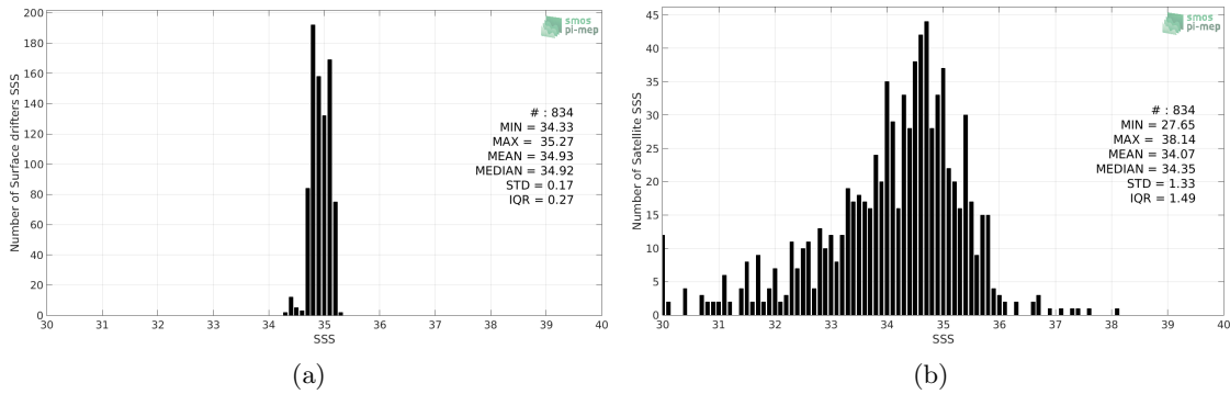
Figure 2: Histograms of SSS from Surface drifters (a) and Aquarius-L2-OR-V5 (b) considering all match-up pairs per bins of 0.1 over the Arctic Ocean Pi-MEP region and for the full satellite product period.
