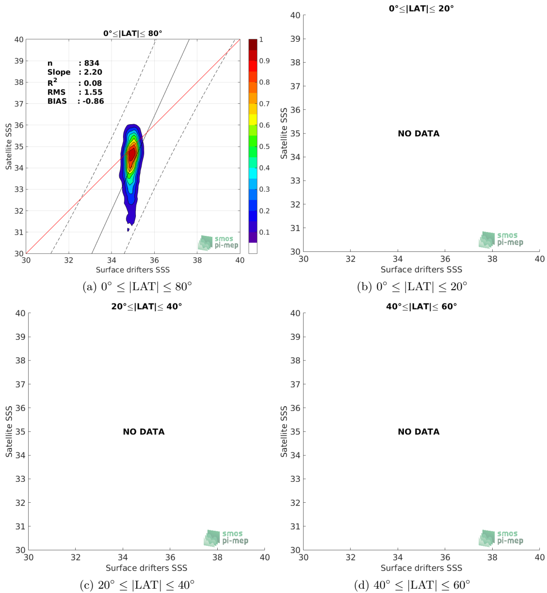
Figure 8: Contour maps of the concentration of Aquarius-L2-OR-V5 SSS (y-axis) versus Surface drifters SSS (x-axis) at match-up pairs for different latitude bands. For each plot, the red line shows x=y . The black thin and dashed lines indicate a linear fit through the data cloud and the \pm 95\% confidence levels, respectively. The number match-up pairs n , the slope and R^2 coefficient of the linear fit, the root mean square (RMS) and the mean bias between satellite and in situ data are indicated for each latitude band in each plots.
