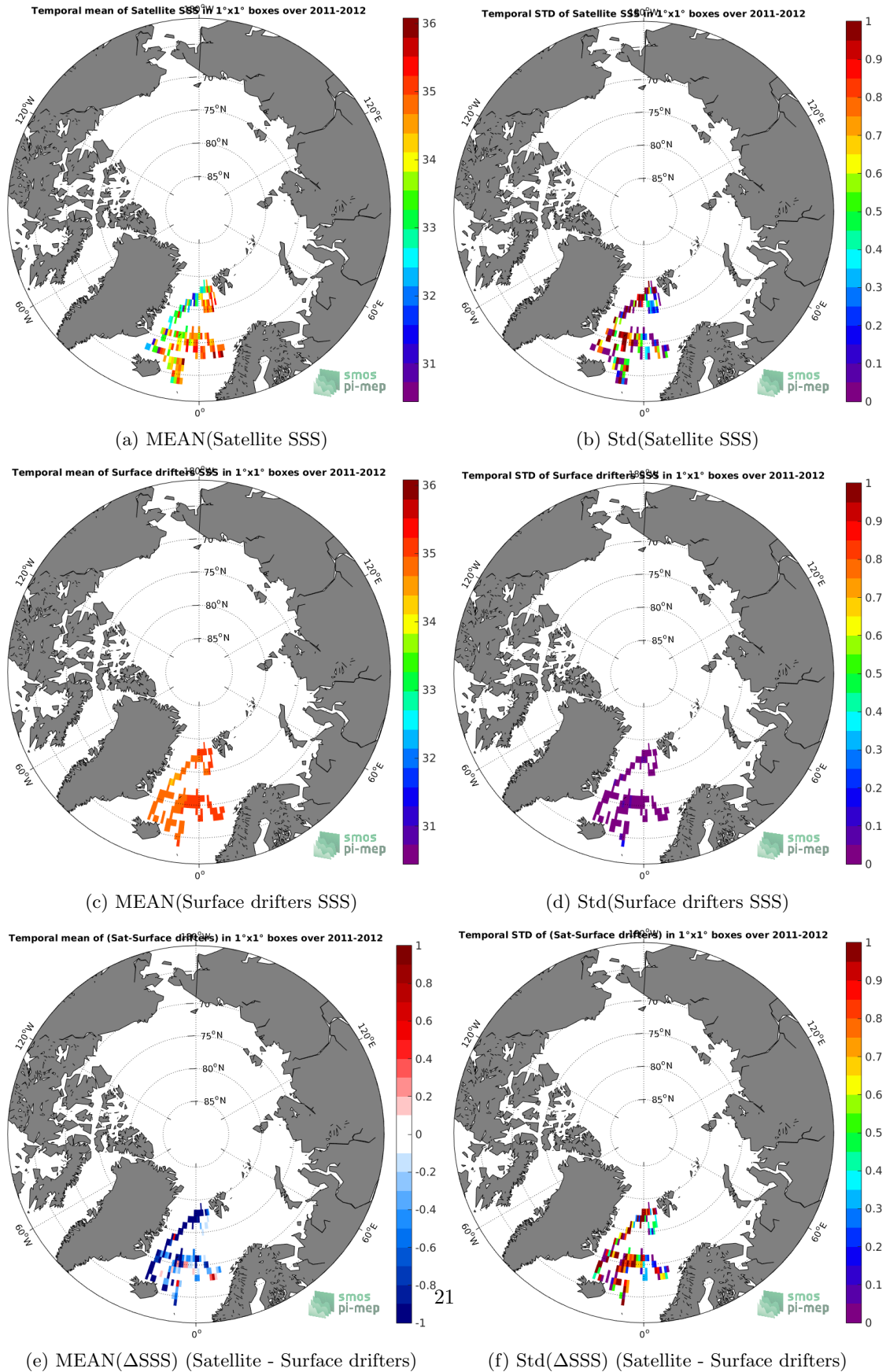
Figure 5: Temporal mean (left) and Std (right) of SSS from Aquarius-L2-OR-V5 (top), Surface drifters (middle), and of \Delta SSS (Satellite - Surface drifters). Only match-up pairs are used to generate these maps.
