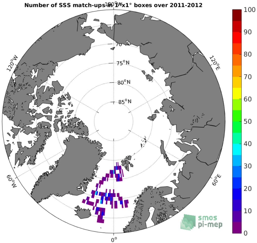
Figure 3: Number of SSS match-ups between Surface drifters SSS and the Aquarius-L2-OR-V5 SSS product for the Arctic Ocean Pi-MEP region over 1°x1° boxes and for the full satellite product period.
