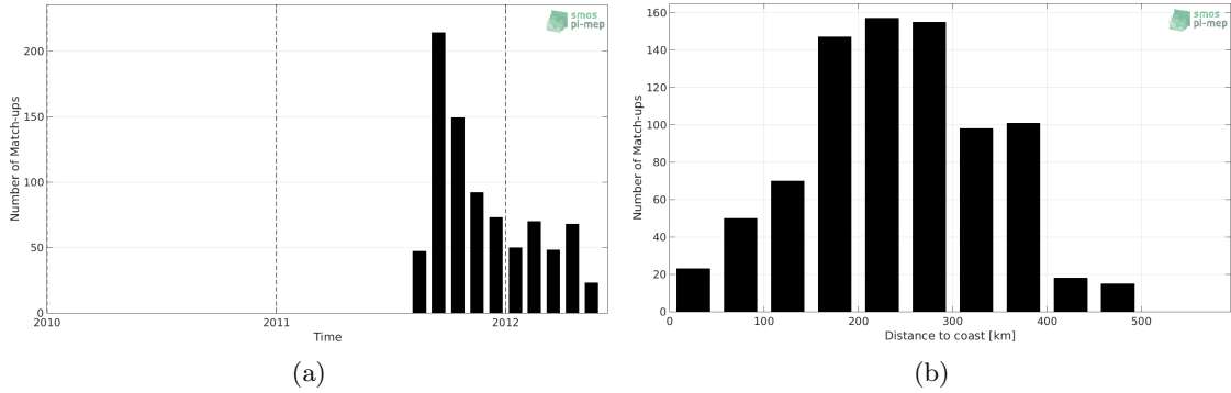
Figure 1: Number of match-ups between Surface drifters and Aquarius-L2-OR-V5 SSS as a function of time (a) and as function of the distance to coast (b) over the Arctic Ocean Pi-MEP region and for the full satellite product period.
