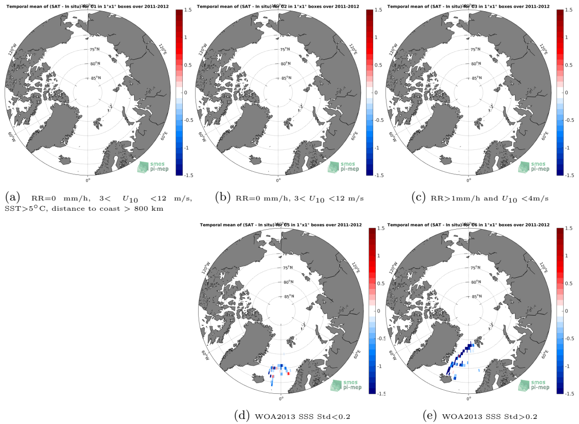
Figure 11: Temporal mean gridded over spatial boxes of size 1^\circ \times 1^\circ of \Delta SSS (Aquarius-L2-OR-V5 - Surface drifters) for 5 different subdatasets corresponding to:RR=0 mm/h, 3 < U_{10} < 12 m/s, SST >5^\circ\text{C} , distance to coast > 800 km (a), RR=0 mm/h, 3 < U_{10} < 12 m/s (b), RR >1 mm/h and U_{10} < 4 m/s (c), WOA2013 SSS Std <0.2 (d), WOA2013 SSS Std >0.2 (e).
