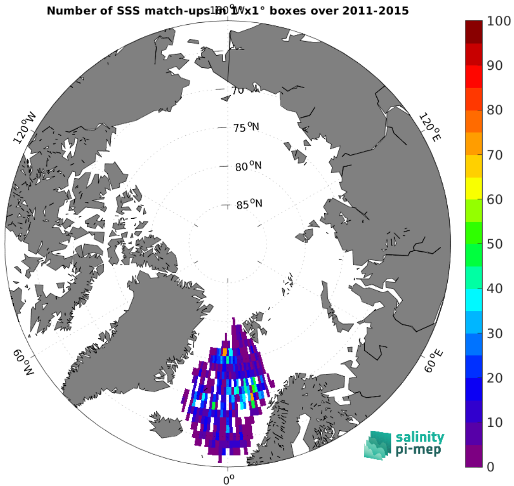
Figure 5: Number of SSS match-ups between Argo SSS and the Aquarius SSS L2 OR v5 (NASA-GSFC) SSS product for the Arctic Ocean Pi-MEP region over 1^\circ \times 1^\circ boxes and for the full satellite product period.
