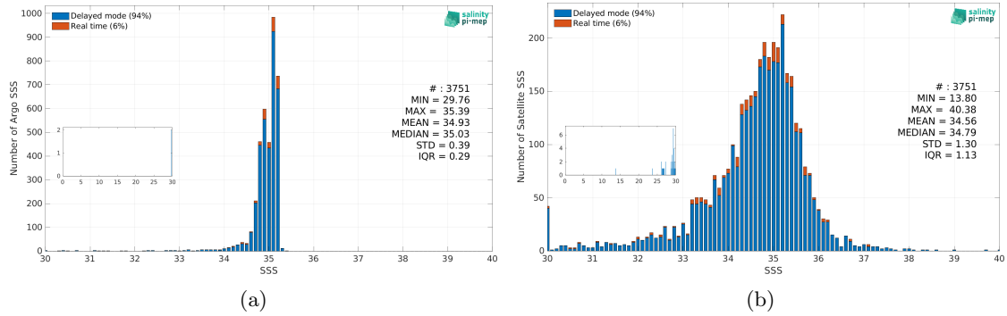
Figure 3: Histograms of SSS from Argo (a) and Aquarius SSS L2 OR v5 (NASA-GSFC) (b) considering all match-up pairs per bins of 0.1 over the Arctic Ocean Pi-MEP region and for the full satellite product period.
