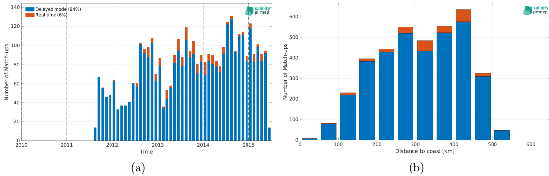
Figure 2: Number of match-ups between Argo and Aquarius SSS L2 OR v5 (NASA-GSFC) SSS as a function of time (a) and as function of the distance to coast (b) over the Arctic Ocean Pi-MEP region and for the full satellite product period.
