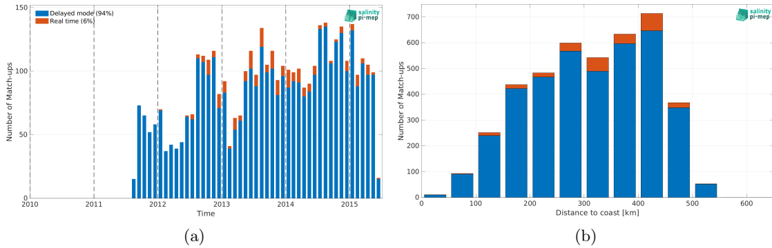
Figure 1: Number of match-ups between Argo and Aquarius SSS L2 OR v5 (NASA-GSFC) SSS as a function of time (a) and as function of the distance to coast (b) over the Arctic Ocean Pi-MEP region and for the full satellite product period.
