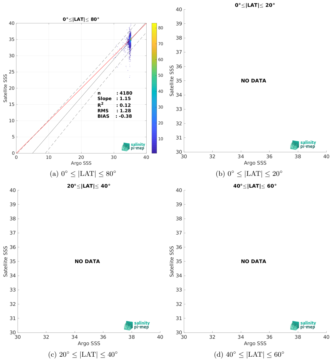
Figure 9: Contour maps of the concentration of Aquarius SSS L2 OR v5 (NASA-GSFC) SSS (y-axis) versus Argo SSS (x-axis) at match-up pairs for different latitude bands. For each plot, the red line shows x=y . The black thin and dashed lines indicate a linear fit through the data cloud and the \pm 95\% confidence levels, respectively. The number match-up pairs n , the slope and R^2 coefficient of the linear fit, the root mean square (RMS) and the mean bias between satellite and in situ data are indicated for each latitude band in each plots.
