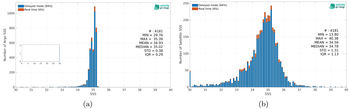
Figure 2: Histograms of SSS from Argo (a) and Aquarius SSS L2 OR v5 (NASA-GSFC) (b) considering all match-up pairs per bins of 0.1 over the Arctic Ocean Pi-MEP region and for the full satellite product period.
