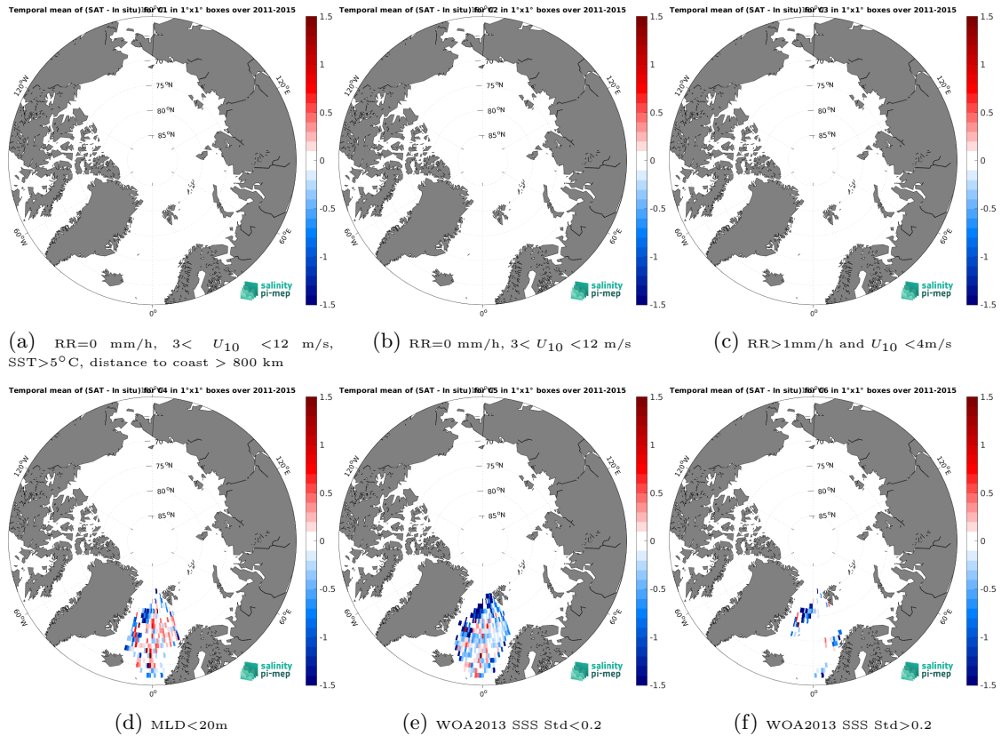
Figure 12: Temporal mean gridded over spatial boxes of size 1^{\circ}\times 1^{\circ} of \Delta\text{SSS} (Aquarius SSS L2 OR v5 (NASA-GSFC) - Argo) for 6 different subdatasets corresponding to:RR=0 mm/h, 3 < U_{10} < 12 m/s, SST > 5^{\circ}\text{C} , distance to coast > 800 km (a), RR=0 mm/h, 3 < U_{10} < 12 m/s (b), RR > 1 mm/h and U_{10} < 4 m/s (c),MLD < 20\text{m} (d),WOA2013 SSS Std < 0.2 (e),WOA2013 SSS Std > 0.2 (f).
