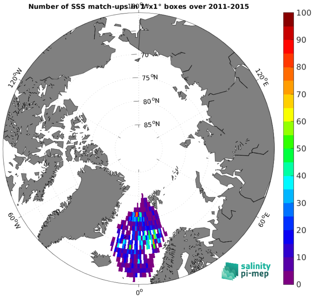
Figure 4: Number of SSS match-ups between Argo SSS and the Aquarius SSS L2 OR v5 (NASA-GSFC) SSS product for the Arctic Ocean Pi-MEP region over 1^\circ \times 1^\circ boxes and for the full satellite product period.
