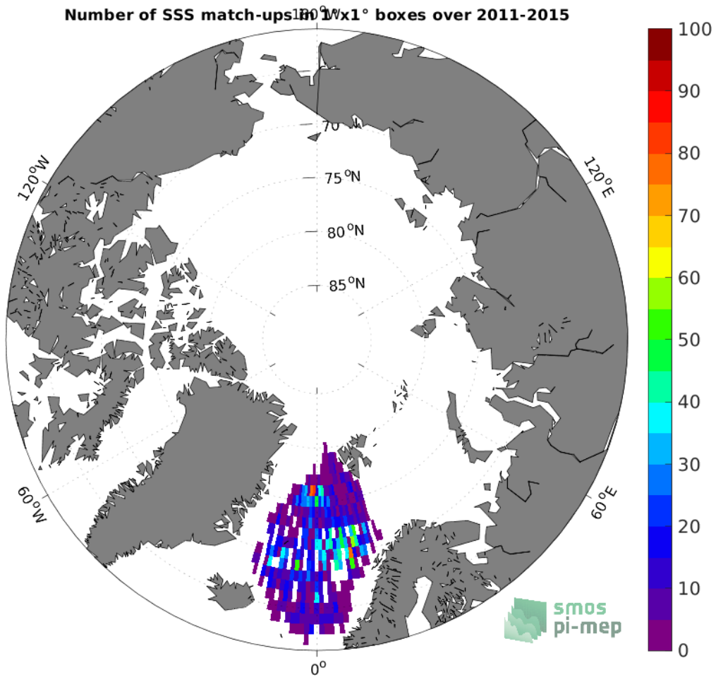
Figure 4: Number of SSS match-ups between Argo SSS and the Aquarius SSS L2 OR v5 (NASA-GSFC) SSS product for the Arctic Ocean Pi-MEP region over 1^{\circ} \times 1^{\circ} boxes and for the full satellite product period.
