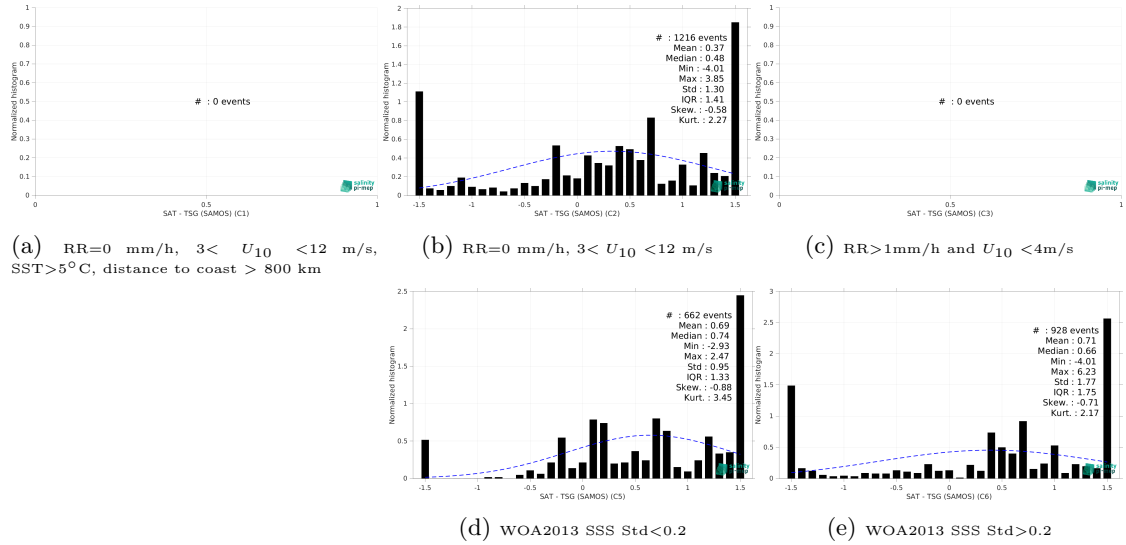
Figure 15: Normalized histogram of \Delta SSS (Aquarius SSS L2 CAP v5 (JPL) - TSG (SAMOS)) for 5 different subdatasets corresponding to: RR=0 mm/h, 3 < U_{10} < 12 m/s, SST > 5°C, distance to coast > 800 km (a), RR=0 mm/h, 3 < U_{10} < 12 m/s (b), RR > 1mm/h and U_{10} < 4 m/s (c), WOA2013 SSS Std < 0.2 (d), WOA2013 SSS Std > 0.2 (e).
