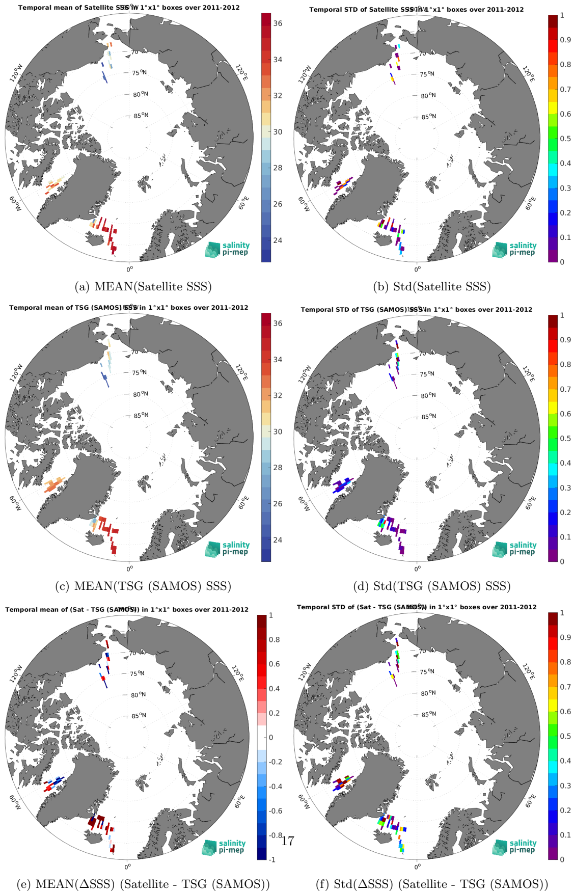
Figure 7: Temporal mean (left) and Std (right) of SSS from Aquarius SSS L2 CAP v5 (JPL) (top), TSG (SAMOS) (middle), and of \Delta SSS (Satellite - TSG (SAMOS)). Only match-up pairs are used to generate these maps.
