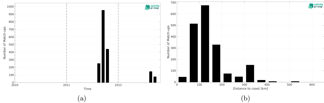
Figure 2: Number of match-ups between TSG (SAMOS) and Aquarius SSS L2 CAP v5 (JPL) SSS as a function of time (a) and as function of the distance to coast (b) over the Arctic Ocean Pi-MEP region and for the full satellite product period.
