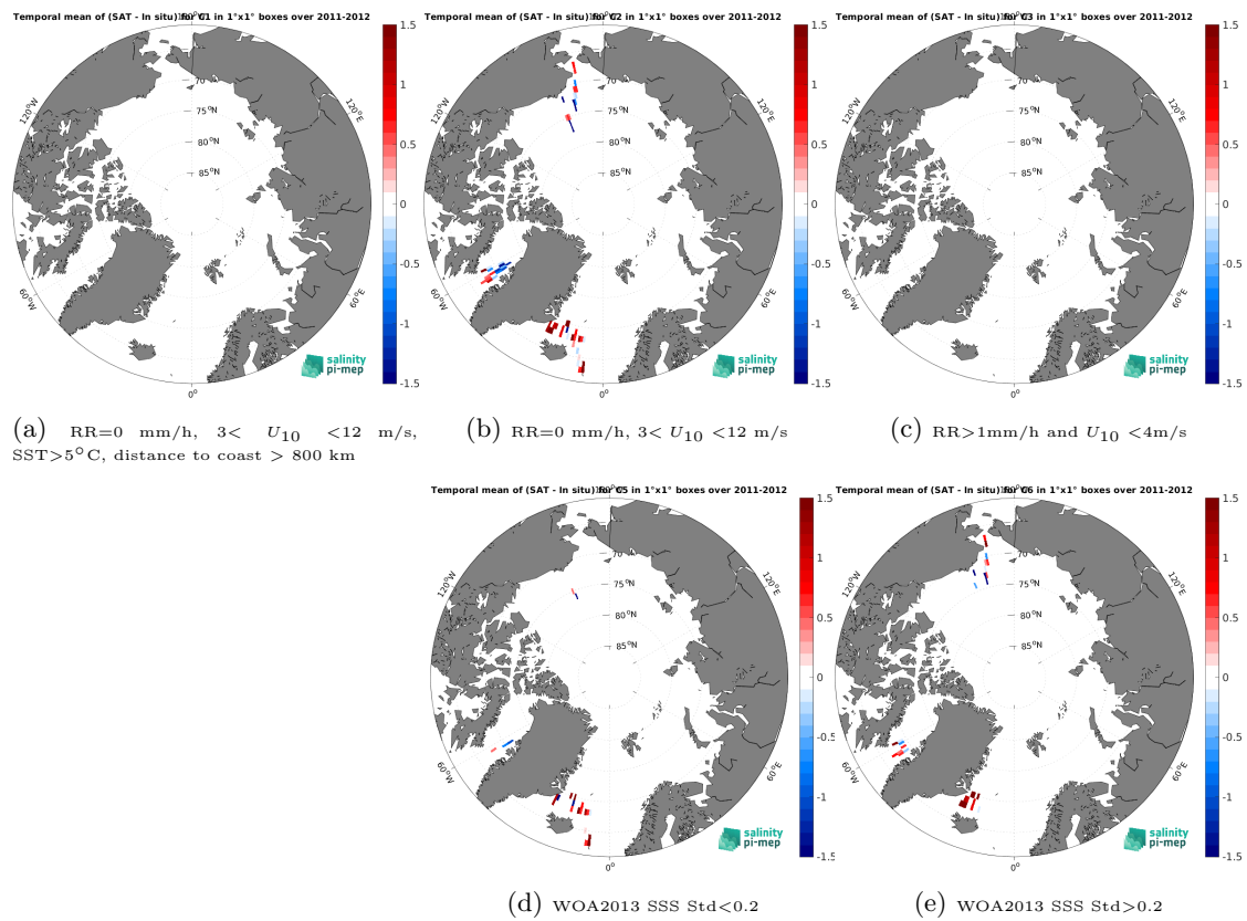
Figure 14: Temporal mean gridded over spatial boxes of size 1^\circ \times 1^\circ of \Delta SSS (Aquarius SSS L2 CAP v5 (JPL) - TSG (SAMOS)) for 5 different subdatasets corresponding to:RR=0 mm/h, 3 < U_{10} < 12 m/s, SST>5°C, distance to coast > 800 km (a), RR=0 mm/h, 3 < U_{10} < 12 m/s (b), RR>1mm/h and U_{10} < 4 m/s (c), WOA2013 SSS Std<0.2 (d), WOA2013 SSS Std>0.2 (e).
