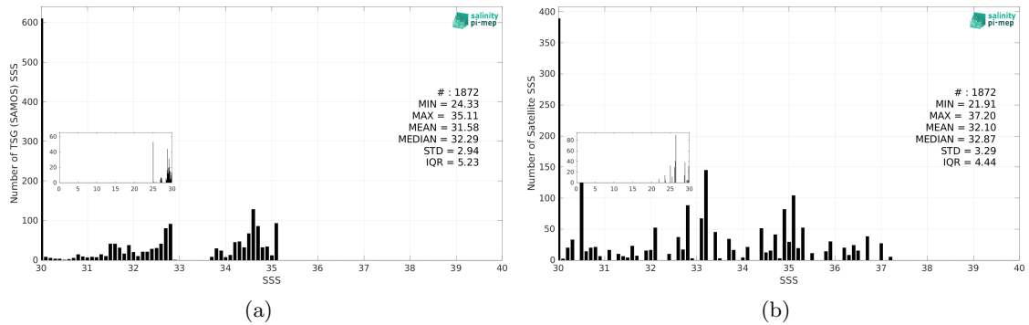
Figure 3: Histograms of SSS from TSG (SAMOS) (a) and Aquarius SSS L2 CAP v5 (JPL) (b) considering all match-up pairs per bins of 0.1 over the Arctic Ocean Pi-MEP region and for the full satellite product period.
