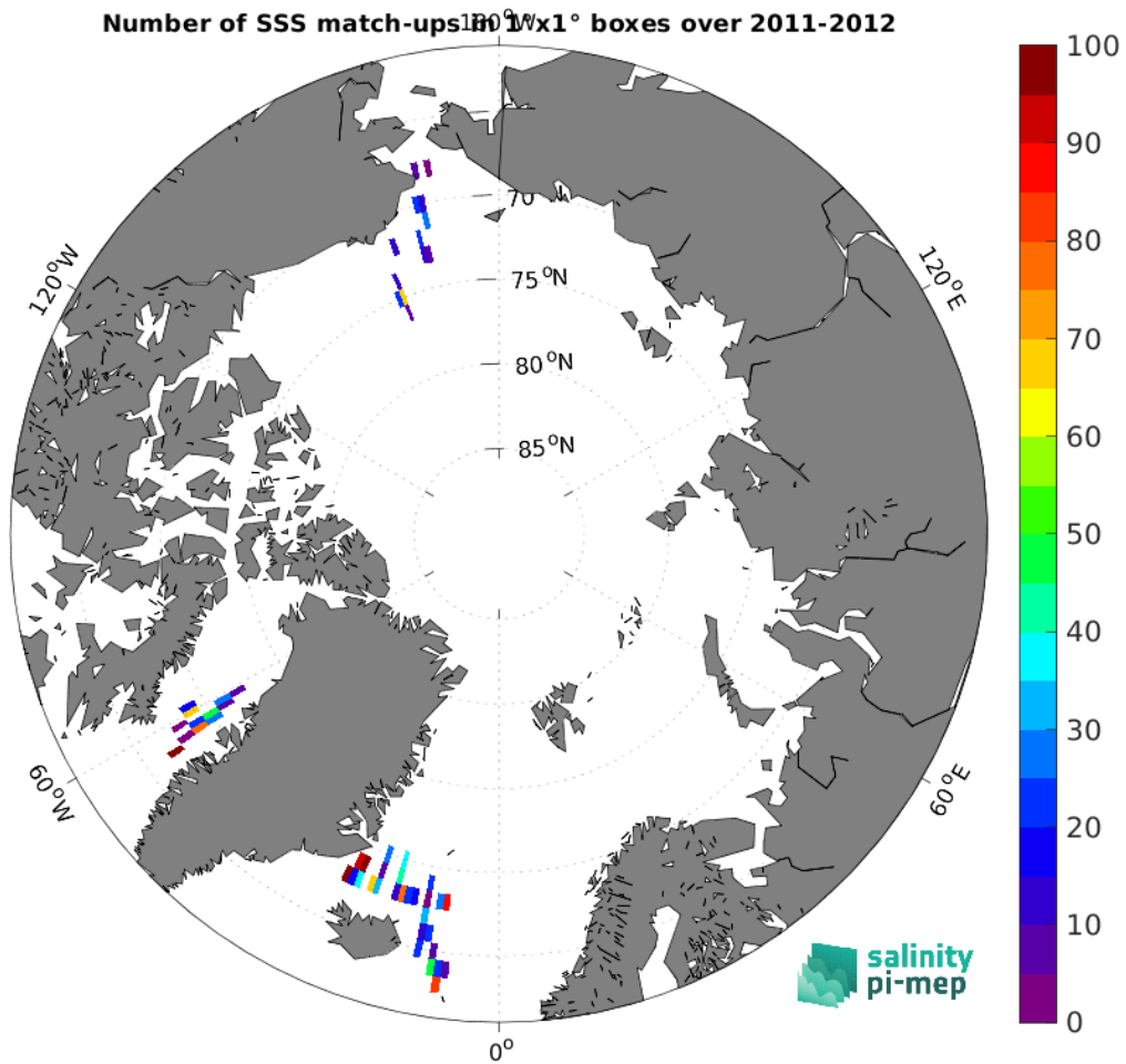
Figure 5: Number of SSS match-ups between TSG (SAMOS) SSS and the Aquarius SSS L2 CAP v5 (JPL) SSS product for the Arctic Ocean Pi-MEP region over 1^\circ \times 1^\circ boxes and for the full satellite product period.
